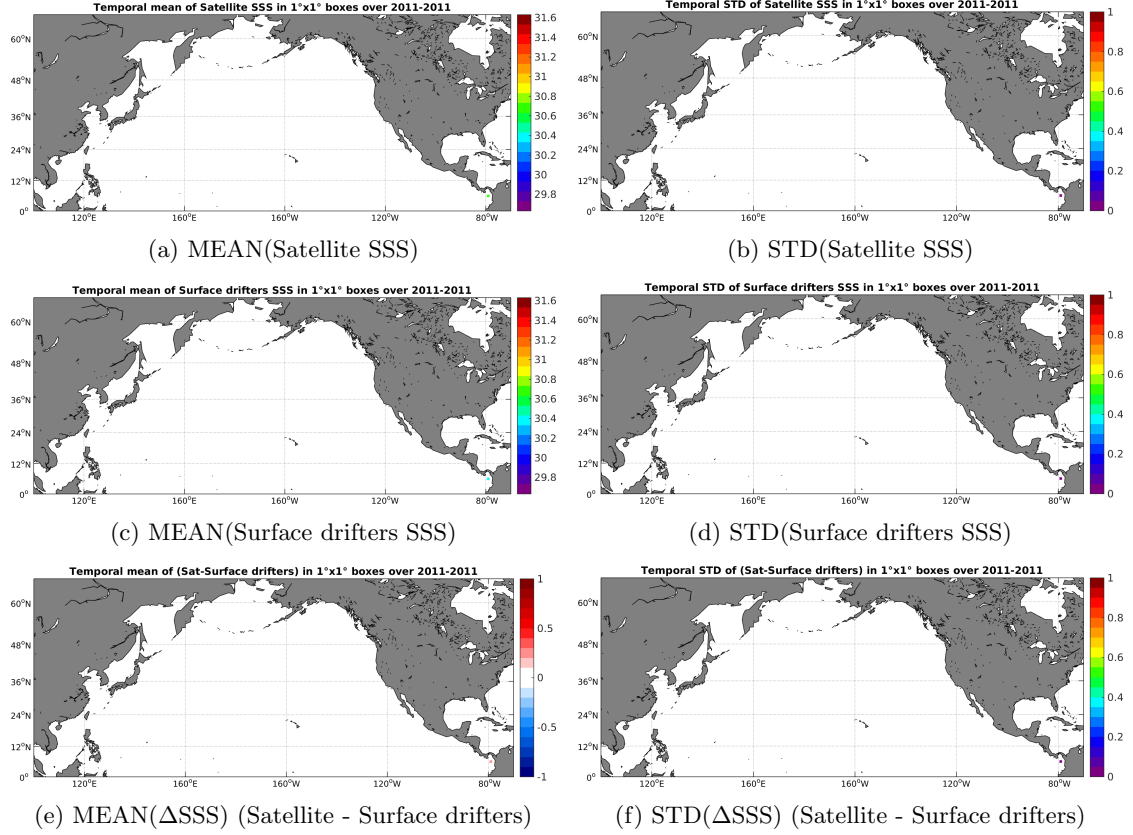
Figure 5: Temporal mean (left) and STD (right) of SSS from AQUARIUS-L2-JPL-V4 (top), Surface drifters (middle), and of \Delta SSS (Satellite - Surface drifters). Only match-up pairs are used to generate these maps.
