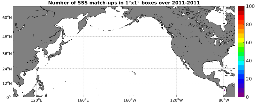
Figure 3: Number of SSS match-ups between Surface drifters SSS and the AQUARIUS-L2-JPL-V4 SSS product for the North Pacific Ocean Pi-MEP region over 1^\circ \times 1^\circ boxes and for the full satellite product period.
