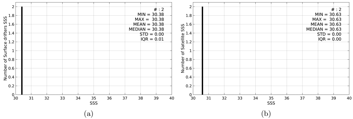
Figure 2: Histograms of SSS from Surface drifters (a) and AQUARIUS-L2-JPL-V4 (b) considering all match-up pairs per bins of 0.1 over the North Pacific Ocean Pi-MEP region and for the full satellite product period.
