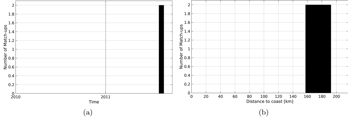
Figure 1: Number of match-ups between Surface drifters and AQUARIUS-L2-JPL-V4 SSS as a function of time (a) and as function of the distance to coast (b) over the North Pacific Ocean Pi-MEP region and for the full satellite product period.
