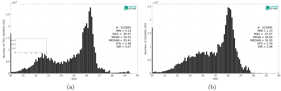
Figure 2: Histograms of SSS from TSG (SAMOS) (a) and SMOS and SMAP SSS L4 OI v1 - 7 Days (LOPS) (b) considering all match-up pairs per bins of 0.1 over the North Atlantic Ocean Pi-MEP region and for the full satellite product period.
