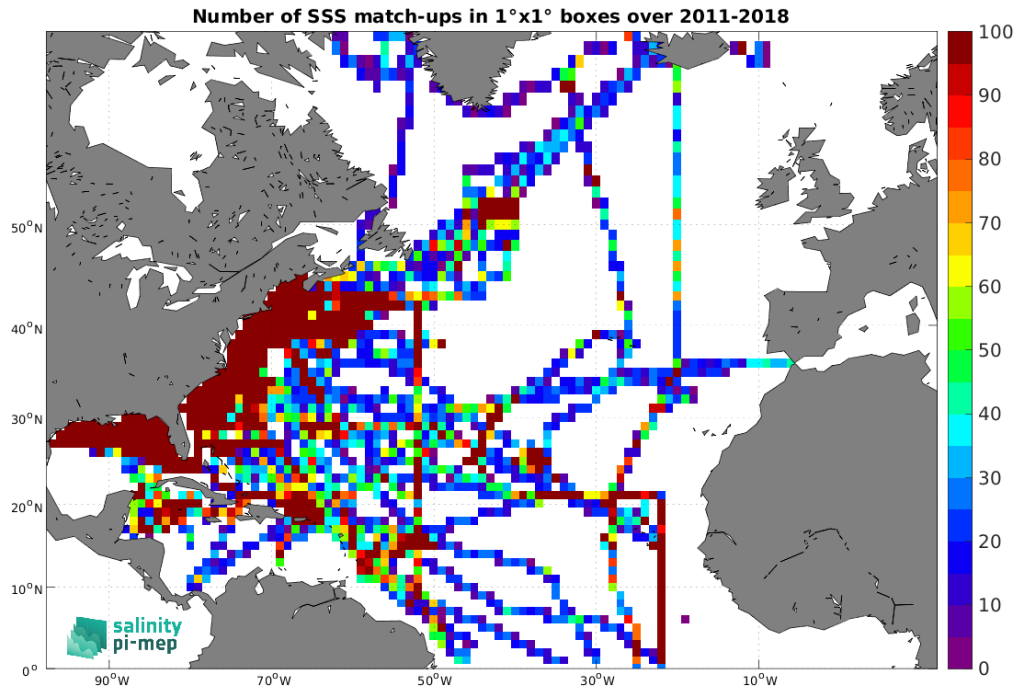
Figure 4: Number of SSS match-ups between TSG (SAMOS) SSS and the SMOS and SMAP SSS L4 OI v1 - 7 Days (LOPS) SSS product for the North Atlantic Ocean Pi-MEP region over 1^\circ \times 1^\circ boxes and for the full satellite product period.
