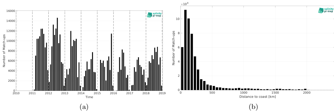
Figure 1: Number of match-ups between TSG (SAMOS) and SMOS and SMAP SSS L4 OI v1 - 7 Days (LOPS) SSS as a function of time (a) and as function of the distance to coast (b) over the North Atlantic Ocean Pi-MEP region and for the full satellite product period.
