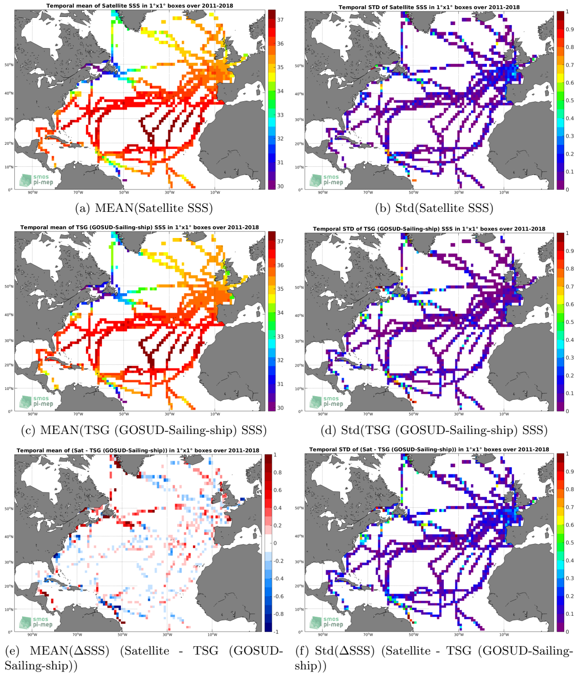
Figure 6: Temporal mean (left) and Std (right) of SSS from SMOS and SMAP SSS L4 OI v1 - 7 Days (LOPS) (top), TSG (GOSUD-Sailing-ship) (middle), and of \Delta SSS (Satellite - TSG (GOSUD-Sailing-ship)). Only match-up pairs are used to generate these maps.
