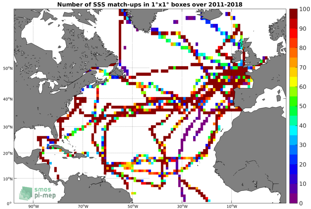
Figure 4: Number of SSS match-ups between TSG (GOSUD-Sailing-ship) SSS and the SMOS and SMAP SSS L4 OI v1 - 7 Days (LOPS) SSS product for the North Atlantic Ocean Pi-MEP region over 1^\circ \times 1^\circ boxes and for the full satellite product period.
