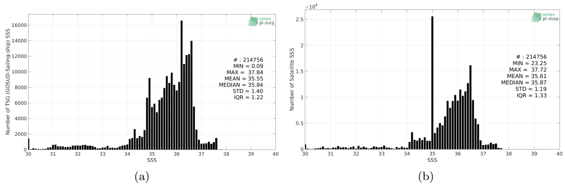
Figure 2: Histograms of SSS from TSG (GOSUD-Sailing-ship) (a) and SMOS and SMAP SSS L4 OI v1 - 7 Days (LOPS) (b) considering all match-up pairs per bins of 0.1 over the North Atlantic Ocean Pi-MEP region and for the full satellite product period.
