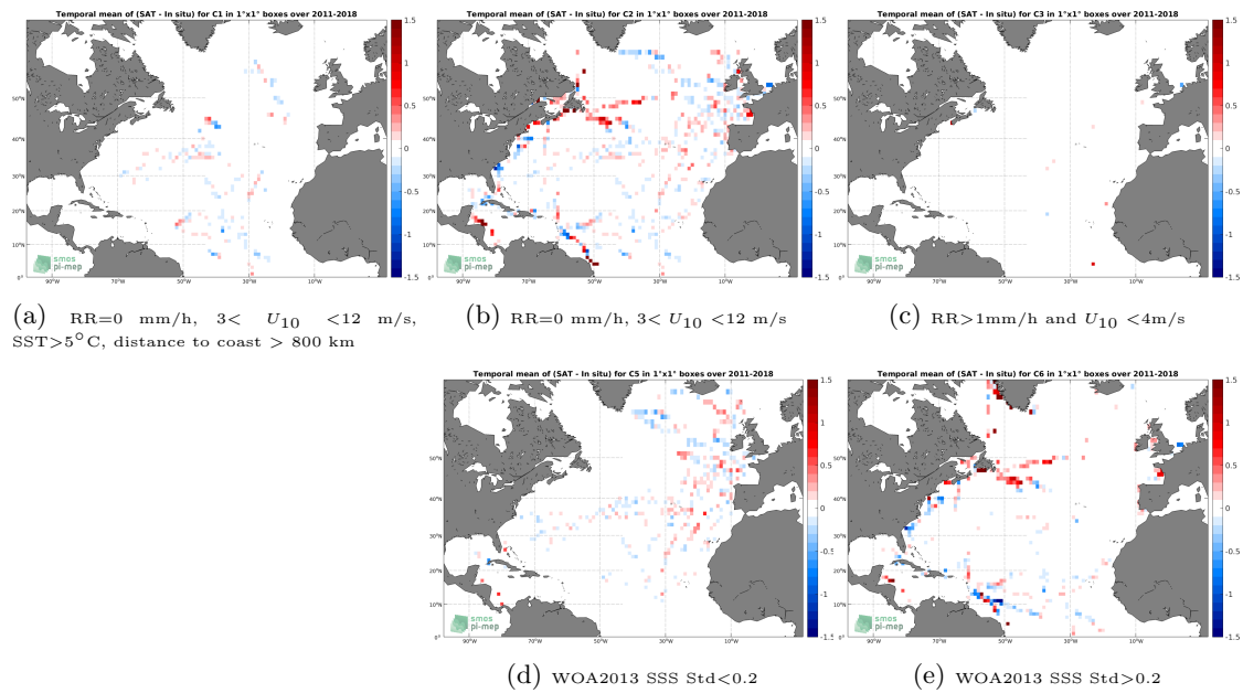
Figure 12: Temporal mean gridded over spatial boxes of size 1^\circ \times 1^\circ of \Delta\text{SSS} (SMOS and SMAP SSS L4 OI v1 - 7 Days (LOPS) - TSG (GOSUD-Sailing-ship)) for 5 different subdatasets corresponding to:RR=0 mm/h, 3 < U_{10} < 12 m/s, SST>5°C, distance to coast > 800 km (a), RR=0 mm/h, 3 < U_{10} < 12 m/s (b), RR>1mm/h and U_{10} < 4 m/s (c), WOA2013 SSS Std<0.2 (d), WOA2013 SSS Std>0.2 (e).
