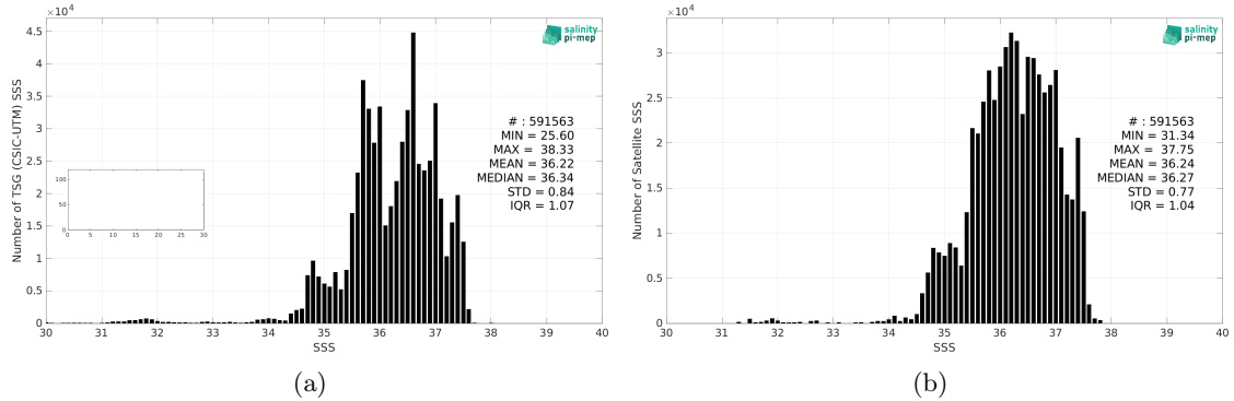
Figure 2: Histograms of SSS from TSG (CSIC-UTM) (a) and SMOS and SMAP SSS L4 OI v1 - 7 Days (LOPS) (b) considering all match-up pairs per bins of 0.1 over the North Atlantic Ocean Pi-MEP region and for the full satellite product period.
