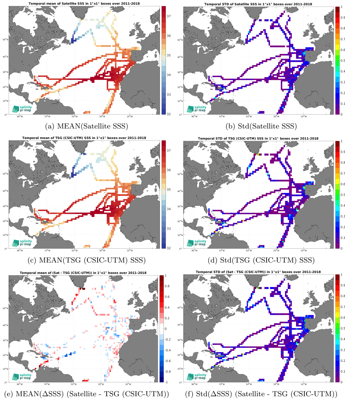
Figure 6: Temporal mean (left) and Std (right) of SSS from SMOS and SMAP SSS L4 OI v1 - 7 Days (LOPS) (top), TSG (CSIC-UTM) (middle), and of \Delta SSS (Satellite - TSG (CSIC-UTM)). Only match-up pairs are used to generate these maps.
