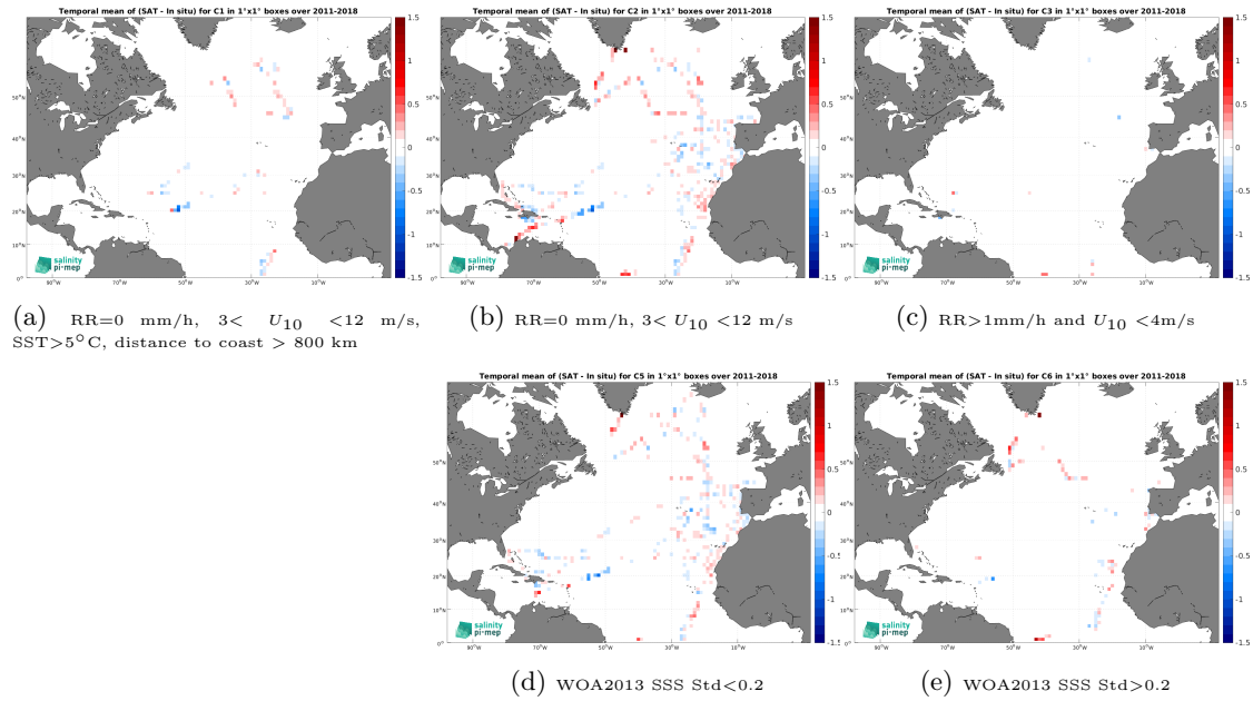
Figure 12: Temporal mean gridded over spatial boxes of size 1^\circ \times 1^\circ of \Delta\text{SSS} (SMOS and SMAP SSS L4 OI v1 - 7 Days (LOPS) - TSG (CSIC-UTM)) for 5 different subdatasets corresponding to:RR=0 mm/h, 3 < U_{10} < 12 m/s, SST >5^\circ\text{C} , distance to coast > 800 km (a), RR=0 mm/h, 3 < U_{10} < 12 m/s (b), RR >1 mm/h and U_{10} < 4 m/s (c), WOA2013 SSS Std <0.2 (d), WOA2013 SSS Std >0.2 (e).
