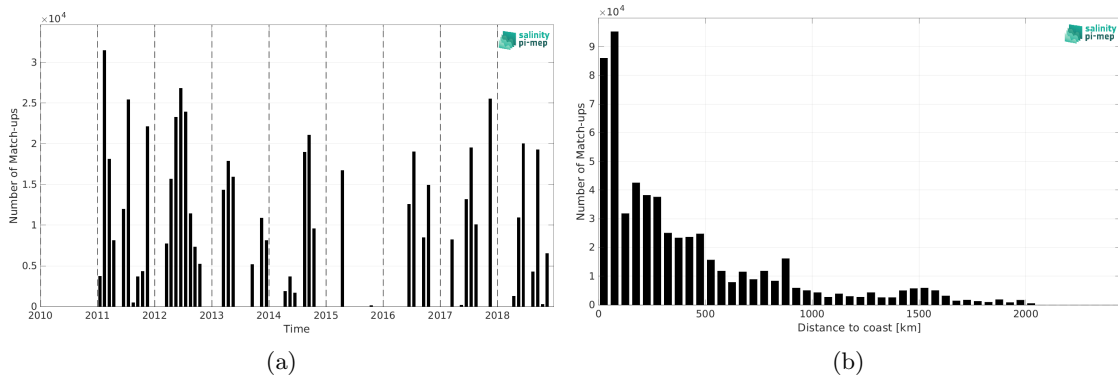
Figure 1: Number of match-ups between TSG (CSIC-UTM) and SMOS and SMAP SSS L4 OI v1 - 7 Days (LOPS) SSS as a function of time (a) and as function of the distance to coast (b) over the North Atlantic Ocean Pi-MEP region and for the full satellite product period.
