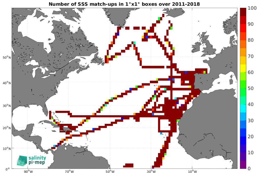
Figure 4: Number of SSS match-ups between TSG (CSIC-UTM) SSS and the SMOS and SMAP SSS L4 OI v1 - 7 Days (LOPS) SSS product for the North Atlantic Ocean Pi-MEP region over 1^\circ \times 1^\circ boxes and for the full satellite product period.
