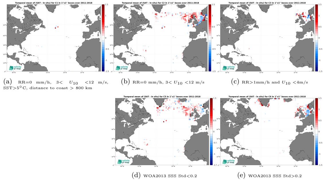
Figure 12: Temporal mean gridded over spatial boxes of size 1^\circ \times 1^\circ of \Delta\text{SSS} (SMOS and SMAP SSS L4 OI v1 - 7 Days (LOPS) - ICES) for 5 different subdatasets corresponding to:RR=0 mm/h, 3 < U_{10} < 12 m/s, SST >5^\circ\text{C} , distance to coast > 800 km (a), RR=0 mm/h, 3 < U_{10} < 12 m/s (b), RR >1 mm/h and U_{10} < 4 m/s (c), WOA2013 SSS Std <0.2 (d), WOA2013 SSS Std >0.2 (e).
