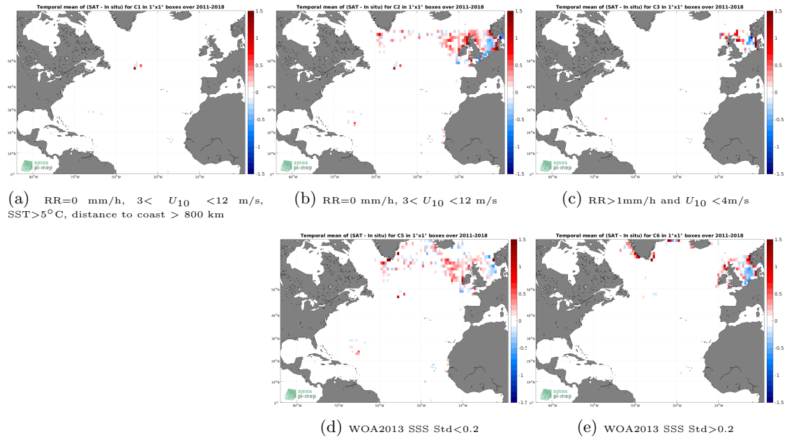
Figure 12: Temporal mean gridded over spatial boxes of size 1^\circ \times 1^\circ of \Delta SSS (SMOS and SMAP SSS L4 OI v1 - 7 Days (LOPS) - ICES) for 5 different subdatasets corresponding to:RR=0 mm/h, 3 < U_{10} < 12 m/s, SST >5^\circ\text{C} , distance to coast > 800 km (a), RR=0 mm/h, 3 < U_{10} < 12 m/s (b), RR >1 mm/h and U_{10} < 4 m/s (c), WOA2013 SSS Std <0.2 (d), WOA2013 SSS Std >0.2 (e).
