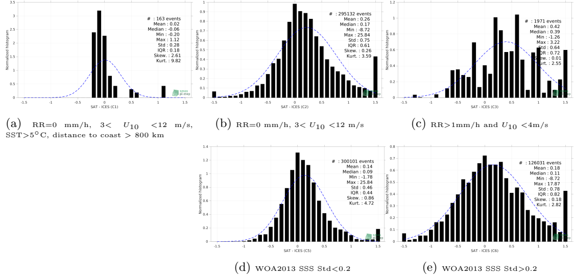
Figure 13: Normalized histogram of \Delta SSS (SMOS and SMAP SSS L4 OI v1 - 7 Days (LOPS) - ICES) for 5 different subdatasets corresponding to: RR=0 mm/h, 3 < U_{10} < 12 m/s, SST > 5°C, distance to coast > 800 km (a), RR=0 mm/h, 3 < U_{10} < 12 m/s (b), RR > 1mm/h and U_{10} < 4 m/s (c), WOA2013 SSS Std < 0.2 (d), WOA2013 SSS Std > 0.2 (e).
