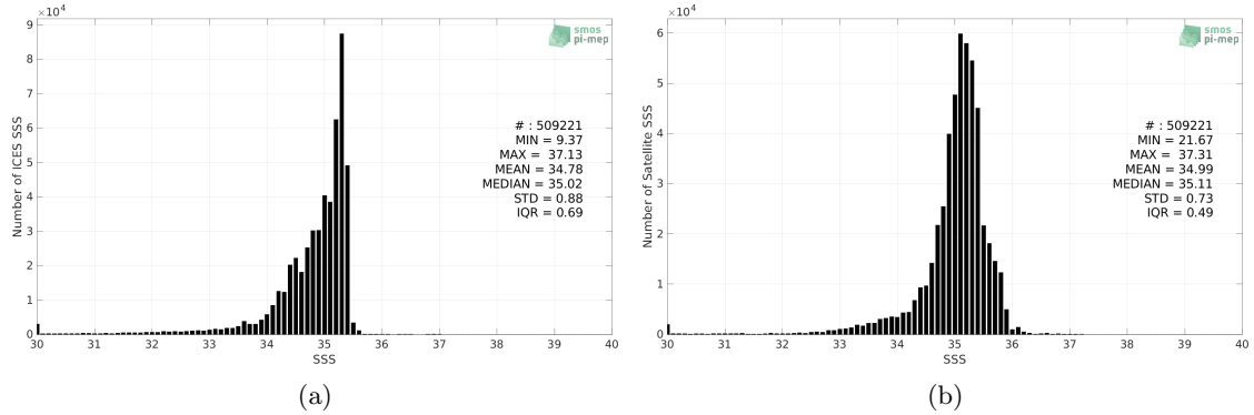
Figure 2: Histograms of SSS from ICES (a) and SMOS and SMAP SSS L4 OI v1 - 7 Days (LOPS) (b) considering all match-up pairs per bins of 0.1 over the North Atlantic Ocean Pi-MEP region and for the full satellite product period.
