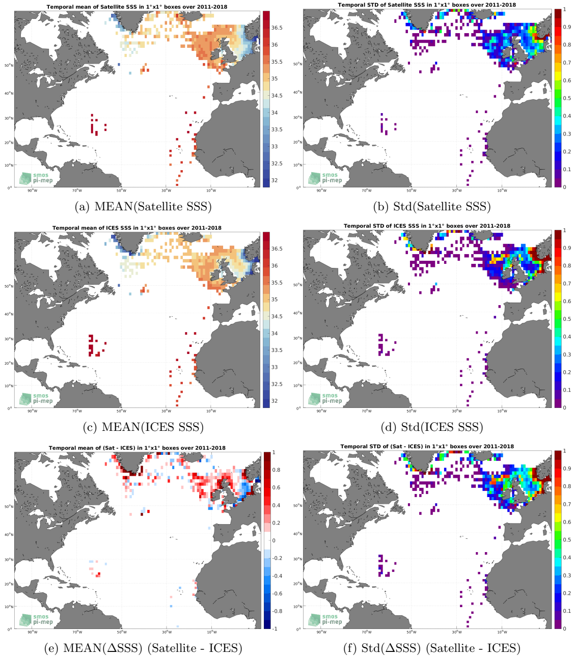
Figure 6: Temporal mean (left) and Std (right) of SSS from SMOS and SMAP SSS L4 OI v1 - 7 Days (LOPS) (top), ICES (middle), and of \Delta SSS (Satellite - ICES). Only match-up pairs are used to generate these maps.
