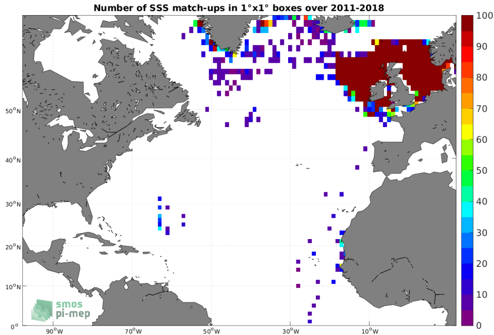
Figure 4: Number of SSS match-ups between ICES SSS and the SMOS and SMAP SSS L4 OI v1 - 7 Days (LOPS) SSS product for the North Atlantic Ocean Pi-MEP region over 1^\circ \times 1^\circ boxes and for the full satellite product period.
