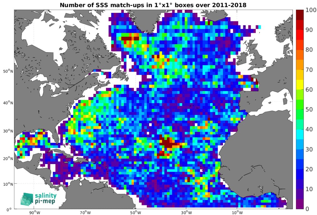
Figure 4: Number of SSS match-ups between Argo SSS and the SMOS and SMAP SSS L4 OI v1 - 7 Days (LOPS) SSS product for the North Atlantic Ocean Pi-MEP region over 1^\circ \times 1^\circ boxes and for the full satellite product period.
