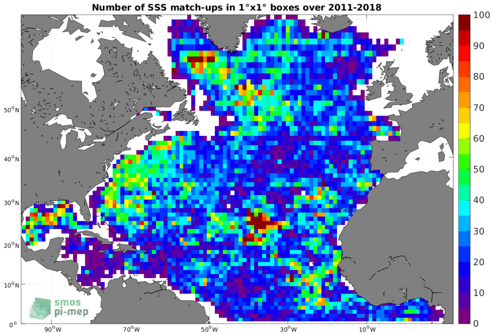
Figure 4: Number of SSS match-ups between Argo SSS and the SMOS and SMAP SSS L4 OI v1 - 7 Days (LOPS) SSS product for the North Atlantic Ocean Pi-MEP region over 1^{\circ} \times 1^{\circ} boxes and for the full satellite product period.
