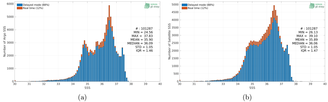
Figure 2: Histograms of SSS from Argo (a) and SMOS and SMAP SSS L4 OI v1 - 7 Days (LOPS) (b) considering all match-up pairs per bins of 0.1 over the North Atlantic Ocean Pi-MEP region and for the full satellite product period.
