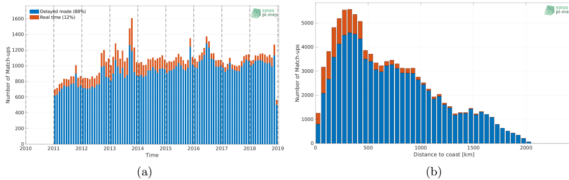
Figure 1: Number of match-ups between Argo and SMOS and SMAP SSS L4 OI v1 - 7 Days (LOPS) SSS as a function of time (a) and as function of the distance to coast (b) over the North Atlantic Ocean Pi-MEP region and for the full satellite product period.
