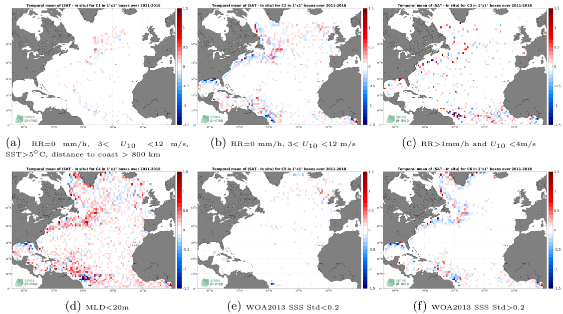
Figure 12: Temporal mean gridded over spatial boxes of size 1^\circ \times 1^\circ of \Delta SSS (SMOS and SMAP SSS L4 OI v1 - 7 Days (LOPS) - Argo) for 6 different subdatasets corresponding to:RR=0 mm/h, 3 < U_{10} < 12 m/s, SST > 5^\circ\text{C} , distance to coast > 800 km (a), RR=0 mm/h, 3 < U_{10} < 12 m/s (b), RR > 1 mm/h and U_{10} < 4 m/s (c),MLD < 20 m (d),WOA2013 SSS Std < 0.2 (e),WOA2013 SSS Std > 0.2 (f).
