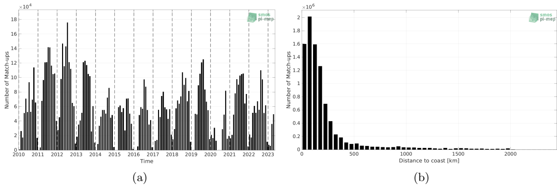
Figure 1: Number of match-ups between TSG (SAMOS) and SMOS SSS L4 v1 - Weekly (CMEMS-CNR) SSS as a function of time (a) and as function of the distance to coast (b) over the North Atlantic Ocean Pi-MEP region and for the full satellite product period.
