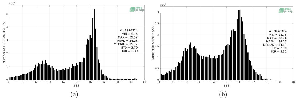
Figure 2: Histograms of SSS from TSG (SAMOS) (a) and SMOS SSS L4 v1 - Weekly (CMEMS-CNR) (b) considering all match-up pairs per bins of 0.1 over the North Atlantic Ocean Pi-MEP region and for the full satellite product period.
