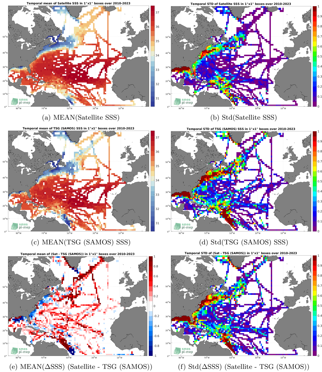
Figure 6: Temporal mean (left) and Std (right) of SSS from SMOS SSS L4 v1 - Weekly (CMEMS-CNR) (top), TSG (SAMOS) (middle), and of \Delta SSS (Satellite - TSG (SAMOS)). Only match-up pairs are used to generate these maps.
