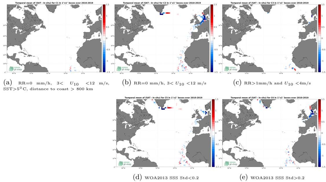
Figure 12: Temporal mean gridded over spatial boxes of size 1^\circ \times 1^\circ of \Delta\text{SSS} (SMOS SSS L4 v1 - Weekly (CMEMS-CNR) - TSG (Polarstern)) for 5 different subdatasets corresponding to:RR=0 mm/h, 3 < U_{10} < 12 m/s, SST >5^\circ\text{C} , distance to coast > 800 km (a), RR=0 mm/h, 3 < U_{10} < 12 m/s (b), RR >1 mm/h and U_{10} < 4 m/s (c), WOA2013 SSS Std <0.2 (d), WOA2013 SSS Std >0.2 (e).
