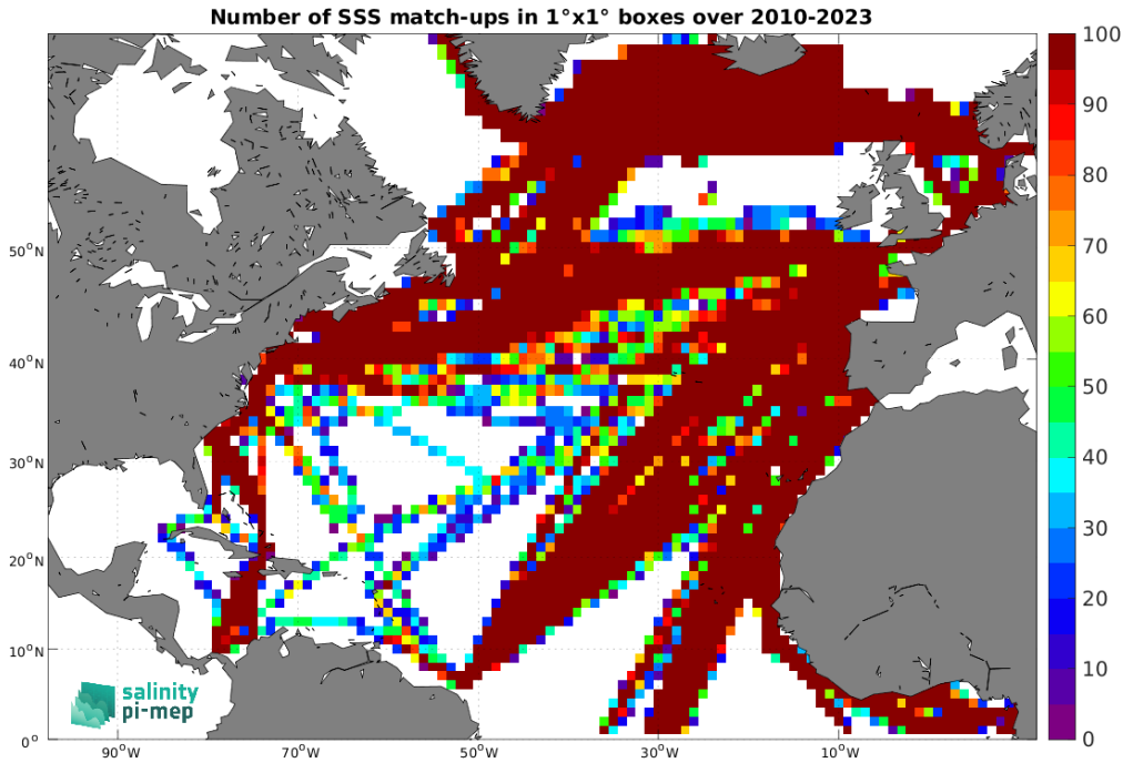
Figure 4: Number of SSS match-ups between TSG (LEGOS-DM) SSS and the SMOS SSS L4 v1 - Weekly (CMEMS-CNR) SSS product for the North Atlantic Ocean Pi-MEP region over 1°x1° boxes and for the full satellite product period.
