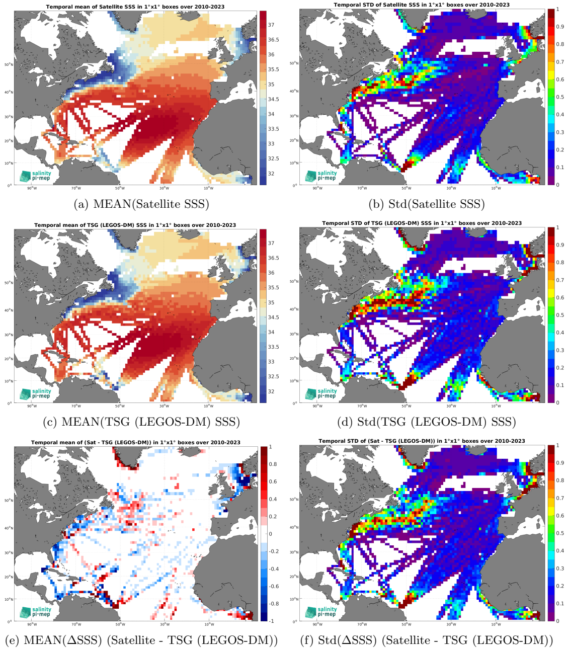
Figure 6: Temporal mean (left) and Std (right) of SSS from SMOS SSS L4 v1 - Weekly (CMEMS-CNR) (top), TSG (LEGOS-DM) (middle), and of \Delta SSS (Satellite - TSG (LEGOS-DM)). Only match-up pairs are used to generate these maps.
