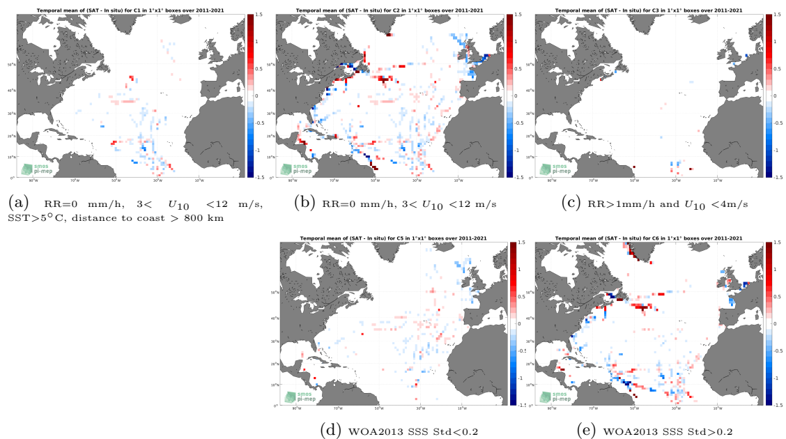
Figure 12: Temporal mean gridded over spatial boxes of size 1^\circ \times 1^\circ of \Delta\text{SSS} (SMOS SSS L4 v1 - Weekly (CMEMS-CNR) - TSG (GOSUD-Sailing-ship)) for 5 different subdatasets corresponding to:RR=0 mm/h, 3 < U_{10} < 12 m/s, SST >5^\circ\text{C} , distance to coast > 800 km (a), RR=0 mm/h, 3 < U_{10} < 12 m/s (b), RR >1 mm/h and U_{10} < 4 m/s (c), WOA2013 SSS Std <0.2 (d), WOA2013 SSS Std >0.2 (e).
