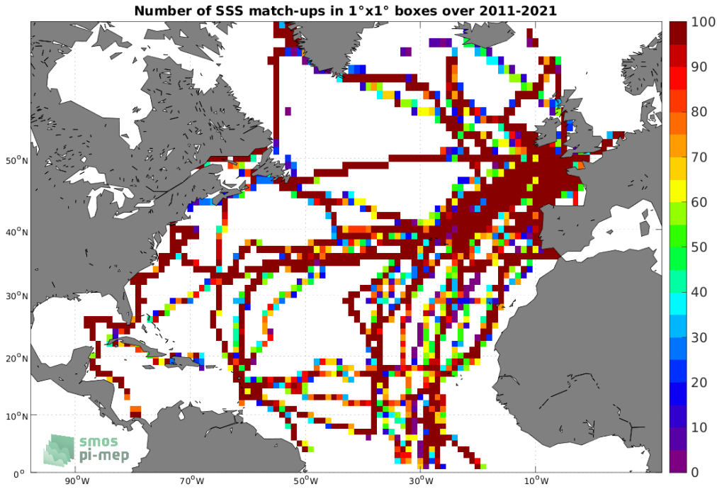
Figure 4: Number of SSS match-ups between TSG (GOSUD-Sailing-ship) SSS and the SMOS SSS L4 v1 - Weekly (CMEMS-CNR) SSS product for the North Atlantic Ocean Pi-MEP region over 1^\circ \times 1^\circ boxes and for the full satellite product period.
