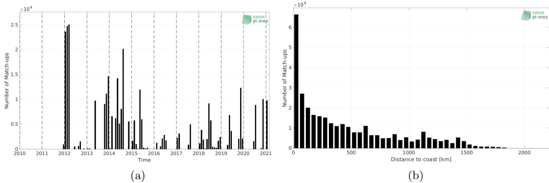
Figure 1: Number of match-ups between TSG (GOSUD-Sailing-ship) and SMOS SSS L4 v1 - Weekly (CMEMS-CNR) SSS as a function of time (a) and as function of the distance to coast (b) over the North Atlantic Ocean Pi-MEP region and for the full satellite product period.
