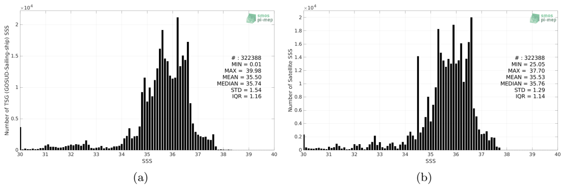
Figure 2: Histograms of SSS from TSG (GOSUD-Sailing-ship) (a) and SMOS SSS L4 v1 - Weekly (CMEMS-CNR) (b) considering all match-up pairs per bins of 0.1 over the North Atlantic Ocean Pi-MEP region and for the full satellite product period.
