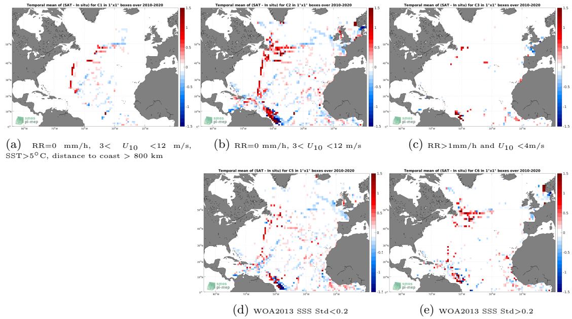
Figure 12: Temporal mean gridded over spatial boxes of size 1^\circ \times 1^\circ of \Delta\text{SSS} (SMOS SSS L4 v1 - Weekly (CMEMS-CNR) - TSG (GOSUD-Research-vessel)) for 5 different subdatasets corresponding to:RR=0 mm/h, 3 < U_{10} < 12 m/s, SST >5^\circ\text{C} , distance to coast > 800 km (a), RR=0 mm/h, 3 < U_{10} < 12 m/s (b), RR >1 mm/h and U_{10} < 4 m/s (c), WOA2013 SSS Std <0.2 (d), WOA2013 SSS Std >0.2 (e).
