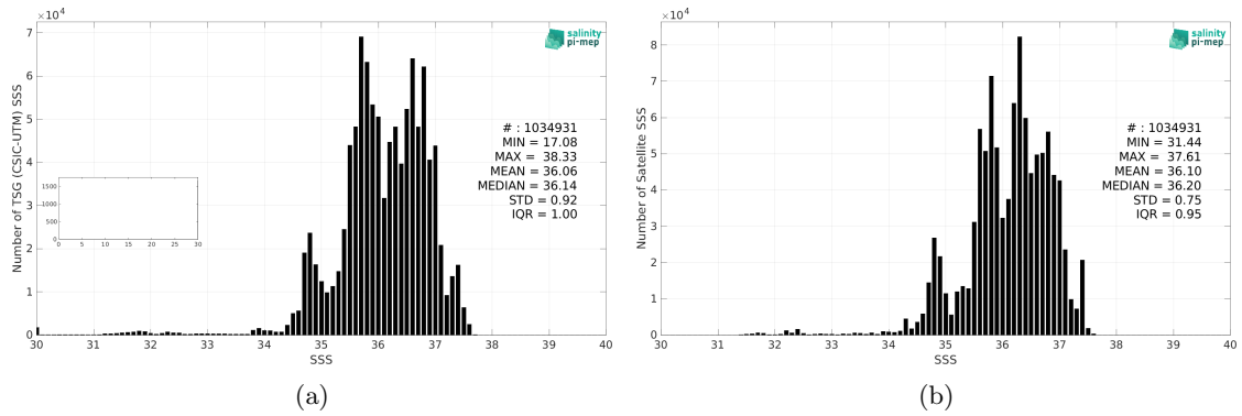
Figure 2: Histograms of SSS from TSG (CSIC-UTM) (a) and SMOS SSS L4 v1 - Weekly (CMEMS-CNR) (b) considering all match-up pairs per bins of 0.1 over the North Atlantic Ocean Pi-MEP region and for the full satellite product period.
