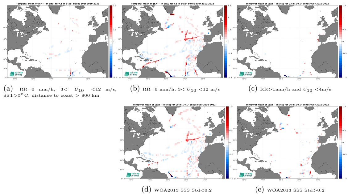
Figure 12: Temporal mean gridded over spatial boxes of size 1^\circ \times 1^\circ of \Delta SSS (SMOS SSS L4 v1 - Weekly (CMEMS-CNR) - TSG (CSIC-UTM)) for 5 different subdatasets corresponding to:RR=0 mm/h, 3 < U_{10} < 12 m/s, SST > 5^\circ\text{C} , distance to coast > 800 km (a), RR=0 mm/h, 3 < U_{10} < 12 m/s (b), RR > 1 mm/h and U_{10} < 4 m/s (c), WOA2013 SSS Std < 0.2 (d), WOA2013 SSS Std > 0.2 (e).
