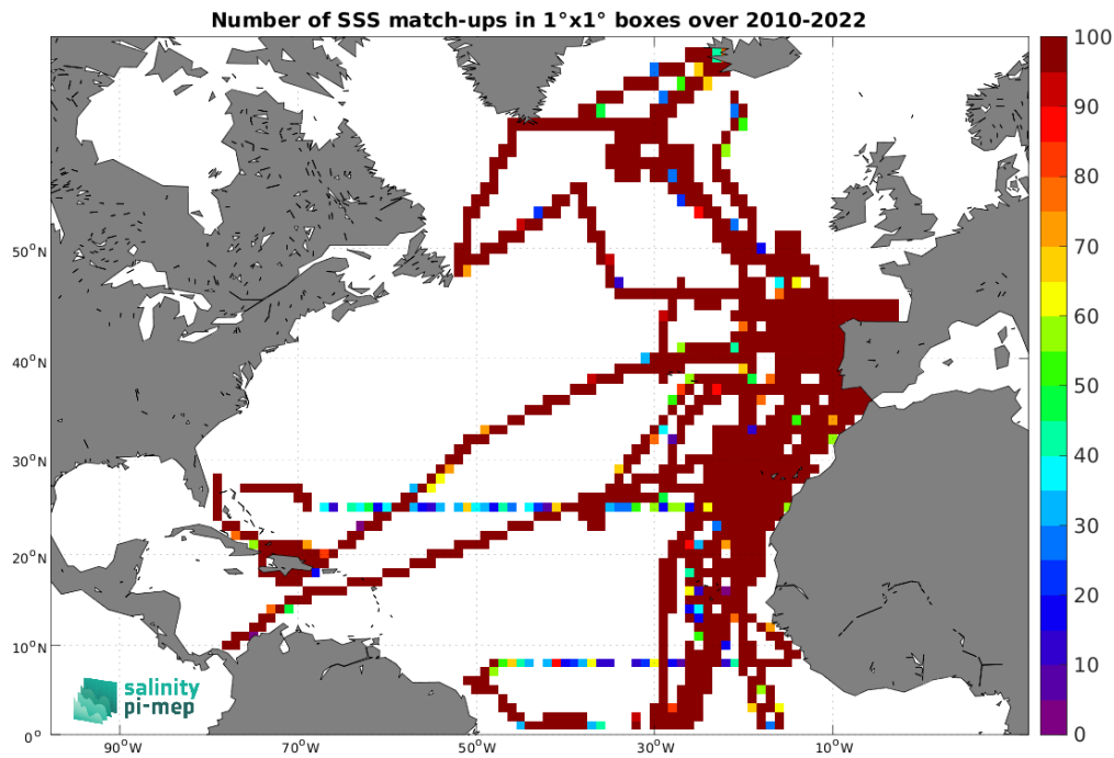
Figure 4: Number of SSS match-ups between TSG (CSIC-UTM) SSS and the SMOS SSS L4 v1 - Weekly (CMEMS-CNR) SSS product for the North Atlantic Ocean Pi-MEP region over 1^\circ \times 1^\circ boxes and for the full satellite product period.
