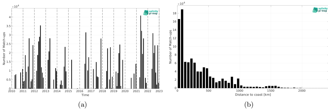
Figure 1: Number of match-ups between TSG (CSIC-UTM) and SMOS SSS L4 v1 - Weekly (CMEMS-CNR) SSS as a function of time (a) and as function of the distance to coast (b) over the North Atlantic Ocean Pi-MEP region and for the full satellite product period.
