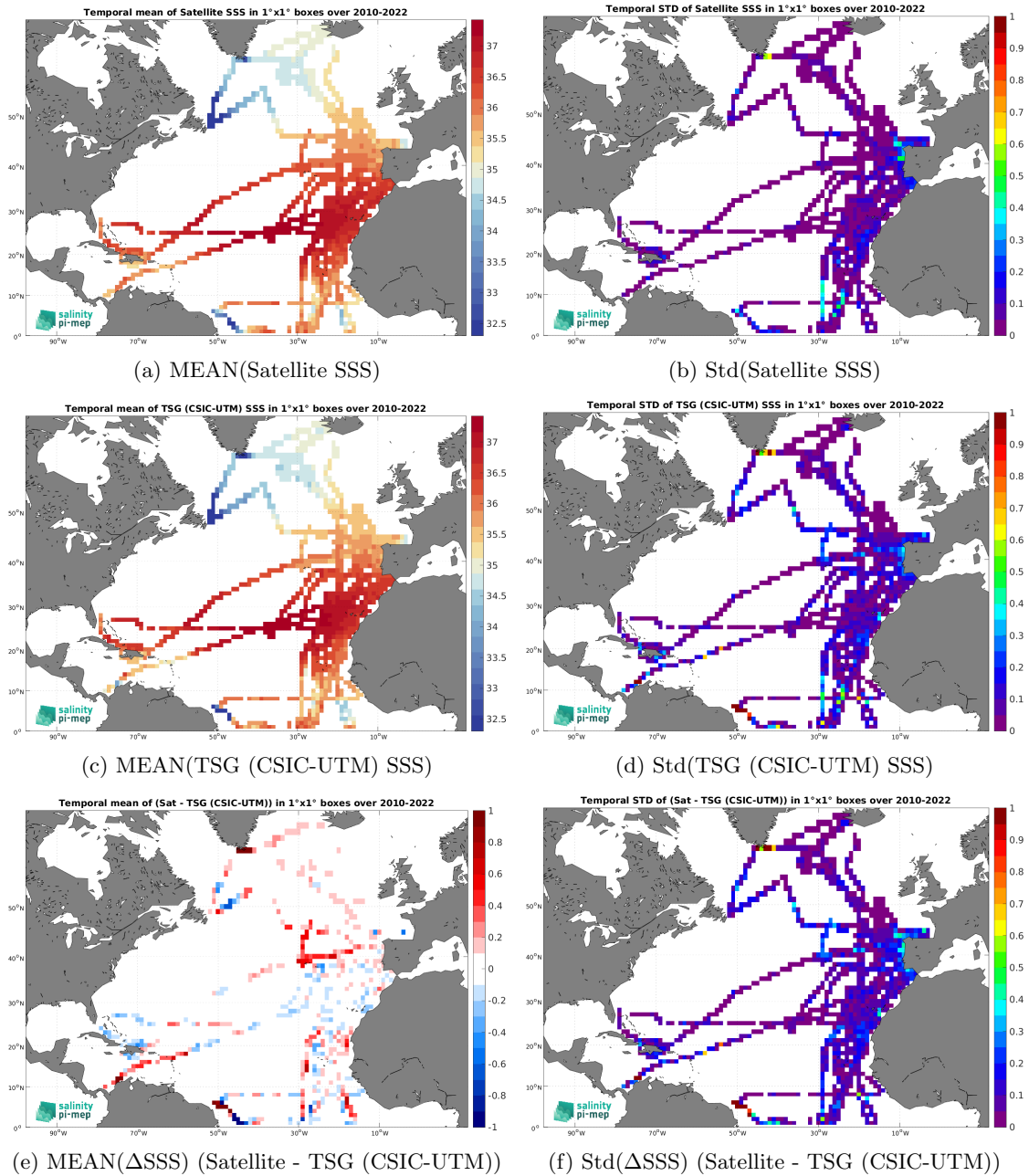
Figure 6: Temporal mean (left) and Std (right) of SSS from SMOS SSS L4 v1 - Weekly (CMEMS-CNR) (top), TSG (CSIC-UTM) (middle), and of \Delta SSS (Satellite - TSG (CSIC-UTM)). Only match-up pairs are used to generate these maps.
