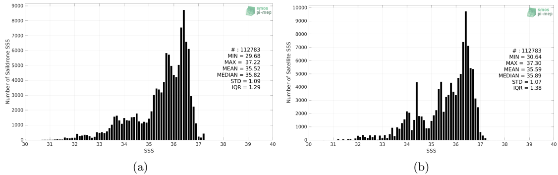
Figure 2: Histograms of SSS from Sairdrone (a) and SMOS SSS L4 v1 - Weekly (CMEMS-CNR) (b) considering all match-up pairs per bins of 0.1 over the North Atlantic Ocean Pi-MEP region and for the full satellite product period.
