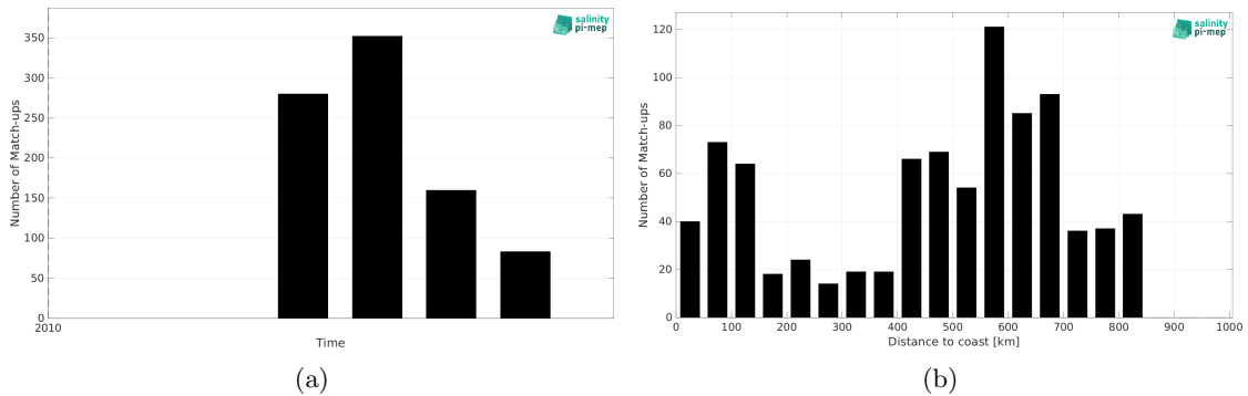
Figure 1: Number of match-ups between Marine mammals and SMOS SSS L4 v1 - Weekly (CMEMS-CNR) SSS as a function of time (a) and as function of the distance to coast (b) over the North Atlantic Ocean Pi-MEP region and for the full satellite product period.
