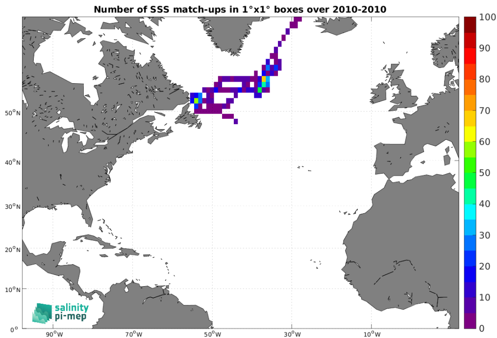
Figure 4: Number of SSS match-ups between Marine mammals SSS and the SMOS SSS L4 v1 - Weekly (CMEMS-CNR) SSS product for the North Atlantic Ocean Pi-MEP region over 1^\circ \times 1^\circ boxes and for the full satellite product period.
