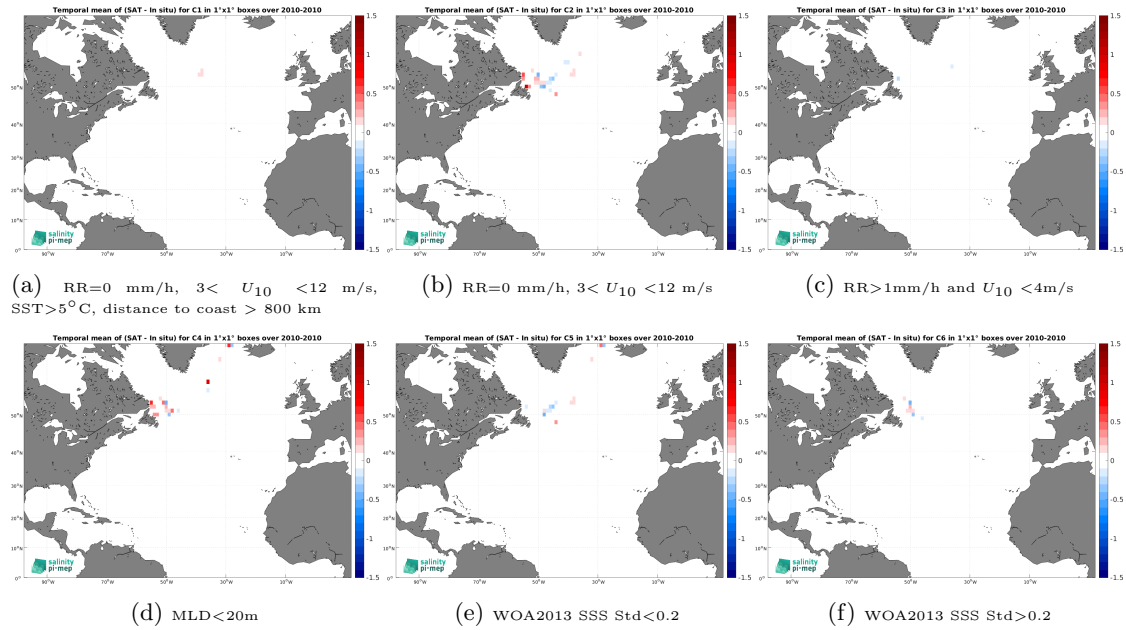
Figure 12: Temporal mean gridded over spatial boxes of size 1^{\circ}\times 1^{\circ} of \Delta\text{SSS} (SMOS SSS L4 v1 - Weekly (CMEMS-CNR) - Marine mammals) for 6 different subdatasets corresponding to:RR=0 mm/h, 3 < U_{10} < 12 m/s, SST > 5^{\circ}\text{C} , distance to coast > 800 km (a), RR=0 mm/h, 3 < U_{10} < 12 m/s (b), RR > 1 mm/h and U_{10} < 4 m/s (c),MLD < 20\text{m} (d),WOA2013 SSS Std < 0.2 (e),WOA2013 SSS Std > 0.2 (f).
