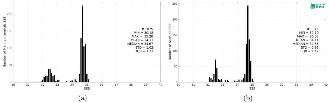
Figure 2: Histograms of SSS from Marine mammals (a) and SMOS SSS L4 v1 - Weekly (CMEMS-CNR) (b) considering all match-up pairs per bins of 0.1 over the North Atlantic Ocean Pi-MEP region and for the full satellite product period.
