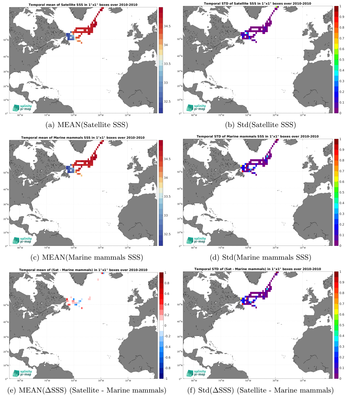
Figure 6: Temporal mean (left) and Std (right) of SSS from SMOS SSS L4 v1 - Weekly (CMEMS-CNR) (top), Marine mammals (middle), and of \Delta SSS (Satellite - Marine mammals). Only match-up pairs are used to generate these maps.
