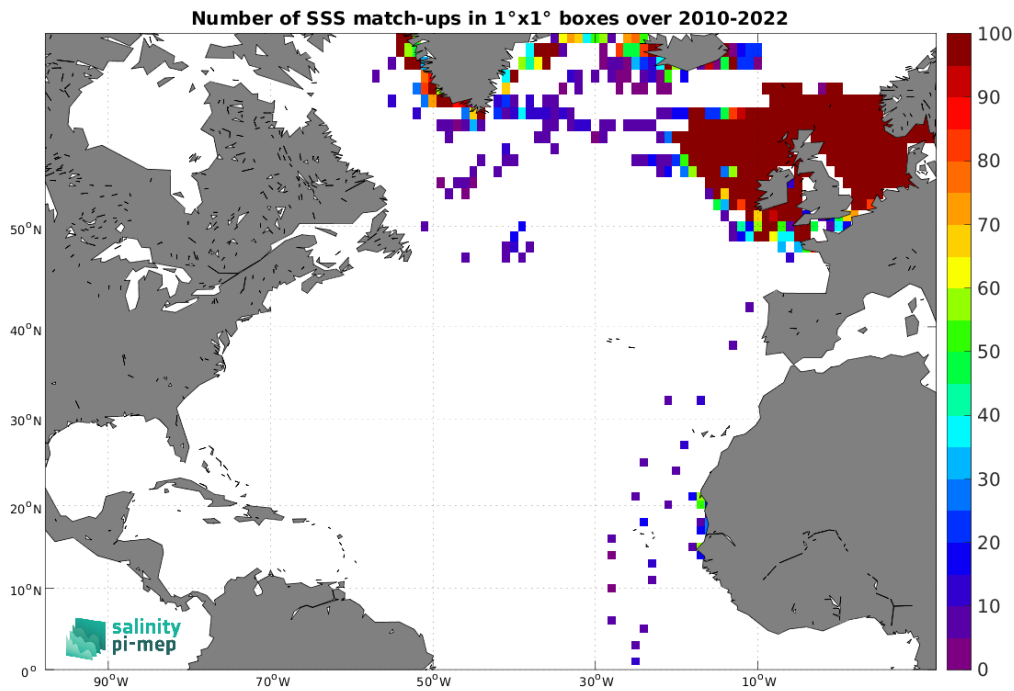
Figure 4: Number of SSS match-ups between ICES SSS and the SMOS SSS L4 v1 - Weekly (CMEMS-CNR) SSS product for the North Atlantic Ocean Pi-MEP region over 1^{\circ} \times 1^{\circ} boxes and for the full satellite product period.
