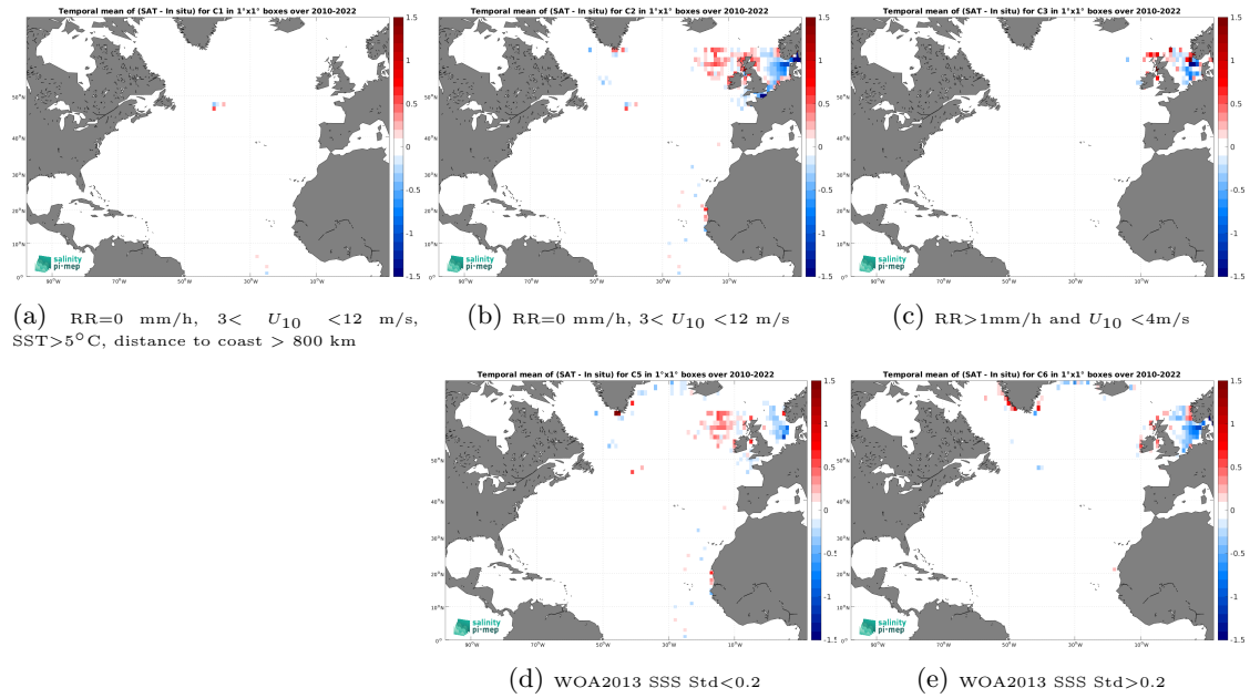
Figure 12: Temporal mean gridded over spatial boxes of size 1^\circ \times 1^\circ of \Delta\text{SSS} (SMOS SSS L4 v1 - Weekly (CMEMS-CNR) - ICES) for 5 different subdatasets corresponding to:RR=0 mm/h, 3 < U_{10} < 12 m/s, SST >5^\circ\text{C} , distance to coast > 800 km (a), RR=0 mm/h, 3 < U_{10} < 12 m/s (b), RR >1 mm/h and U_{10} < 4 m/s (c), WOA2013 SSS Std <0.2 (d), WOA2013 SSS Std >0.2 (e).
