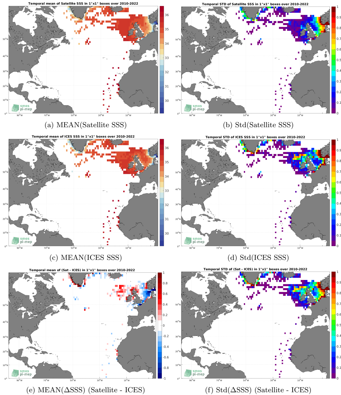
Figure 6: Temporal mean (left) and Std (right) of SSS from SMOS SSS L4 v1 - Weekly (CMEMS-CNR) (top), ICES (middle), and of \Delta SSS (Satellite - ICES). Only match-up pairs are used to generate these maps.
