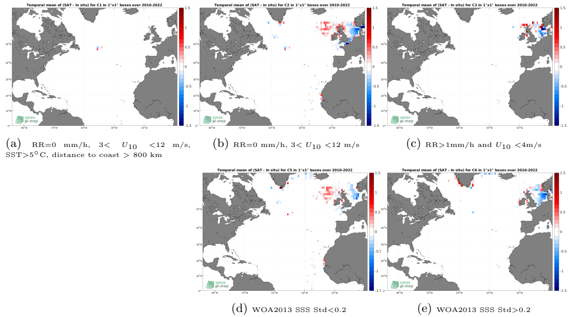
Figure 12: Temporal mean gridded over spatial boxes of size 1^\circ \times 1^\circ of \Delta SSS (SMOS SSS L4 v1 - Weekly (CMEMS-CNR) - ICES) for 5 different subdatasets corresponding to:RR=0 mm/h, 3 < U_{10} < 12 m/s, SST >5^\circ\text{C} , distance to coast > 800 km (a), RR=0 mm/h, 3 < U_{10} < 12 m/s (b), RR >1 mm/h and U_{10} < 4 m/s (c), WOA2013 SSS Std <0.2 (d), WOA2013 SSS Std >0.2 (e).
