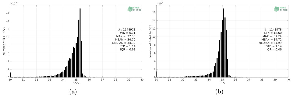
Figure 2: Histograms of SSS from ICES (a) and SMOS SSS L4 v1 - Weekly (CMEMS-CNR) (b) considering all match-up pairs per bins of 0.1 over the North Atlantic Ocean Pi-MEP region and for the full satellite product period.
