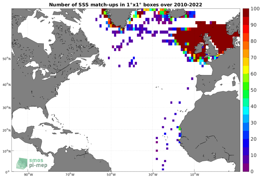
Figure 4: Number of SSS match-ups between ICES SSS and the SMOS SSS L4 v1 - Weekly (CMEMS-CNR) SSS product for the North Atlantic Ocean Pi-MEP region over 1^\circ \times 1^\circ boxes and for the full satellite product period.
