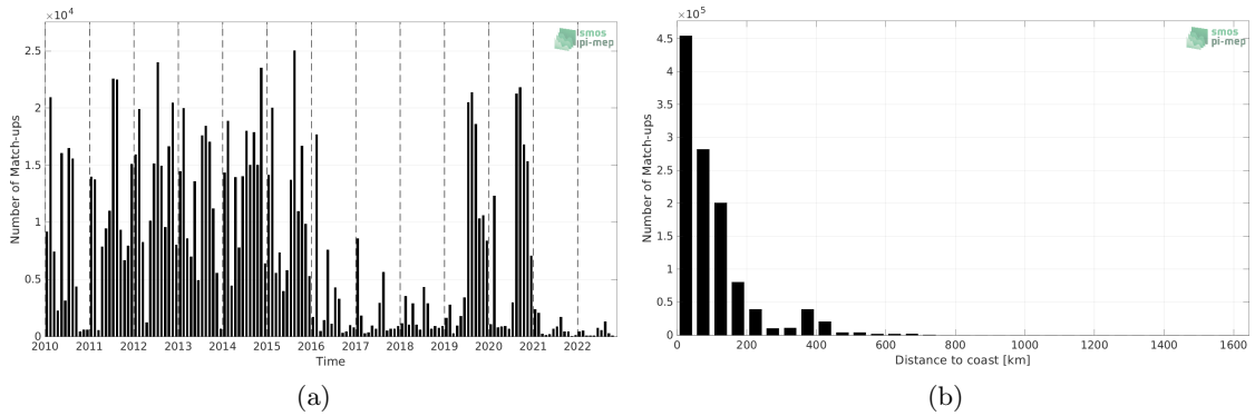
Figure 1: Number of match-ups between ICES and SMOS SSS L4 v1 - Weekly (CMEMS-CNR) SSS as a function of time (a) and as function of the distance to coast (b) over the North Atlantic Ocean Pi-MEP region and for the full satellite product period.
