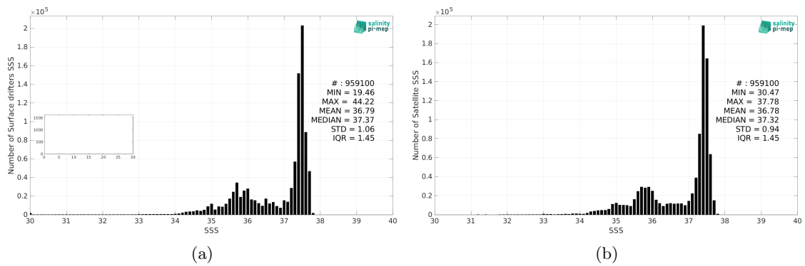
Figure 2: Histograms of SSS from Surface drifters (a) and SMOS SSS L4 v1 - Weekly (CMEMS-CNR) (b) considering all match-up pairs per bins of 0.1 over the North Atlantic Ocean Pi-MEP region and for the full satellite product period.
