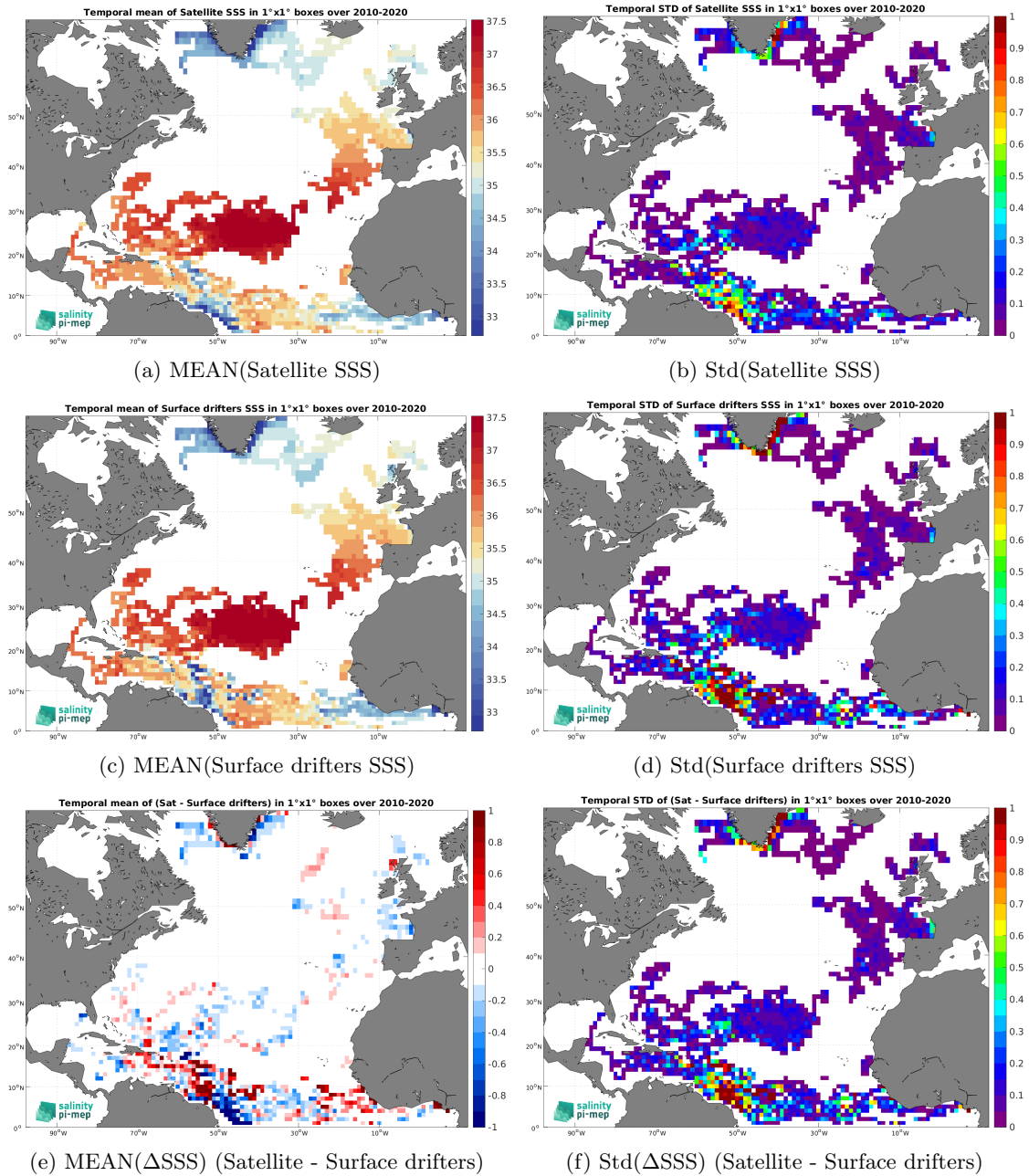
Figure 5: Temporal mean (left) and Std (right) of SSS from SMOS SSS L4 v1 - Weekly (CMEMS-CNR) (top), Surface drifters (middle), and of \Delta SSS (Satellite - Surface drifters). Only match-up pairs are used to generate these maps.
