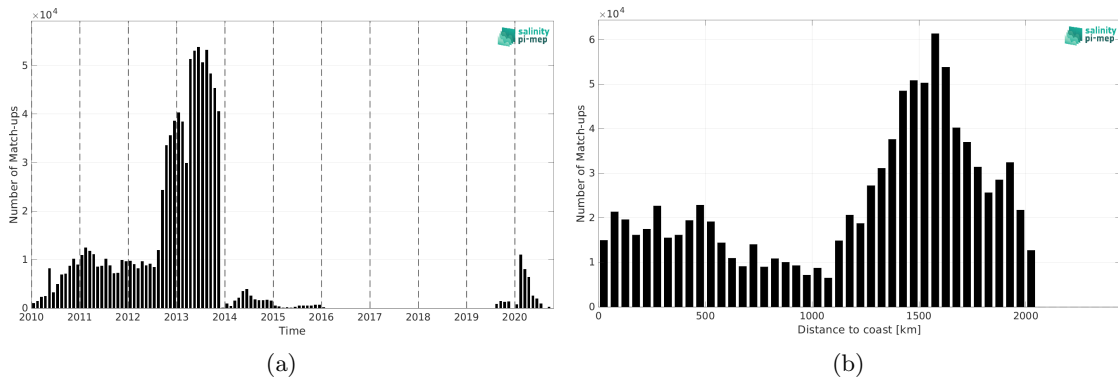
Figure 1: Number of match-ups between Surface drifters and SMOS SSS L4 v1 - Weekly (CMEMS-CNR) SSS as a function of time (a) and as function of the distance to coast (b) over the North Atlantic Ocean Pi-MEP region and for the full satellite product period.
