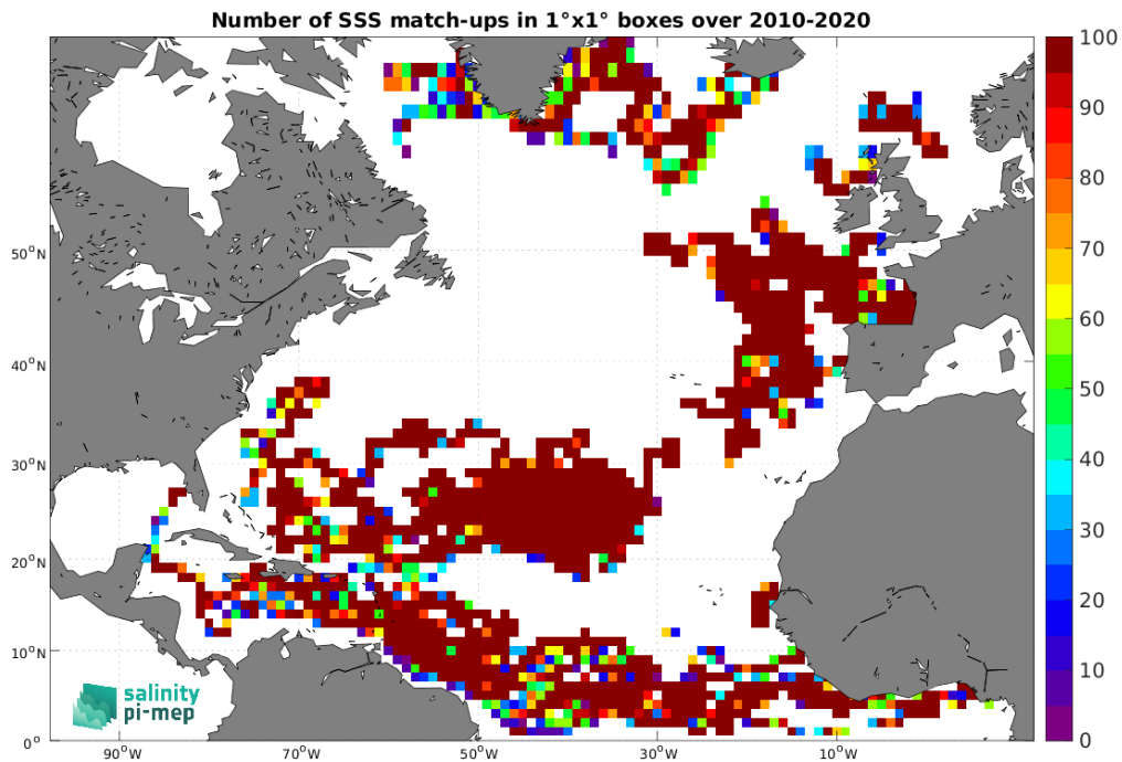
Figure 3: Number of SSS match-ups between Surface drifters SSS and the SMOS SSS L4 v1 - Weekly (CMEMS-CNR) SSS product for the North Atlantic Ocean Pi-MEP region over 1^\circ \times 1^\circ boxes and for the full satellite product period.
