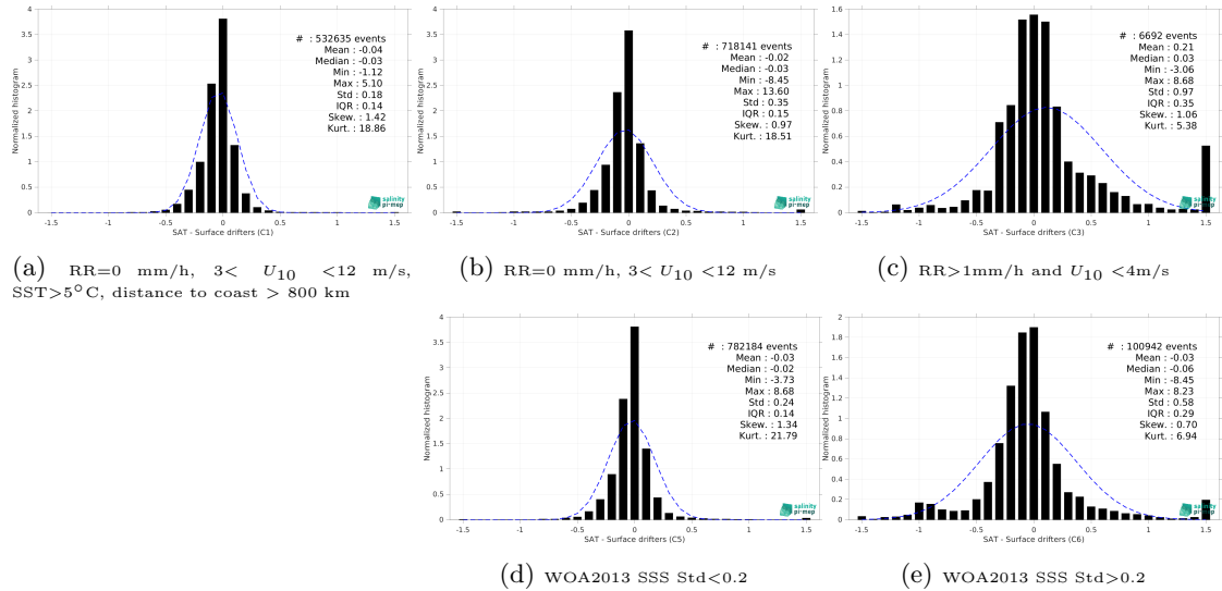
Figure 12: Normalized histogram of \Delta SSS (SMOS SSS L4 v1 - Weekly (CMEMS-CNR) - Surface drifters) for 5 different subdatasets corresponding to: RR=0 mm/h, 3 < U_{10} < 12 m/s, SST>5°C, distance to coast > 800 km (a), RR=0 mm/h, 3 < U_{10} < 12 m/s (b), RR>1mm/h and U_{10} < 4 m/s (c), WOA2013 SSS Std<0.2 (d), WOA2013 SSS Std>0.2 (e).
