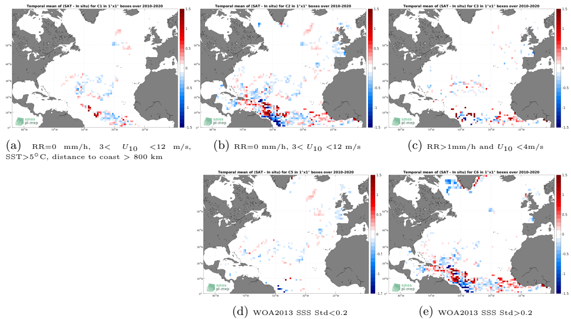
Figure 11: Temporal mean gridded over spatial boxes of size 1^\circ \times 1^\circ of \Delta\text{SSS} (SMOS SSS L4 v1 - Weekly (CMEMS-CNR) - Surface drifters) for 5 different subdatasets corresponding to:RR=0 mm/h, 3 < U_{10} < 12 m/s, SST >5^\circ\text{C} , distance to coast > 800 km (a), RR=0 mm/h, 3 < U_{10} < 12 m/s (b), RR >1 mm/h and U_{10} < 4 m/s (c), WOA2013 SSS Std <0.2 (d), WOA2013 SSS Std >0.2 (e).
