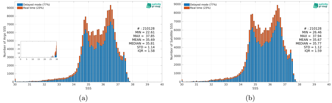
Figure 2: Histograms of SSS from Argo (a) and SMOS SSS L4 v1 - Weekly (CMEMS-CNR) (b) considering all match-up pairs per bins of 0.1 over the North Atlantic Ocean Pi-MEP region and for the full satellite product period.
