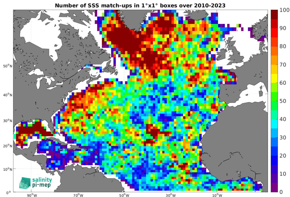
Figure 4: Number of SSS match-ups between Argo SSS and the SMOS SSS L4 v1 - Weekly (CMEMS-CNR) SSS product for the North Atlantic Ocean Pi-MEP region over 1^\circ \times 1^\circ boxes and for the full satellite product period.
