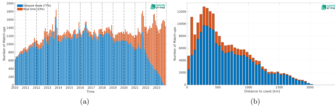
Figure 1: Number of match-ups between Argo and SMOS SSS L4 v1 - Weekly (CMEMS-CNR) SSS as a function of time (a) and as function of the distance to coast (b) over the North Atlantic Ocean Pi-MEP region and for the full satellite product period.
