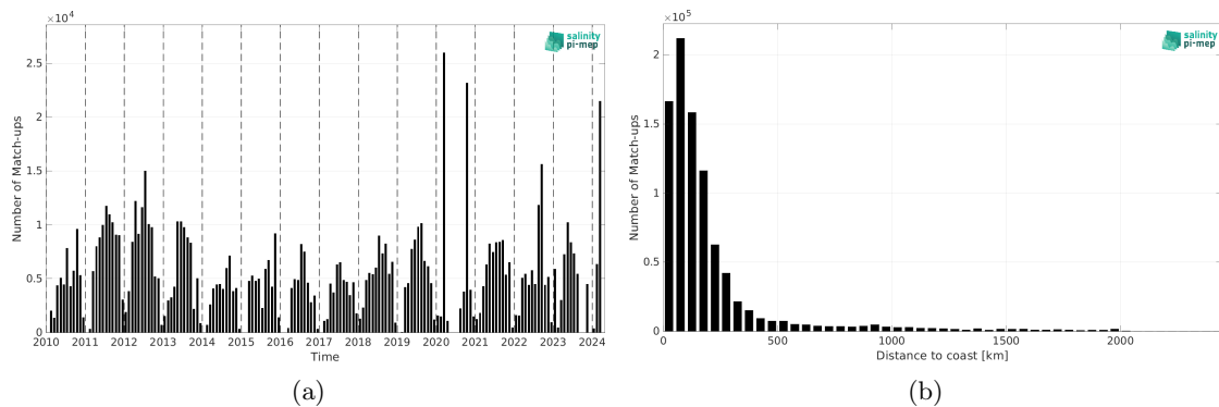
Figure 2: Number of match-ups between TSG (SAMOS) and SMOS SSS L4 v1 - Monthly (CMEMS-CNR) SSS as a function of time (a) and as function of the distance to coast (b) over the North Atlantic Ocean Pi-MEP region and for the full satellite product period.
