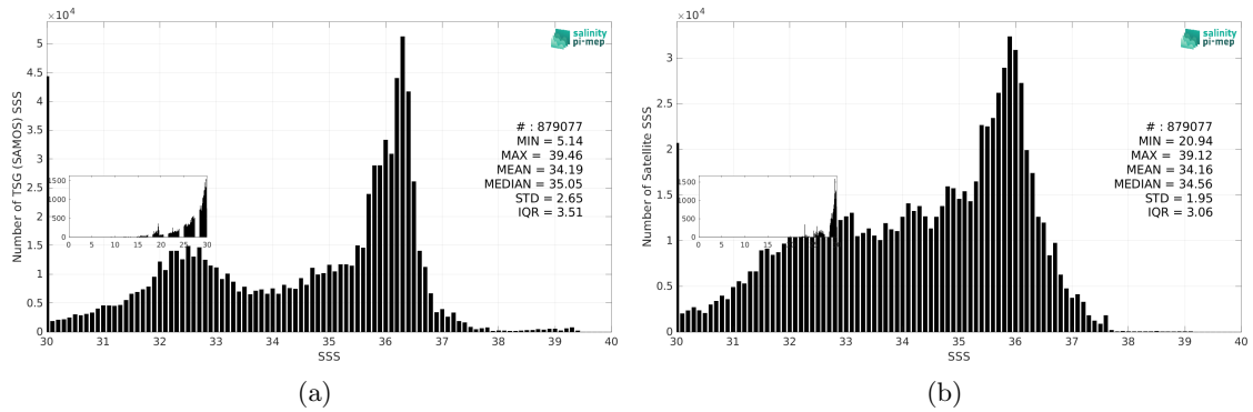
Figure 3: Histograms of SSS from TSG (SAMOS) (a) and SMOS SSS L4 v1 - Monthly (CMEMS-CNR) (b) considering all match-up pairs per bins of 0.1 over the North Atlantic Ocean Pi-MEP region and for the full satellite product period.
