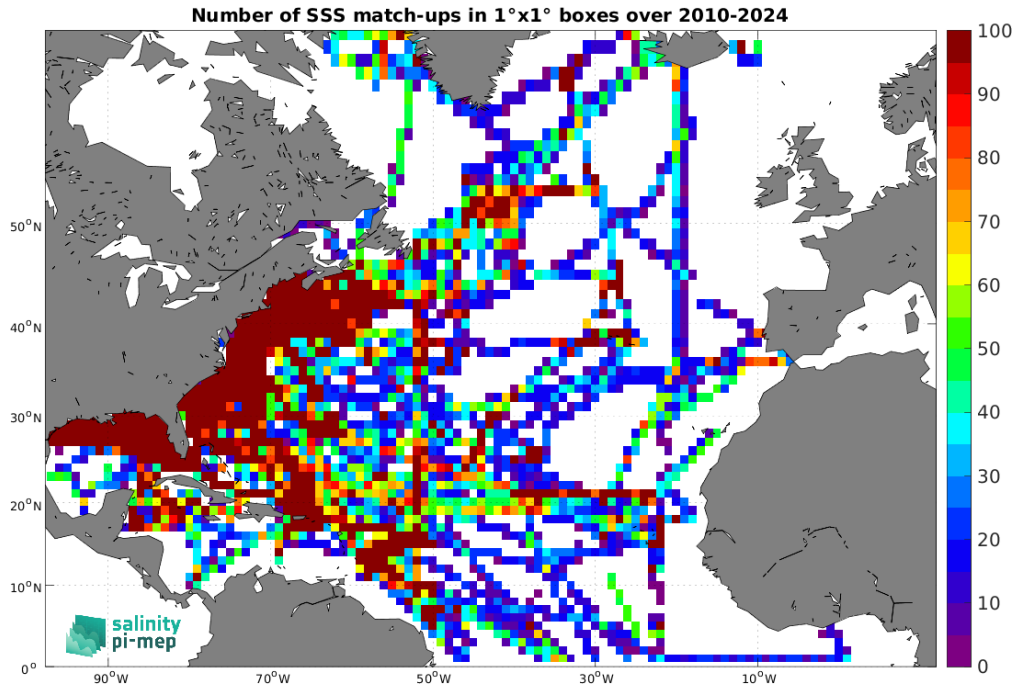
Figure 5: Number of SSS match-ups between TSG (SAMOS) SSS and the SMOS SSS L4 v1 - Monthly (CMEMS-CNR) SSS product for the North Atlantic Ocean Pi-MEP region over 1^\circ \times 1^\circ boxes and for the full satellite product period.
