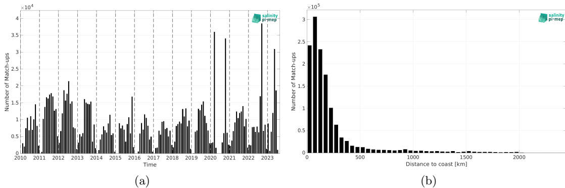
Figure 1: Number of match-ups between TSG (SAMOS) and SMOS SSS L4 v1 - Monthly (CMEMS-CNR) SSS as a function of time (a) and as function of the distance to coast (b) over the North Atlantic Ocean Pi-MEP region and for the full satellite product period.
