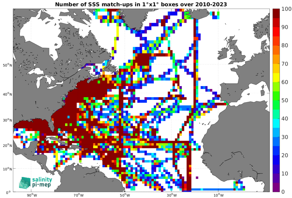
Figure 4: Number of SSS match-ups between TSG (SAMOS) SSS and the SMOS SSS L4 v1 - Monthly (CMEMS-CNR) SSS product for the North Atlantic Ocean Pi-MEP region over 1^\circ \times 1^\circ boxes and for the full satellite product period.
