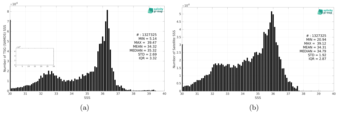
Figure 2: Histograms of SSS from TSG (SAMOS) (a) and SMOS SSS L4 v1 - Monthly (CMEMS-CNR) (b) considering all match-up pairs per bins of 0.1 over the North Atlantic Ocean Pi-MEP region and for the full satellite product period.
