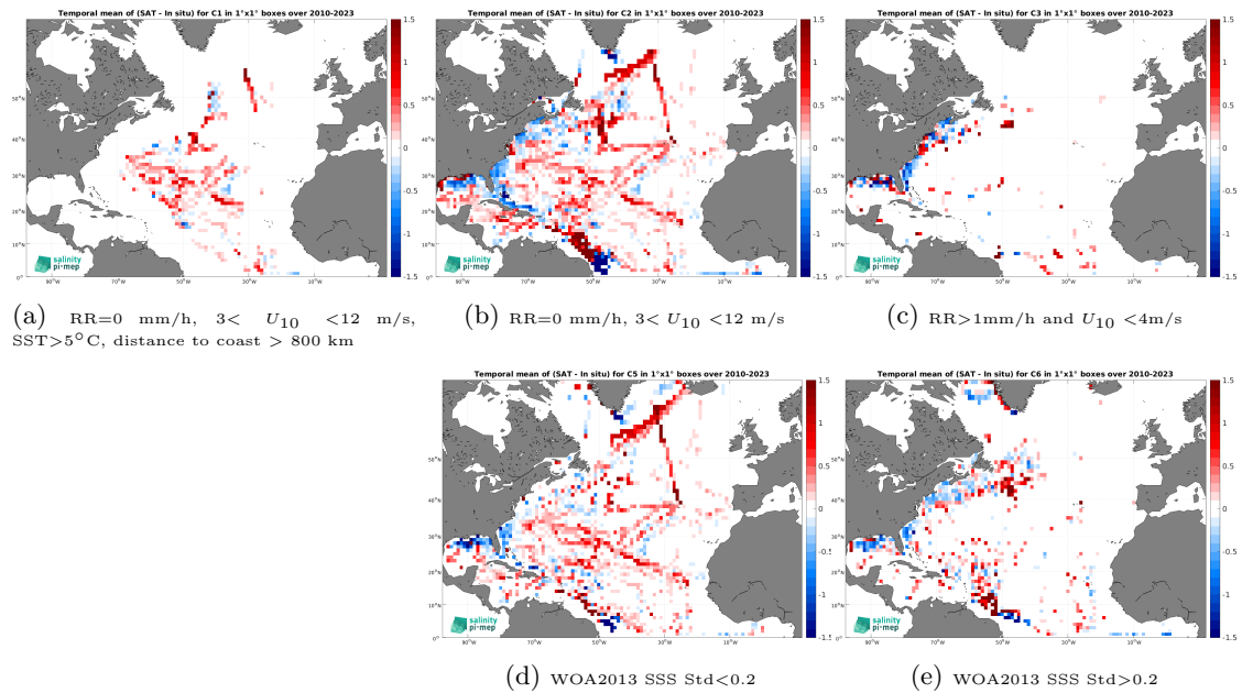
Figure 12: Temporal mean gridded over spatial boxes of size 1^\circ \times 1^\circ of \Delta\text{SSS} (SMOS SSS L4 v1 - Monthly (CMEMS-CNR) - TSG (SAMOS)) for 5 different subdatasets corresponding to:RR=0 mm/h, 3 < U_{10} < 12 m/s, SST > 5^\circ\text{C} , distance to coast > 800 km (a), RR=0 mm/h, 3 < U_{10} < 12 m/s (b), RR > 1 mm/h and U_{10} < 4 m/s (c), WOA2013 SSS Std < 0.2 (d), WOA2013 SSS Std > 0.2 (e).
