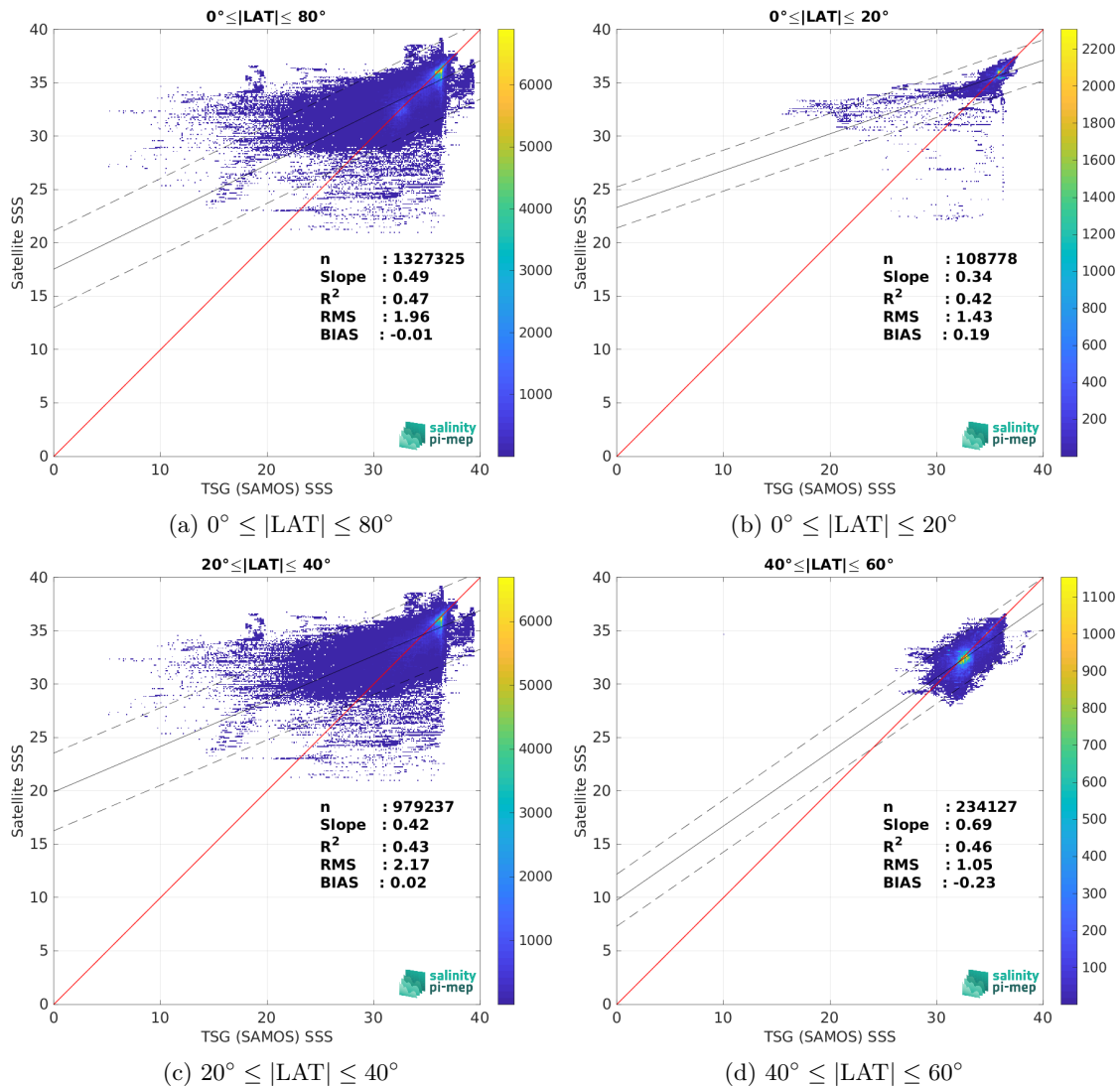
Figure 9: Contour maps of the concentration of SMOS SSS L4 v1 - Monthly (CMEMS-CNR) SSS (y-axis) versus TSG (SAMOS) SSS (x-axis) at match-up pairs for different latitude bands. For each plot, the red line shows x=y . The black thin and dashed lines indicate a linear fit through the data cloud and the \pm 95\% confidence levels, respectively. The number match-up pairs n , the slope and R^2 coefficient of the linear fit, the root mean square (RMS) and the mean bias between satellite and in situ data are indicated for each latitude band in each plots.
