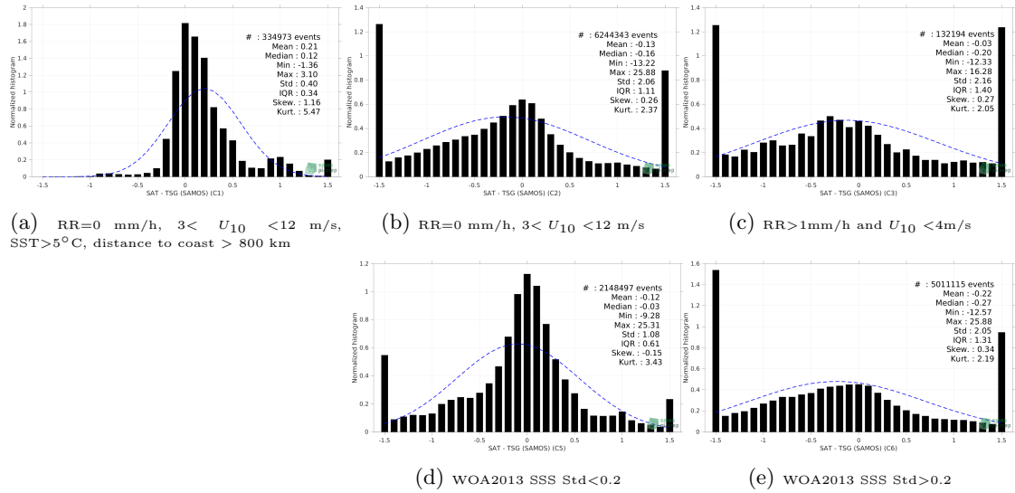
Figure 13: Normalized histogram of \Delta\text{SSS} (SMOS SSS L4 v1 - Monthly (CMEMS-CNR) - TSG (SAMOS)) for 5 different subdatasets corresponding to: RR=0 mm/h, 3 < U_{10} < 12 m/s, SST>5°C, distance to coast > 800 km (a), RR=0 mm/h, 3 < U_{10} < 12 m/s (b), RR>1mm/h and U_{10} < 4 m/s (c), WOA2013 SSS Std<0.2 (d), WOA2013 SSS Std>0.2 (e).
