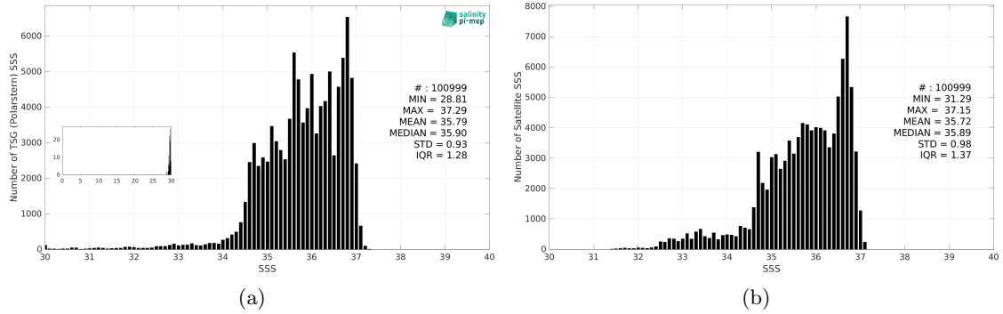
Figure 3: Histograms of SSS from TSG (Polarstern) (a) and SMOS SSS L4 v1 - Monthly (CMEMS-CNR) (b) considering all match-up pairs per bins of 0.1 over the North Atlantic Ocean Pi-MEP region and for the full satellite product period.
