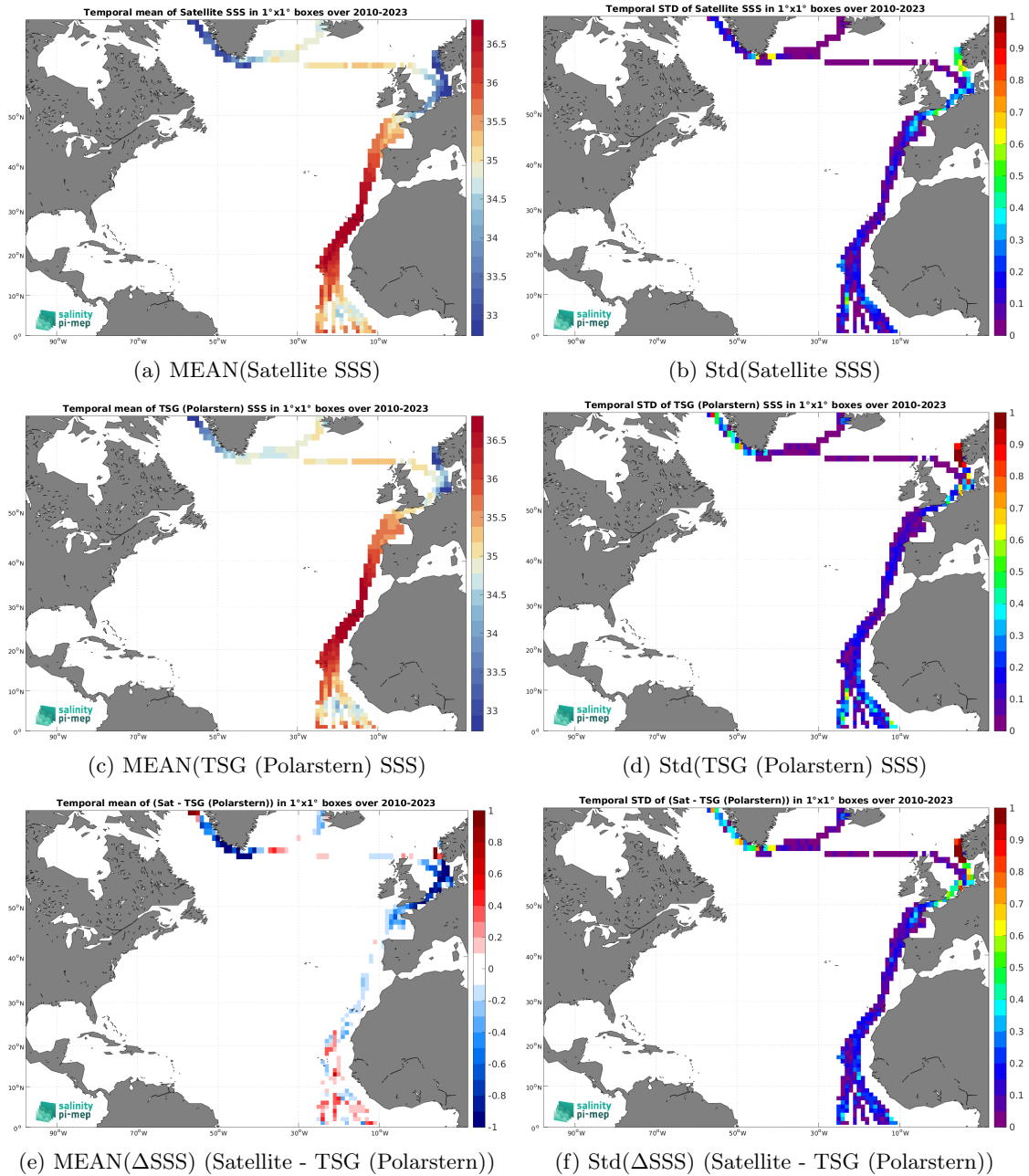
Figure 7: Temporal mean (left) and Std (right) of SSS from SMOS SSS L4 v1 - Monthly (CMEMS-CNR) (top), TSG (Polarstern) (middle), and of \Delta SSS (Satellite - TSG (Polarstern)). Only match-up pairs are used to generate these maps.
