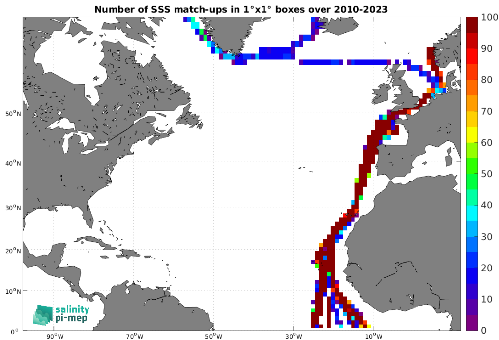
Figure 5: Number of SSS match-ups between TSG (Polarstern) SSS and the SMOS SSS L4 v1 - Monthly (CMEMS-CNR) SSS product for the North Atlantic Ocean Pi-MEP region over 1^\circ \times 1^\circ boxes and for the full satellite product period.
