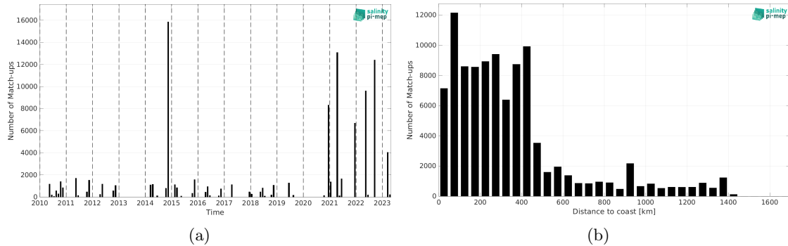
Figure 2: Number of match-ups between TSG (Polarstern) and SMOS SSS L4 v1 - Monthly (CMEMS-CNR) SSS as a function of time (a) and as function of the distance to coast (b) over the North Atlantic Ocean Pi-MEP region and for the full satellite product period.
