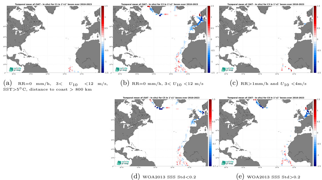
Figure 14: Temporal mean gridded over spatial boxes of size 1^\circ \times 1^\circ of \Delta\text{SSS} (SMOS SSS L4 v1 - Monthly (CMEMS-CNR) - TSG (Polarstern)) for 5 different subdatasets corresponding to:RR=0 mm/h, 3 < U_{10} < 12 m/s, SST >5^\circ\text{C} , distance to coast > 800 km (a), RR=0 mm/h, 3 < U_{10} < 12 m/s (b), RR >1 mm/h and U_{10} < 4 m/s (c), WOA2013 SSS Std <0.2 (d), WOA2013 SSS Std >0.2 (e).
