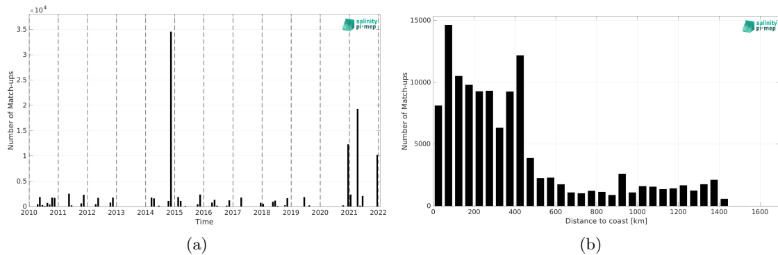
Figure 1: Number of match-ups between TSG (Polarstern) and SMOS SSS L4 v1 - Monthly (CMEMS-CNR) SSS as a function of time (a) and as function of the distance to coast (b) over the North Atlantic Ocean Pi-MEP region and for the full satellite product period.
