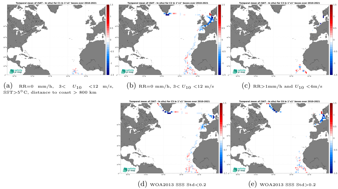
Figure 12: Temporal mean gridded over spatial boxes of size 1^\circ \times 1^\circ of \Delta\text{SSS} (SMOS SSS L4 v1 - Monthly (CMEMS-CNR) - TSG (Polarstern)) for 5 different subdatasets corresponding to:RR=0 mm/h, 3 < U_{10} < 12 m/s, SST >5^\circ\text{C} , distance to coast > 800 km (a), RR=0 mm/h, 3 < U_{10} < 12 m/s (b), RR >1 mm/h and U_{10} < 4 m/s (c), WOA2013 SSS Std <0.2 (d), WOA2013 SSS Std >0.2 (e).
