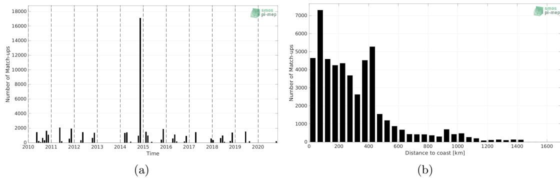
Figure 1: Number of match-ups between TSG (Polarstern) and SMOS SSS L4 v1 - Monthly (CMEMS-CNR) SSS as a function of time (a) and as function of the distance to coast (b) over the North Atlantic Ocean Pi-MEP region and for the full satellite product period.
