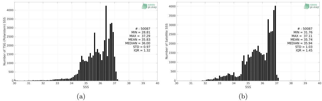
Figure 2: Histograms of SSS from TSG (Polarstern) (a) and SMOS SSS L4 v1 - Monthly (CMEMS-CNR) (b) considering all match-up pairs per bins of 0.1 over the North Atlantic Ocean Pi-MEP region and for the full satellite product period.
