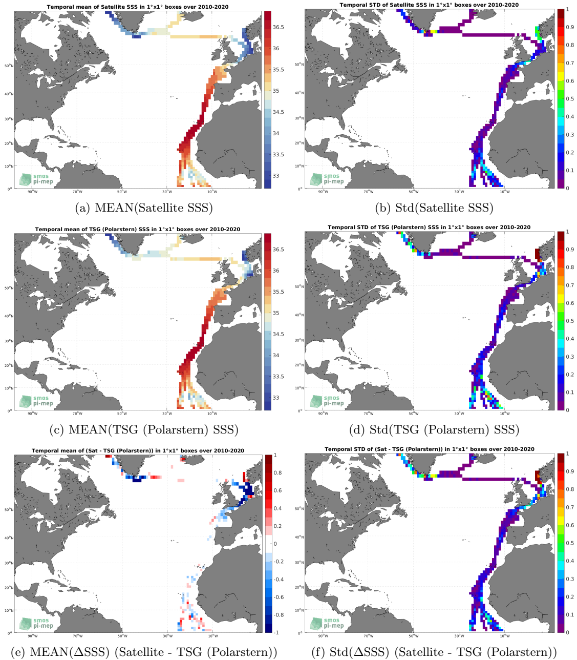
Figure 6: Temporal mean (left) and Std (right) of SSS from SMOS SSS L4 v1 - Monthly (CMEMS-CNR) (top), TSG (Polarstern) (middle), and of \Delta SSS (Satellite - TSG (Polarstern)). Only match-up pairs are used to generate these maps.
