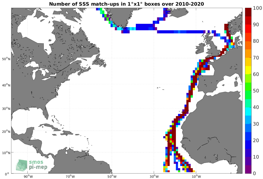
Figure 4: Number of SSS match-ups between TSG (Polarstern) SSS and the SMOS SSS L4 v1 - Monthly (CMEMS-CNR) SSS product for the North Atlantic Ocean Pi-MEP region over 1^\circ \times 1^\circ boxes and for the full satellite product period.
