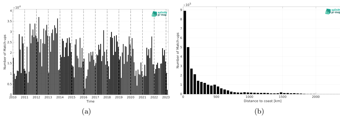
Figure 2: Number of match-ups between TSG (LEGOS-DM) and SMOS SSS L4 v1 - Monthly (CMEMS-CNR) SSS as a function of time (a) and as function of the distance to coast (b) over the North Atlantic Ocean Pi-MEP region and for the full satellite product period.
