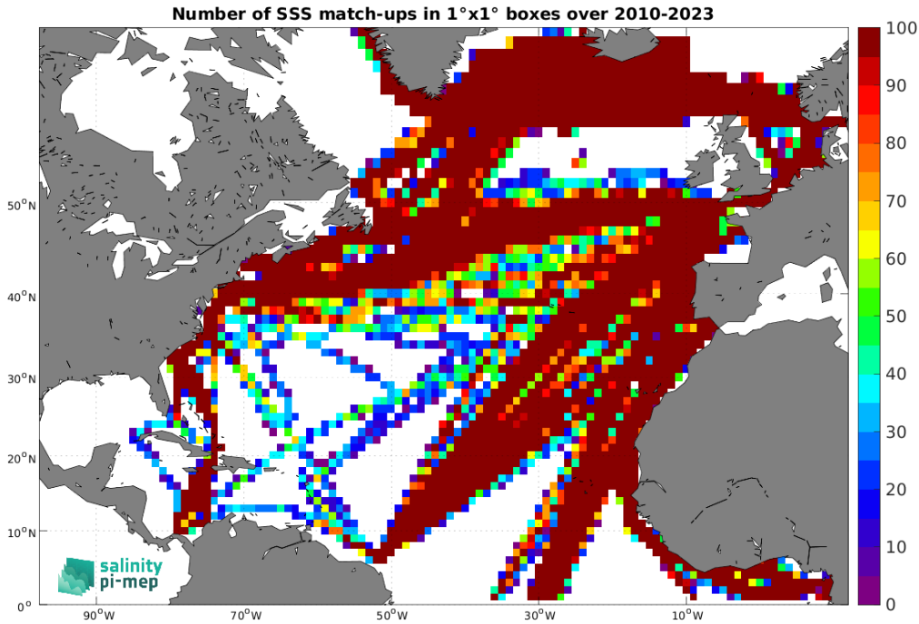
Figure 5: Number of SSS match-ups between TSG (LEGOS-DM) SSS and the SMOS SSS L4 v1 - Monthly (CMEMS-CNR) SSS product for the North Atlantic Ocean Pi-MEP region over 1^\circ \times 1^\circ boxes and for the full satellite product period.
