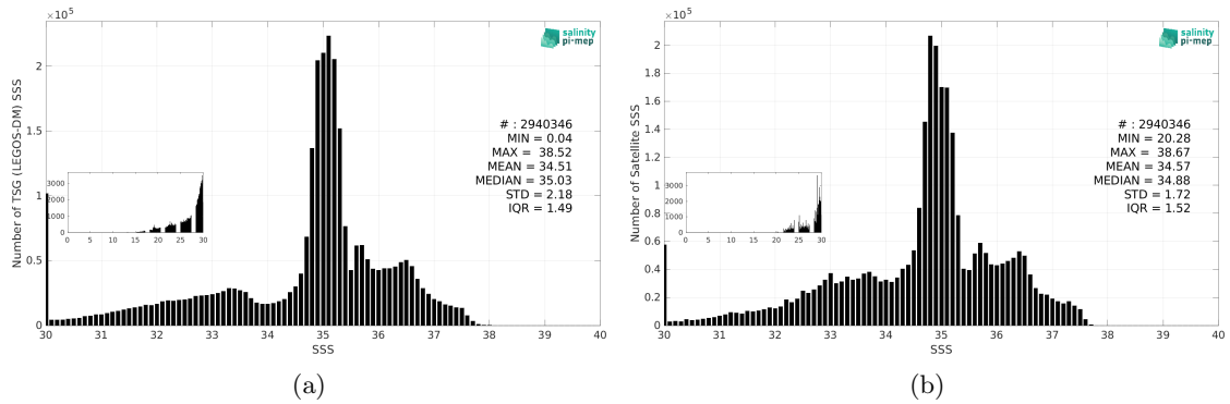
Figure 3: Histograms of SSS from TSG (LEGOS-DM) (a) and SMOS SSS L4 v1 - Monthly (CMEMS-CNR) (b) considering all match-up pairs per bins of 0.1 over the North Atlantic Ocean Pi-MEP region and for the full satellite product period.
