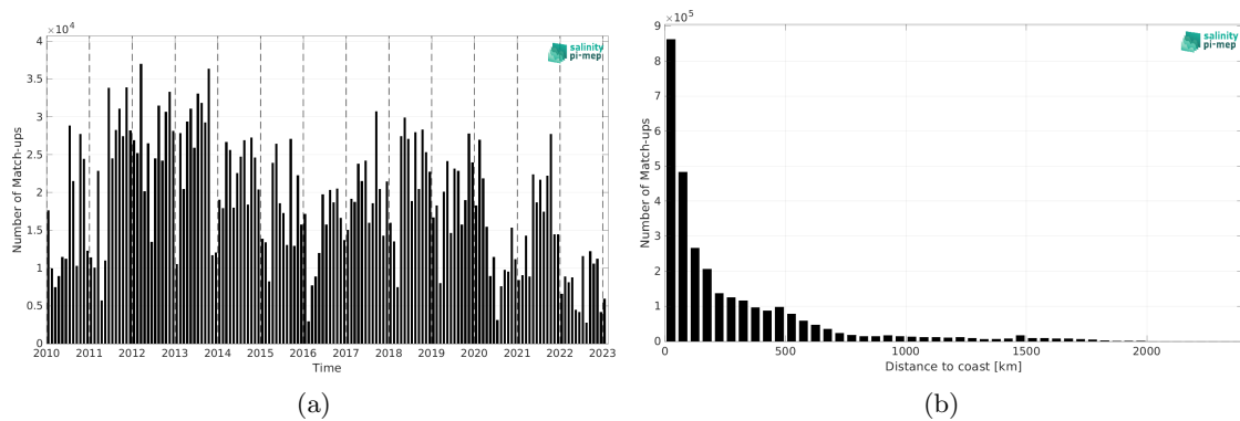
Figure 2: Number of match-ups between TSG (LEGOS-DM) and SMOS SSS L4 v1 - Monthly (CMEMS-CNR) SSS as a function of time (a) and as function of the distance to coast (b) over the North Atlantic Ocean Pi-MEP region and for the full satellite product period.
