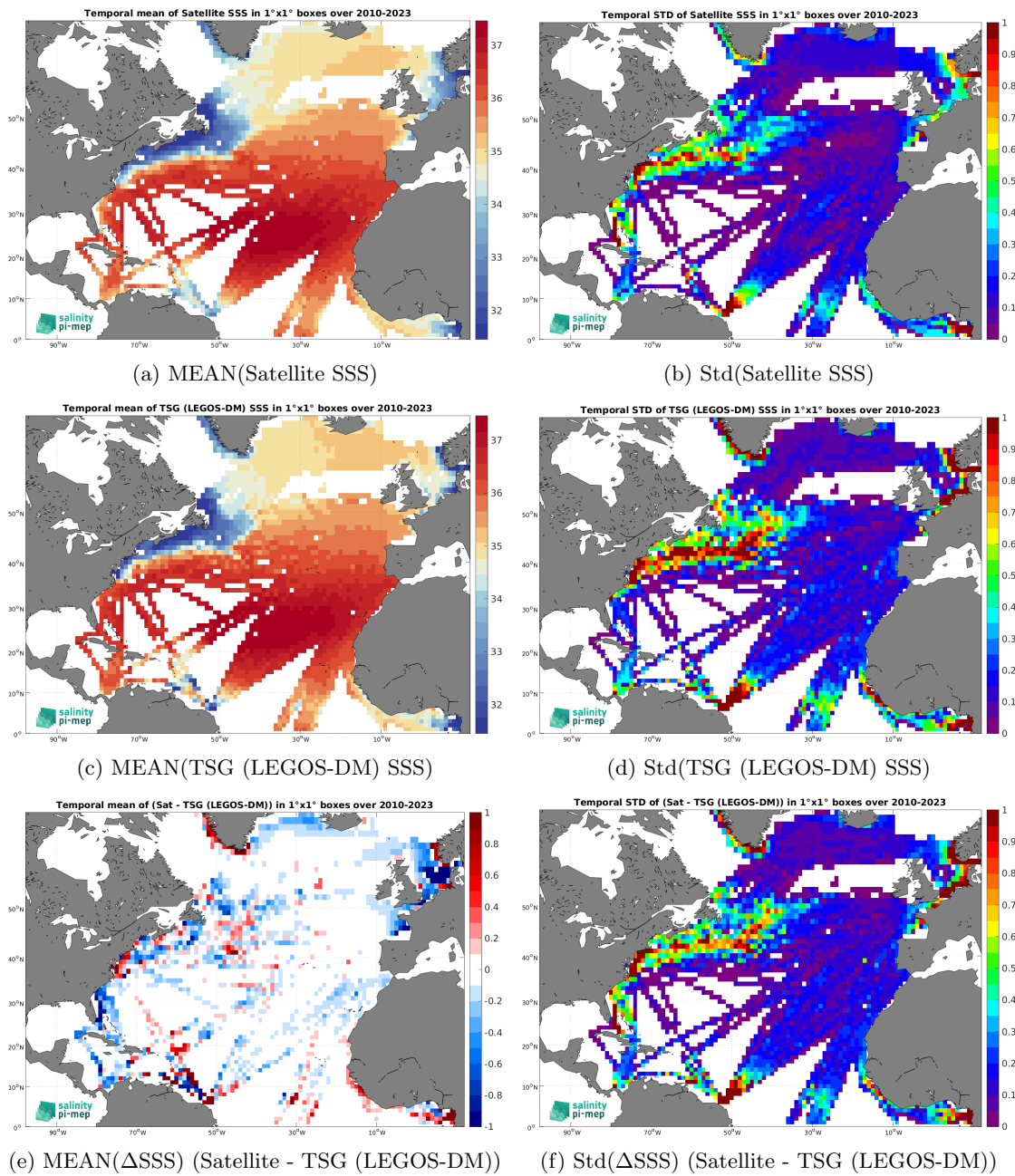
Figure 7: Temporal mean (left) and Std (right) of SSS from SMOS SSS L4 v1 - Monthly (CMEMS-CNR) (top), TSG (LEGOS-DM) (middle), and of \Delta SSS (Satellite - TSG (LEGOS-DM)). Only match-up pairs are used to generate these maps.
