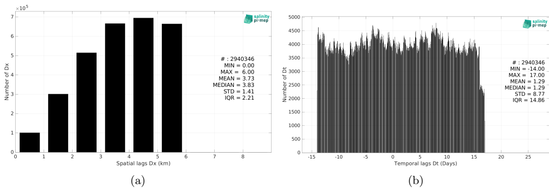
Figure 6: Histograms of the spatial (a) and temporal (b) lags between the location/time of the TSG (LEGOS-DM) measurement and the date of the corresponding SMOS SSS L4 v1 - Monthly (CMEMS-CNR) SSS pixel.
