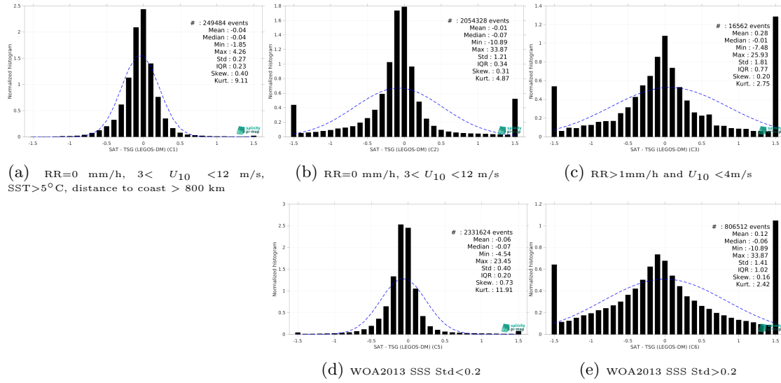
Figure 13: Normalized histogram of \Delta\text{SSS} (SMOS SSS L4 v1 - Monthly (CMEMS-CNR) - TSG (LEGOS-DM)) for 5 different subdatasets corresponding to: RR=0 mm/h, 3 < U_{10} < 12 m/s, SST>5°C, distance to coast > 800 km (a), RR=0 mm/h, 3 < U_{10} < 12 m/s (b), RR>1mm/h and U_{10} < 4 m/s (c), WOA2013 SSS Std<0.2 (d), WOA2013 SSS Std>0.2 (e).
