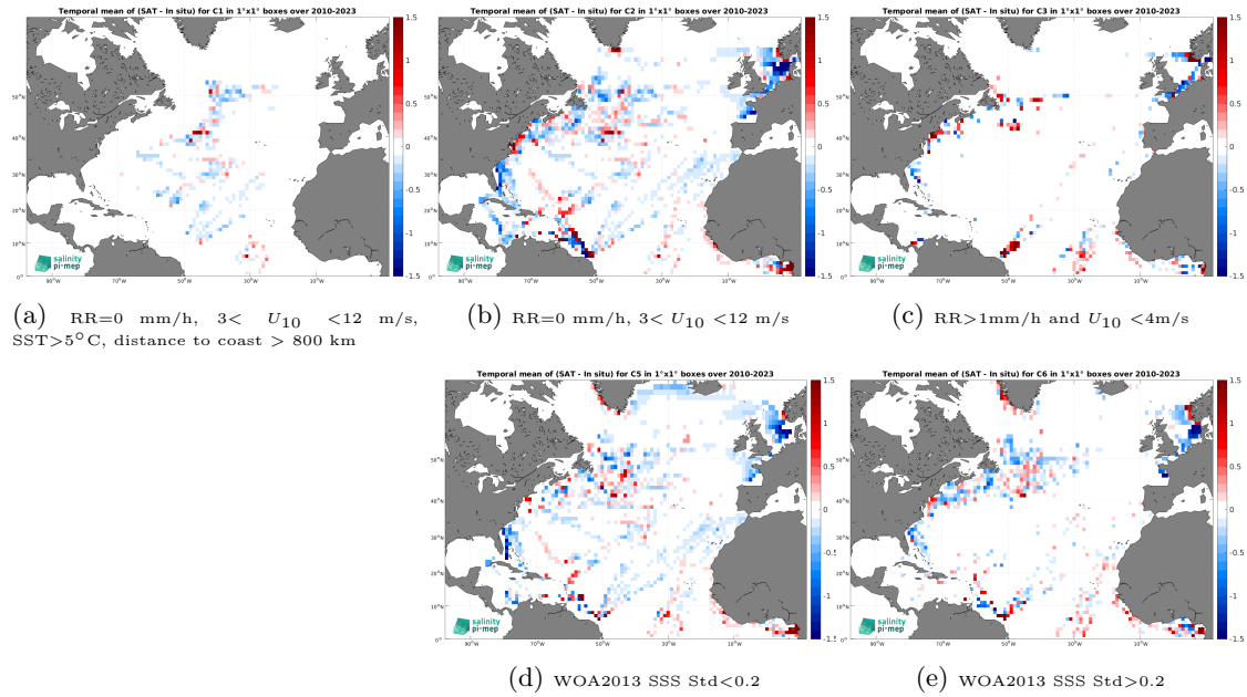
Figure 12: Temporal mean gridded over spatial boxes of size 1^\circ \times 1^\circ of \Delta\text{SSS} (SMOS SSS L4 v1 - Monthly (CMEMS-CNR) - TSG (LEGOS-DM)) for 5 different subdatasets corresponding to:RR=0 mm/h, 3 < U_{10} < 12 m/s, SST >5^\circ\text{C} , distance to coast > 800 km (a), RR=0 mm/h, 3 < U_{10} < 12 m/s (b), RR >1 mm/h and U_{10} < 4 m/s (c), WOA2013 SSS Std <0.2 (d), WOA2013 SSS Std >0.2 (e).
