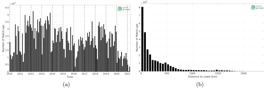
Figure 1: Number of match-ups between TSG (LEGOS-DM) and SMOS SSS L4 v1 - Monthly (CMEMS-CNR) SSS as a function of time (a) and as function of the distance to coast (b) over the North Atlantic Ocean Pi-MEP region and for the full satellite product period.
