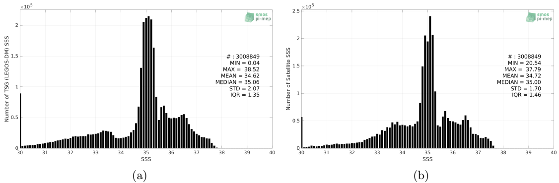
Figure 2: Histograms of SSS from TSG (LEGOS-DM) (a) and SMOS SSS L4 v1 - Monthly (CMEMS-CNR) (b) considering all match-up pairs per bins of 0.1 over the North Atlantic Ocean Pi-MEP region and for the full satellite product period.
