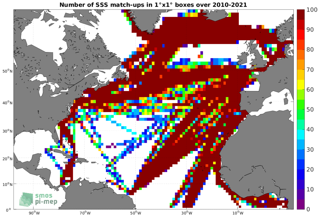
Figure 4: Number of SSS match-ups between TSG (LEGOS-DM) SSS and the SMOS SSS L4 v1 - Monthly (CMEMS-CNR) SSS product for the North Atlantic Ocean Pi-MEP region over 1^\circ \times 1^\circ boxes and for the full satellite product period.
