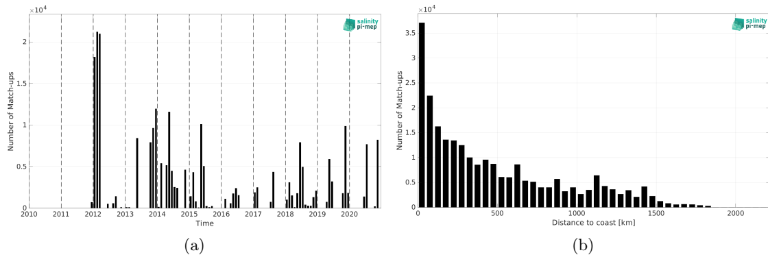
Figure 2: Number of match-ups between TSG (GOSUD-Sailing-ship) and SMOS SSS L4 v1 - Monthly (CMEMS-CNR) SSS as a function of time (a) and as function of the distance to coast (b) over the North Atlantic Ocean Pi-MEP region and for the full satellite product period.
