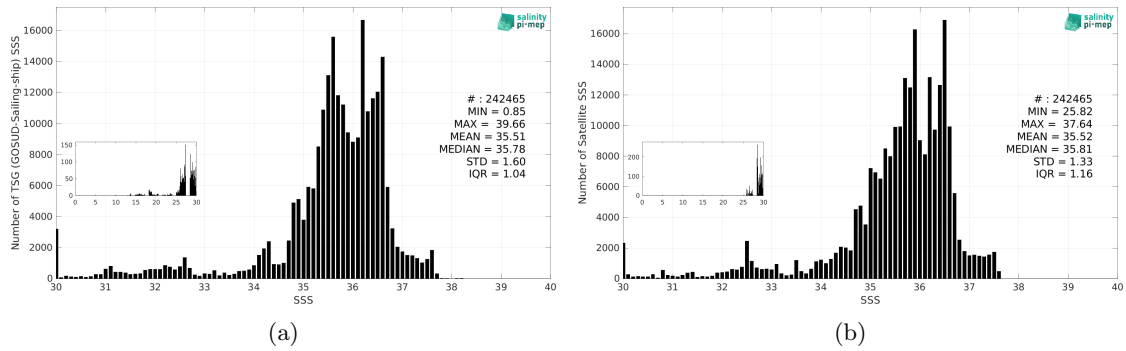
Figure 3: Histograms of SSS from TSG (GOSUD-Sailing-ship) (a) and SMOS SSS L4 v1 - Monthly (CMEMS-CNR) (b) considering all match-up pairs per bins of 0.1 over the North Atlantic Ocean Pi-MEP region and for the full satellite product period.
