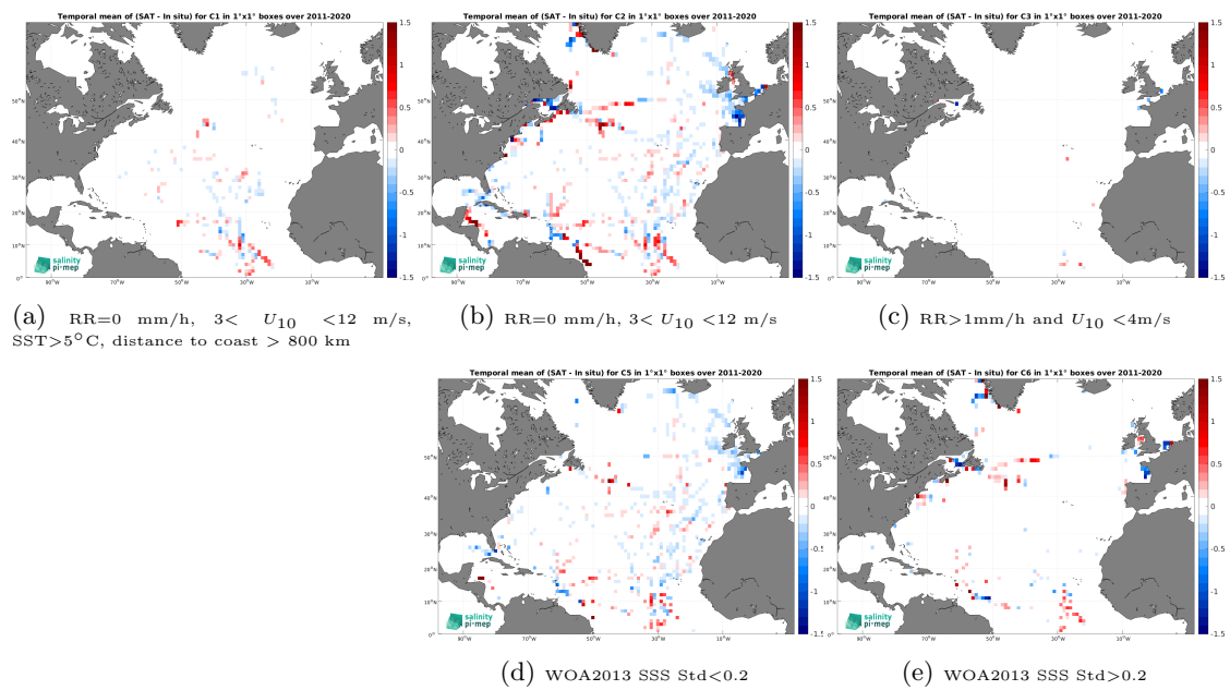
Figure 14: Temporal mean gridded over spatial boxes of size 1^\circ \times 1^\circ of \Delta\text{SSS} (SMOS SSS L4 v1 - Monthly (CMEMS-CNR) - TSG (GOSUD-Sailing-ship)) for 5 different subdatasets corresponding to:RR=0 mm/h, 3 < U_{10} < 12 m/s, SST >5^\circ\text{C} , distance to coast > 800 km (a), RR=0 mm/h, 3 < U_{10} < 12 m/s (b), RR >1 mm/h and U_{10} < 4 m/s (c), WOA2013 SSS Std <0.2 (d), WOA2013 SSS Std >0.2 (e).
