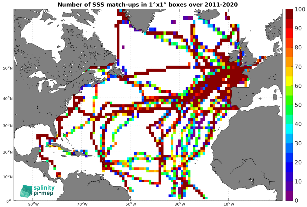
Figure 5: Number of SSS match-ups between TSG (GOSUD-Sailing-ship) SSS and the SMOS SSS L4 v1 - Monthly (CMEMS-CNR) SSS product for the North Atlantic Ocean Pi-MEP region over 1^\circ \times 1^\circ boxes and for the full satellite product period.
