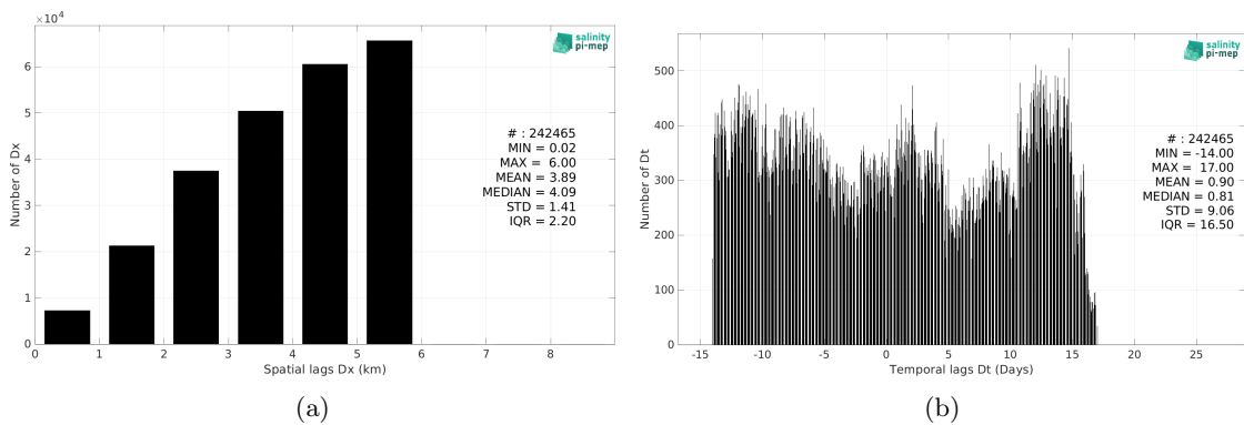
Figure 6: Histograms of the spatial (a) and temporal (b) lags between the location/time of the TSG (GOSUD-Sailing-ship) measurement and the date of the corresponding SMOS SSS L4 v1 - Monthly (CMEMS-CNR) SSS pixel.
