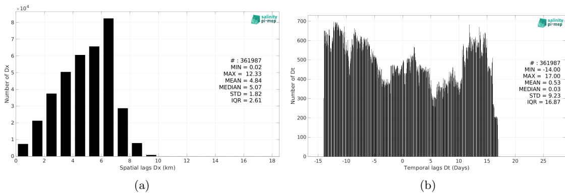
Figure 5: Histograms of the spatial (a) and temporal (b) lags between the location/time of the TSG (GOSUD-Sailing-ship) measurement and the date of the corresponding SMOS SSS L4 v1 - Monthly (CMEMS-CNR) SSS pixel.
