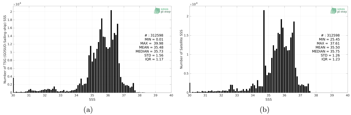
Figure 2: Histograms of SSS from TSG (GOSUD-Sailing-ship) (a) and SMOS SSS L4 v1 - Monthly (CMEMS-CNR) (b) considering all match-up pairs per bins of 0.1 over the North Atlantic Ocean Pi-MEP region and for the full satellite product period.
