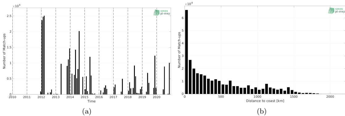
Figure 1: Number of match-ups between TSG (GOSUD-Sailing-ship) and SMOS SSS L4 v1 - Monthly (CMEMS-CNR) SSS as a function of time (a) and as function of the distance to coast (b) over the North Atlantic Ocean Pi-MEP region and for the full satellite product period.
