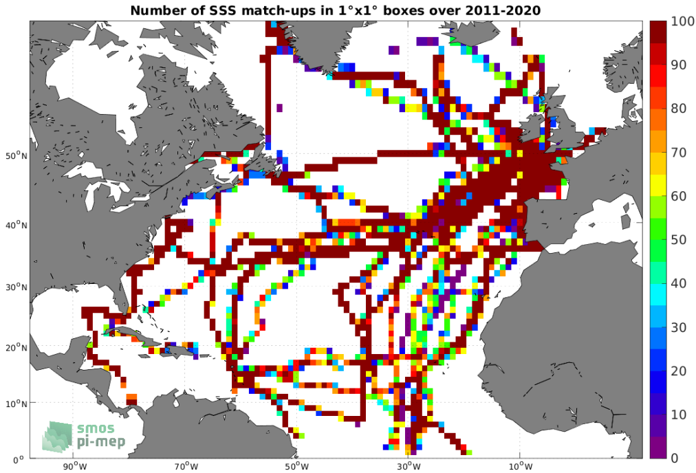
Figure 4: Number of SSS match-ups between TSG (GOSUD-Sailing-ship) SSS and the SMOS SSS L4 v1 - Monthly (CMEMS-CNR) SSS product for the North Atlantic Ocean Pi-MEP region over 1^\circ \times 1^\circ boxes and for the full satellite product period.
