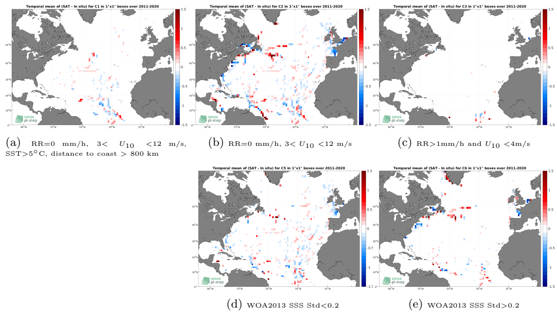
Figure 12: Temporal mean gridded over spatial boxes of size 1^\circ \times 1^\circ of \Delta\text{SSS} (SMOS SSS L4 v1 - Monthly (CMEMS-CNR) - TSG (GOSUD-Sailing-ship)) for 5 different subdatasets corresponding to:RR=0 mm/h, 3 < U_{10} < 12 m/s, SST >5^\circ\text{C} , distance to coast > 800 km (a), RR=0 mm/h, 3 < U_{10} < 12 m/s (b), RR >1 mm/h and U_{10} < 4 m/s (c), WOA2013 SSS Std <0.2 (d), WOA2013 SSS Std >0.2 (e).
