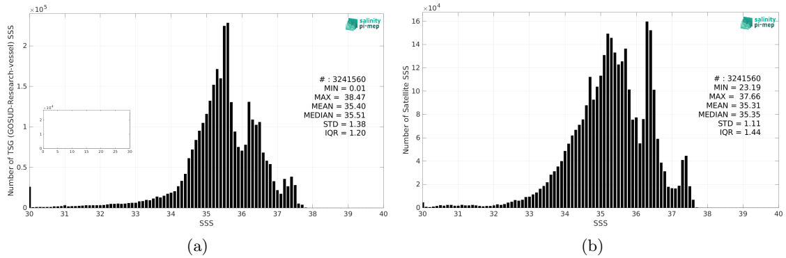
Figure 2: Histograms of SSS from TSG (GOSUD-Research-vessel) (a) and SMOS SSS L4 v1 - Monthly (CMEMS-CNR) (b) considering all match-up pairs per bins of 0.1 over the North Atlantic Ocean Pi-MEP region and for the full satellite product period.
