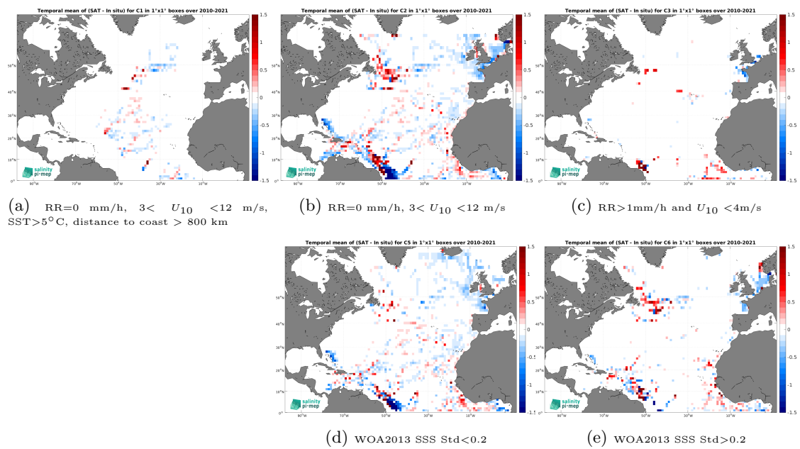
Figure 12: Temporal mean gridded over spatial boxes of size 1^\circ \times 1^\circ of \Delta\text{SSS} (SMOS SSS L4 v1 - Monthly (CMEMS-CNR) - TSG (GOSUD-Research-vessel)) for 5 different subdatasets corresponding to:RR=0 mm/h, 3 < U_{10} < 12 m/s, SST >5^\circ\text{C} , distance to coast > 800 km (a), RR=0 mm/h, 3 < U_{10} < 12 m/s (b), RR >1 mm/h and U_{10} < 4 m/s (c), WOA2013 SSS Std <0.2 (d), WOA2013 SSS Std >0.2 (e).
