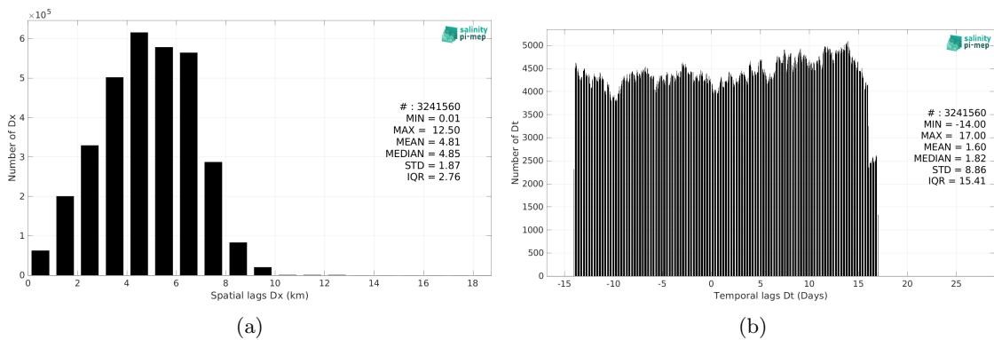
Figure 5: Histograms of the spatial (a) and temporal (b) lags between the location/time of the TSG (GOSUD-Research-vessel) measurement and the date of the corresponding SMOS SSS L4 v1 - Monthly (CMEMS-CNR) SSS pixel.
