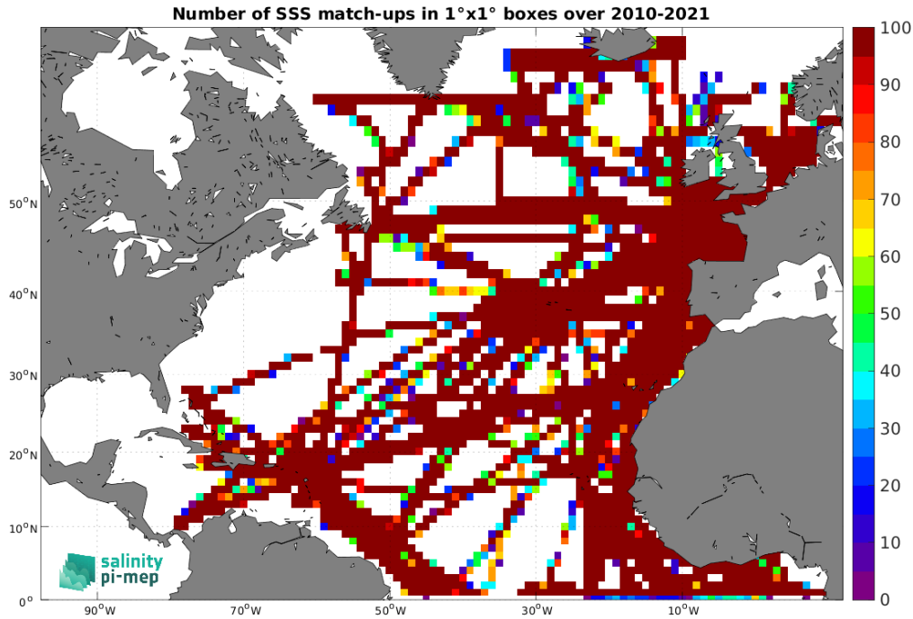
Figure 4: Number of SSS match-ups between TSG (GOSUD-Research-vessel) SSS and the SMOS SSS L4 v1 - Monthly (CMEMS-CNR) SSS product for the North Atlantic Ocean Pi-MEP region over 1^\circ \times 1^\circ boxes and for the full satellite product period.
