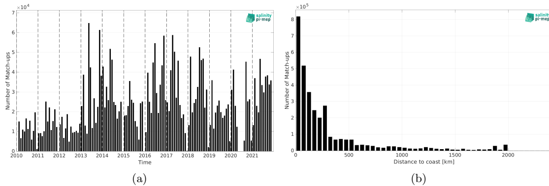
Figure 1: Number of match-ups between TSG (GOSUD-Research-vessel) and SMOS SSS L4 v1 - Monthly (CMEMS-CNR) SSS as a function of time (a) and as function of the distance to coast (b) over the North Atlantic Ocean Pi-MEP region and for the full satellite product period.
