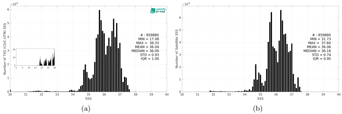
Figure 3: Histograms of SSS from TSG (CSIC-UTM) (a) and SMOS SSS L4 v1 - Monthly (CMEMS-CNR) (b) considering all match-up pairs per bins of 0.1 over the North Atlantic Ocean Pi-MEP region and for the full satellite product period.
