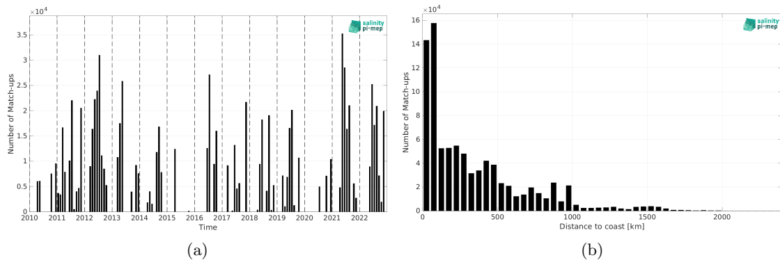
Figure 2: Number of match-ups between TSG (CSIC-UTM) and SMOS SSS L4 v1 - Monthly (CMEMS-CNR) SSS as a function of time (a) and as function of the distance to coast (b) over the North Atlantic Ocean Pi-MEP region and for the full satellite product period.
