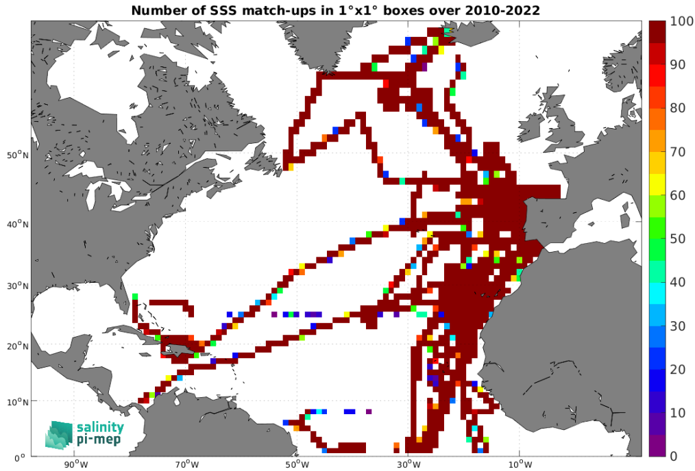
Figure 5: Number of SSS match-ups between TSG (CSIC-UTM) SSS and the SMOS SSS L4 v1 - Monthly (CMEMS-CNR) SSS product for the North Atlantic Ocean Pi-MEP region over 1^\circ \times 1^\circ boxes and for the full satellite product period.
