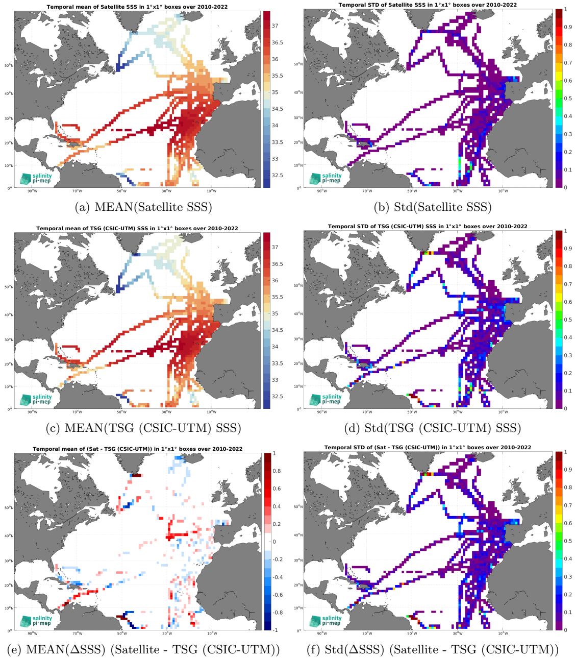
Figure 7: Temporal mean (left) and Std (right) of SSS from SMOS SSS L4 v1 - Monthly (CMEMS-CNR) (top), TSG (CSIC-UTM) (middle), and of \Delta SSS (Satellite - TSG (CSIC-UTM)). Only match-up pairs are used to generate these maps.
