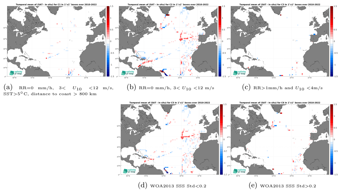
Figure 14: Temporal mean gridded over spatial boxes of size 1^\circ \times 1^\circ of \Delta SSS (SMOS SSS L4 v1 - Monthly (CMEMS-CNR) - TSG (CSIC-UTM)) for 5 different subdatasets corresponding to:RR=0 mm/h, 3 < U_{10} < 12 m/s, SST >5^\circ\text{C} , distance to coast > 800 km (a), RR=0 mm/h, 3 < U_{10} < 12 m/s (b), RR >1 mm/h and U_{10} < 4 m/s (c), WOA2013 SSS Std <0.2 (d), WOA2013 SSS Std >0.2 (e).
