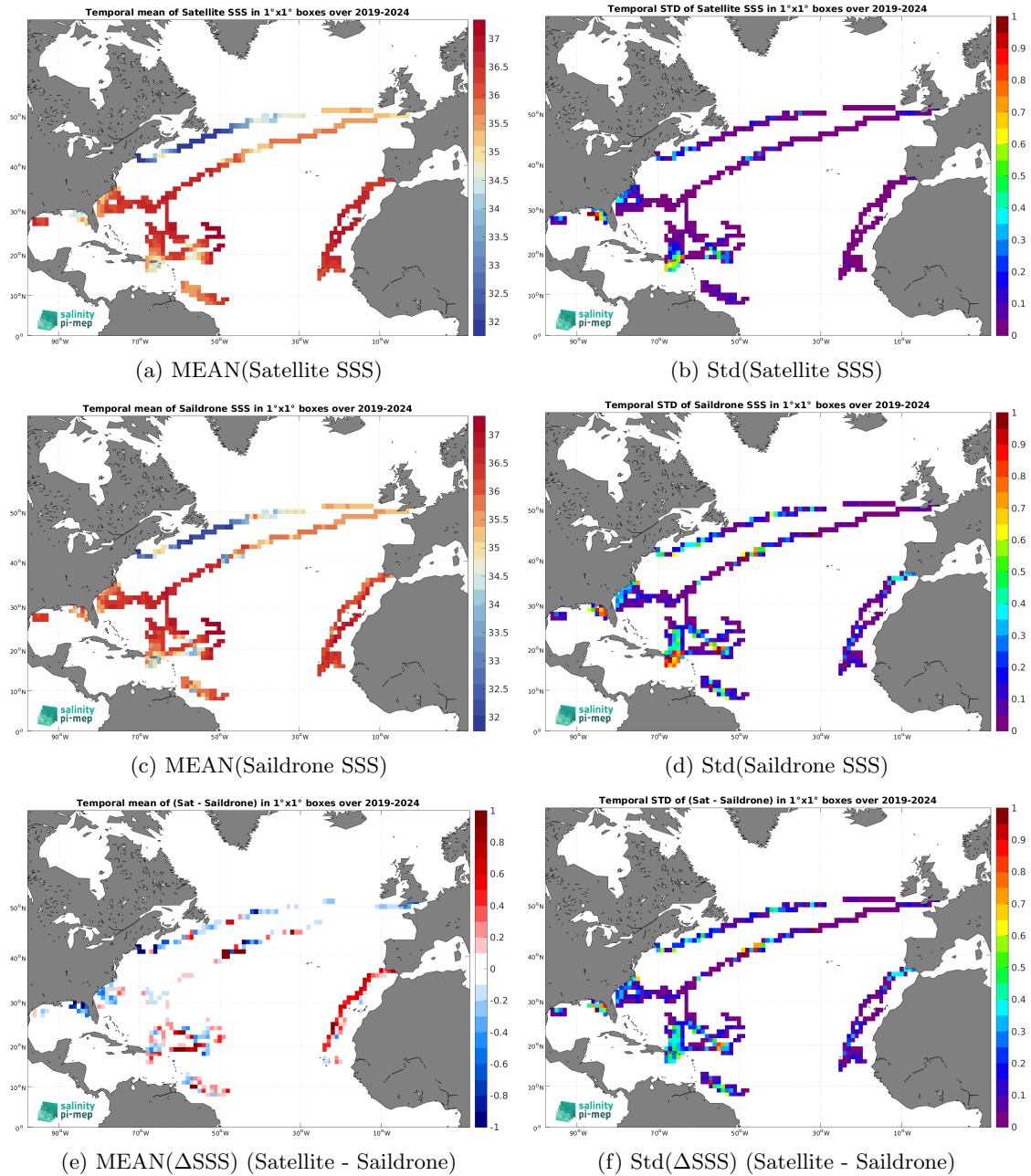
Figure 7: Temporal mean (left) and Std (right) of SSS from SMOS SSS L4 v1 - Monthly (CMEMS-CNR) (top), Saildrone (middle), and of \Delta SSS (Satellite - Saildrone). Only match-pairs are used to generate these maps.
