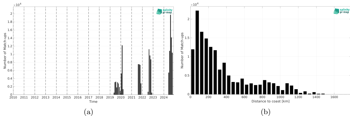
Figure 2: Number of match-ups between Saildrone and SMOS SSS L4 v1 - Monthly (CMEMS-CNR) SSS as a function of time (a) and as function of the distance to coast (b) over the North Atlantic Ocean Pi-MEP region and for the full satellite product period.
