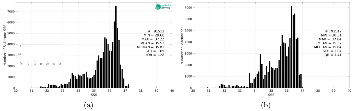
Figure 3: Histograms of SSS from Saildrone (a) and SMOS SSS L4 v1 - Monthly (CMEMS-CNR) (b) considering all match-up pairs per bins of 0.1 over the North Atlantic Ocean Pi-MEP region and for the full satellite product period.
