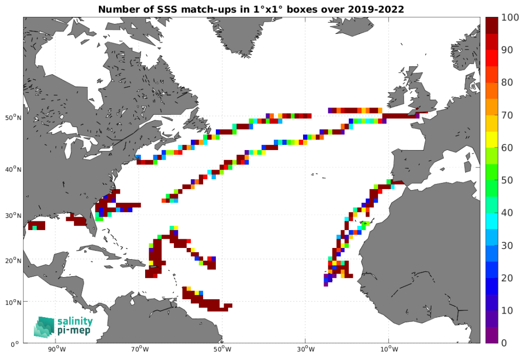
Figure 5: Number of SSS match-ups between Saildrone SSS and the SMOS SSS L4 v1 - Monthly (CMEMS-CNR) SSS product for the North Atlantic Ocean Pi-MEP region over 1^\circ \times 1^\circ boxes and for the full satellite product period.
