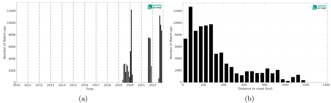
Figure 2: Number of match-ups between Saildrone and SMOS SSS L4 v1 - Monthly (CMEMS-CNR) SSS as a function of time (a) and as function of the distance to coast (b) over the North Atlantic Ocean Pi-MEP region and for the full satellite product period.
