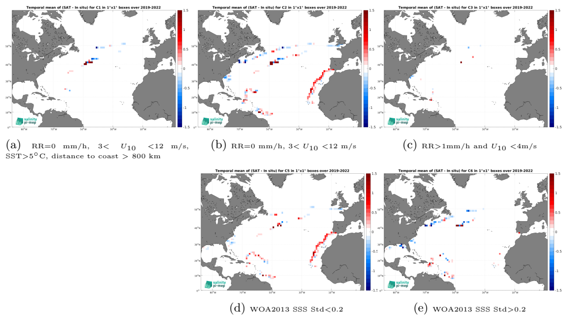
Figure 14: Temporal mean gridded over spatial boxes of size 1^\circ \times 1^\circ of \Delta\text{SSS} (SMOS SSS L4 v1 - Monthly (CMEMS-CNR) - Saildrone) for 5 different subdatasets corresponding to:RR=0 mm/h, 3 < U_{10} < 12 m/s, SST >5^\circ\text{C} , distance to coast > 800 km (a), RR=0 mm/h, 3 < U_{10} < 12 m/s (b), RR >1 mm/h and U_{10} < 4 m/s (c), WOA2013 SSS Std <0.2 (d), WOA2013 SSS Std >0.2 (e).
