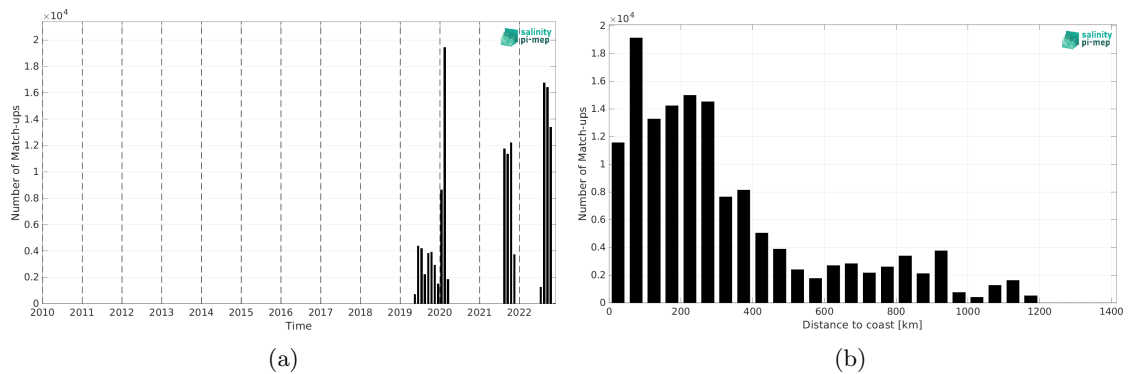
Figure 1: Number of match-ups between Saildrone and SMOS SSS L4 v1 - Monthly (CMEMS-CNR) SSS as a function of time (a) and as function of the distance to coast (b) over the North Atlantic Ocean Pi-MEP region and for the full satellite product period.
