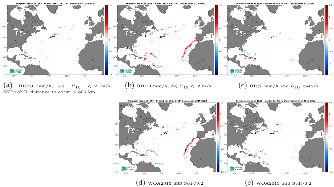
Figure 12: Temporal mean gridded over spatial boxes of size 1^\circ \times 1^\circ of \Delta\text{SSS} (SMOS SSS L4 v1 - Monthly (CMEMS-CNR) - Saildrone) for 5 different subdatasets corresponding to:RR=0 mm/h, 3 < U_{10} < 12 m/s, SST >5^\circ\text{C} , distance to coast > 800 km (a), RR=0 mm/h, 3 < U_{10} < 12 m/s (b), RR >1 mm/h and U_{10} < 4 m/s (c), WOA2013 SSS Std <0.2 (d), WOA2013 SSS Std >0.2 (e).
