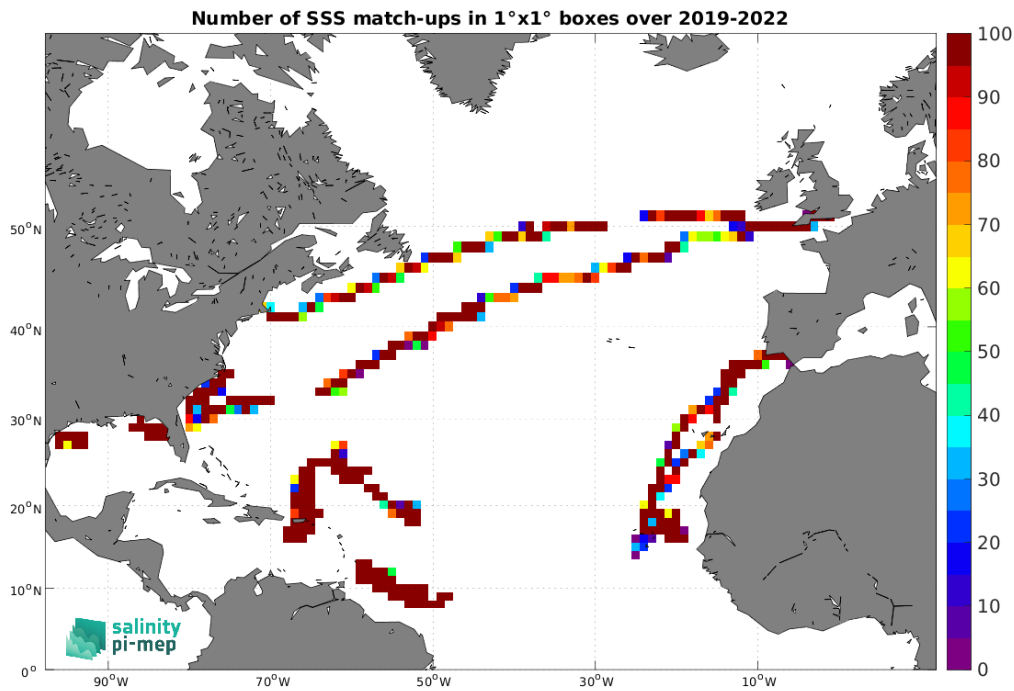
Figure 4: Number of SSS match-ups between Saildrone SSS and the SMOS SSS L4 v1 - Monthly (CMEMS-CNR) SSS product for the North Atlantic Ocean Pi-MEP region over 1^\circ \times 1^\circ boxes and for the full satellite product period.
