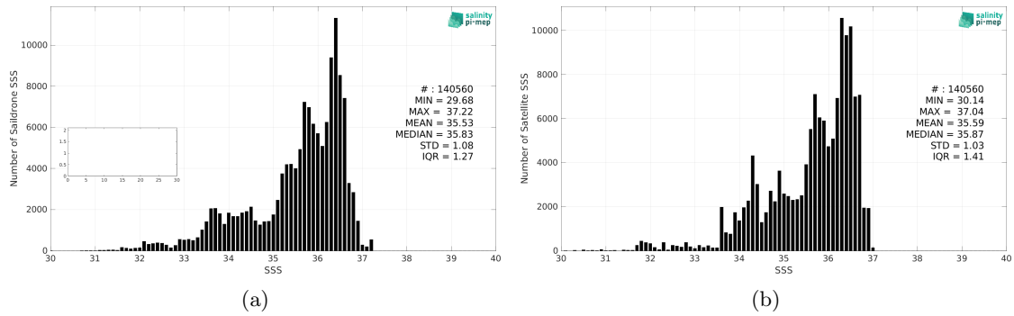
Figure 2: Histograms of SSS from Saildrone (a) and SMOS SSS L4 v1 - Monthly (CMEMS-CNR) (b) considering all match-up pairs per bins of 0.1 over the North Atlantic Ocean Pi-MEP region and for the full satellite product period.
