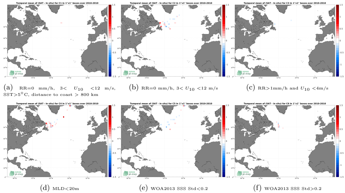
Figure 12: Temporal mean gridded over spatial boxes of size 1^{\circ}\times 1^{\circ} of \Delta\text{SSS} (SMOS SSS L4 v1 - Monthly (CMEMS-CNR) - Marine mammals) for 6 different subdatasets corresponding to:RR=0 mm/h, 3 < U_{10} < 12 m/s, SST >5^{\circ}\text{C} , distance to coast > 800 km (a), RR=0 mm/h, 3 < U_{10} < 12 m/s (b), RR >1 mm/h and U_{10} < 4 m/s (c),MLD <20 m (d),WOA2013 SSS Std <0.2 (e),WOA2013 SSS Std >0.2 (f).
