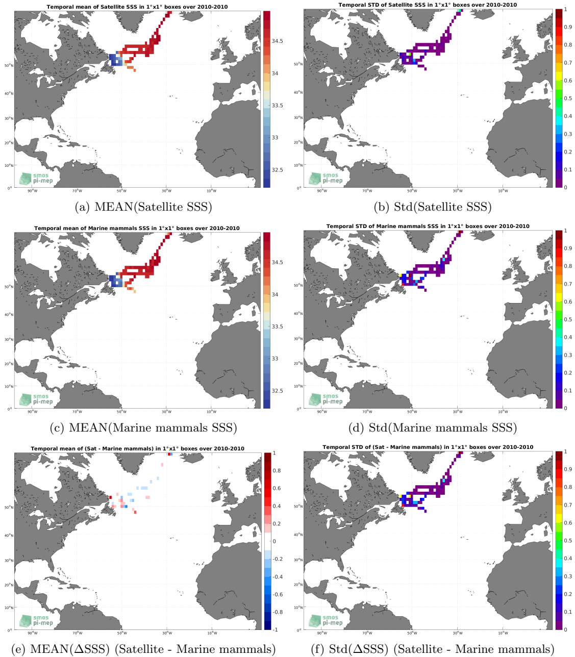
Figure 6: Temporal mean (left) and Std (right) of SSS from SMOS SSS L4 v1 - Monthly (CMEMS-CNR) (top), Marine mammals (middle), and of \Delta SSS (Satellite - Marine mammals). Only match-up pairs are used to generate these maps.
