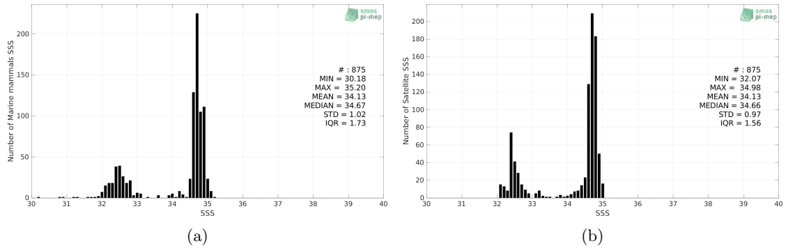
Figure 2: Histograms of SSS from Marine mammals (a) and SMOS SSS L4 v1 - Monthly (CMEMS-CNR) (b) considering all match-up pairs per bins of 0.1 over the North Atlantic Ocean Pi-MEP region and for the full satellite product period.
