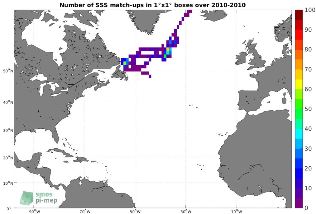
Figure 4: Number of SSS match-ups between Marine mammals SSS and the SMOS SSS L4 v1 - Monthly (CMEMS-CNR) SSS product for the North Atlantic Ocean Pi-MEP region over 1^\circ \times 1^\circ boxes and for the full satellite product period.
