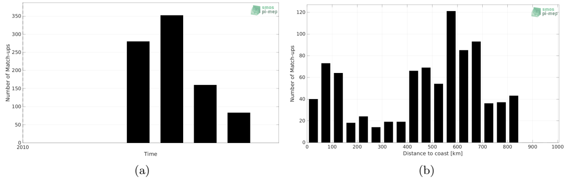
Figure 1: Number of match-ups between Marine mammals and SMOS SSS L4 v1 - Monthly (CMEMS-CNR) SSS as a function of time (a) and as function of the distance to coast (b) over the North Atlantic Ocean Pi-MEP region and for the full satellite product period.
