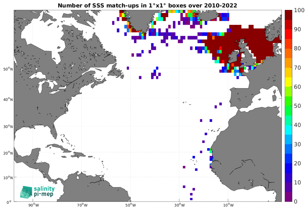
Figure 5: Number of SSS match-ups between ICES SSS and the SMOS SSS L4 v1 - Monthly (CMEMS-CNR) SSS product for the North Atlantic Ocean Pi-MEP region over 1^\circ \times 1^\circ boxes and for the full satellite product period.
