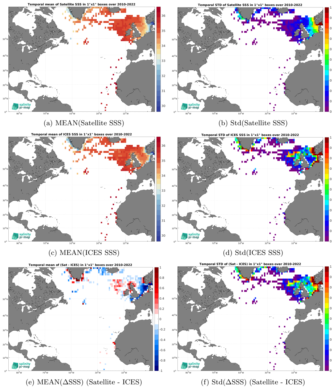
Figure 7: Temporal mean (left) and Std (right) of SSS from SMOS SSS L4 v1 - Monthly (CMEMS-CNR) (top), ICES (middle), and of \Delta SSS (Satellite - ICES). Only match-up pairs are used to generate these maps.
