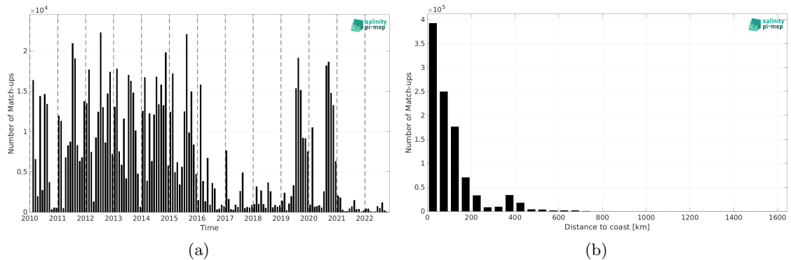
Figure 2: Number of match-ups between ICES and SMOS SSS L4 v1 - Monthly (CMEMS-CNR) SSS as a function of time (a) and as function of the distance to coast (b) over the North Atlantic Ocean Pi-MEP region and for the full satellite product period.
