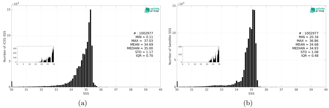
Figure 3: Histograms of SSS from ICES (a) and SMOS SSS L4 v1 - Monthly (CMEMS-CNR) (b) considering all match-up pairs per bins of 0.1 over the North Atlantic Ocean Pi-MEP region and for the full satellite product period.
