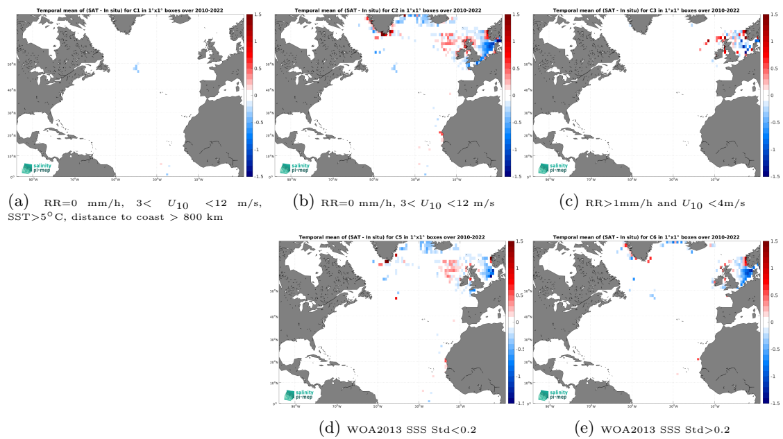
Figure 14: Temporal mean gridded over spatial boxes of size 1^\circ \times 1^\circ of \Delta\text{SSS} (SMOS SSS L4 v1 - Monthly (CMEMS-CNR) - ICES) for 5 different subdatasets corresponding to:RR=0 mm/h, 3 < U_{10} < 12 m/s, SST > 5^\circ\text{C} , distance to coast > 800 km (a), RR=0 mm/h, 3 < U_{10} < 12 m/s (b), RR > 1 mm/h and U_{10} < 4 m/s (c), WOA2013 SSS Std < 0.2 (d), WOA2013 SSS Std > 0.2 (e).
