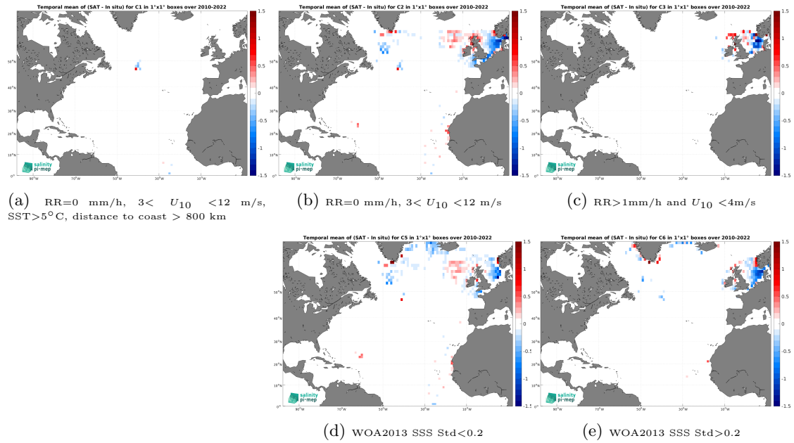
Figure 12: Temporal mean gridded over spatial boxes of size 1^\circ \times 1^\circ of \Delta\text{SSS} (SMOS SSS L4 v1 - Monthly (CMEMS-CNR) - ICES) for 5 different subdatasets corresponding to:RR=0 mm/h, 3 < U_{10} < 12 m/s, SST >5^\circ\text{C} , distance to coast > 800 km (a), RR=0 mm/h, 3 < U_{10} < 12 m/s (b), RR >1 mm/h and U_{10} < 4 m/s (c), WOA2013 SSS Std <0.2 (d), WOA2013 SSS Std >0.2 (e).
