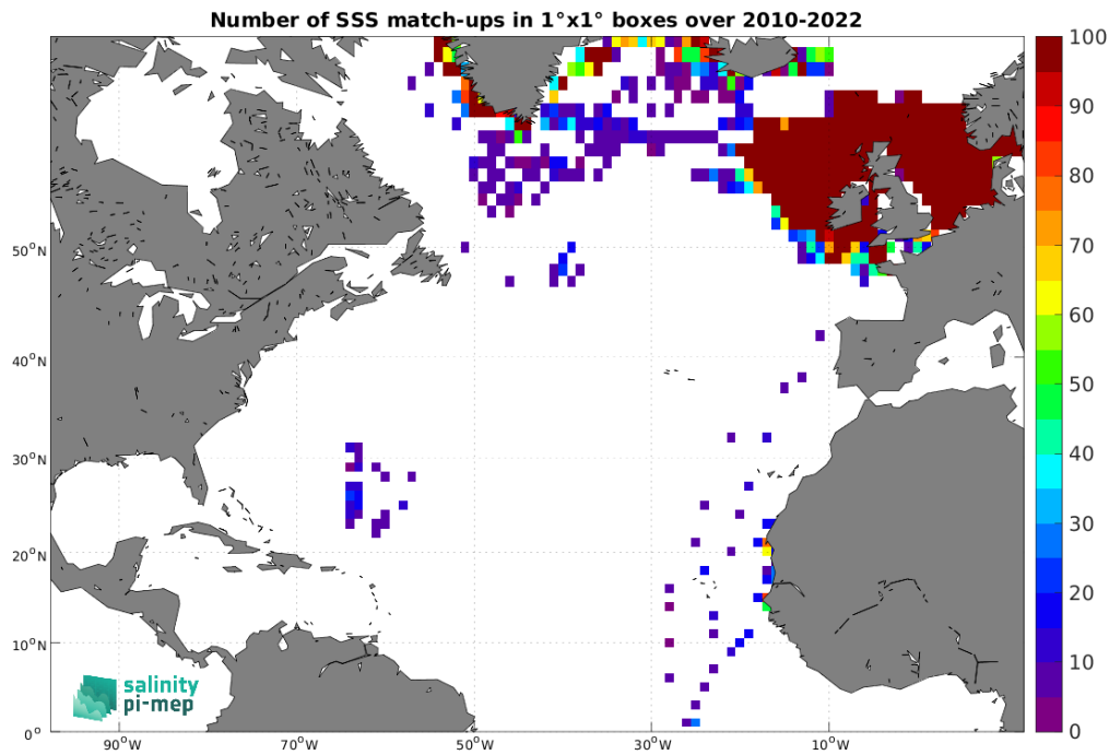
Figure 4: Number of SSS match-ups between ICES SSS and the SMOS SSS L4 v1 - Monthly (CMEMS-CNR) SSS product for the North Atlantic Ocean Pi-MEP region over 1^\circ \times 1^\circ boxes and for the full satellite product period.
