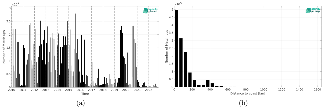
Figure 1: Number of match-ups between ICES and SMOS SSS L4 v1 - Monthly (CMEMS-CNR) SSS as a function of time (a) and as function of the distance to coast (b) over the North Atlantic Ocean Pi-MEP region and for the full satellite product period.
