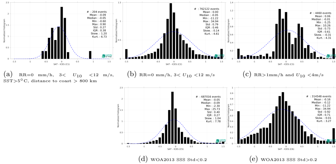
Figure 13: Normalized histogram of \Delta SSS (SMOS SSS L4 v1 - Monthly (CMEMS-CNR) - ICES) for 5 different subdatasets corresponding to: RR=0 mm/h, 3 < U_{10} < 12 m/s, SST>5°C, distance to coast > 800 km (a), RR=0 mm/h, 3 < U_{10} < 12 m/s (b), RR>1mm/h and U_{10} < 4 m/s (c), WOA2013 SSS Std<0.2 (d), WOA2013 SSS Std>0.2 (e).
