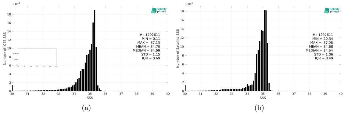
Figure 2: Histograms of SSS from ICES (a) and SMOS SSS L4 v1 - Monthly (CMEMS-CNR) (b) considering all match-up pairs per bins of 0.1 over the North Atlantic Ocean Pi-MEP region and for the full satellite product period.
