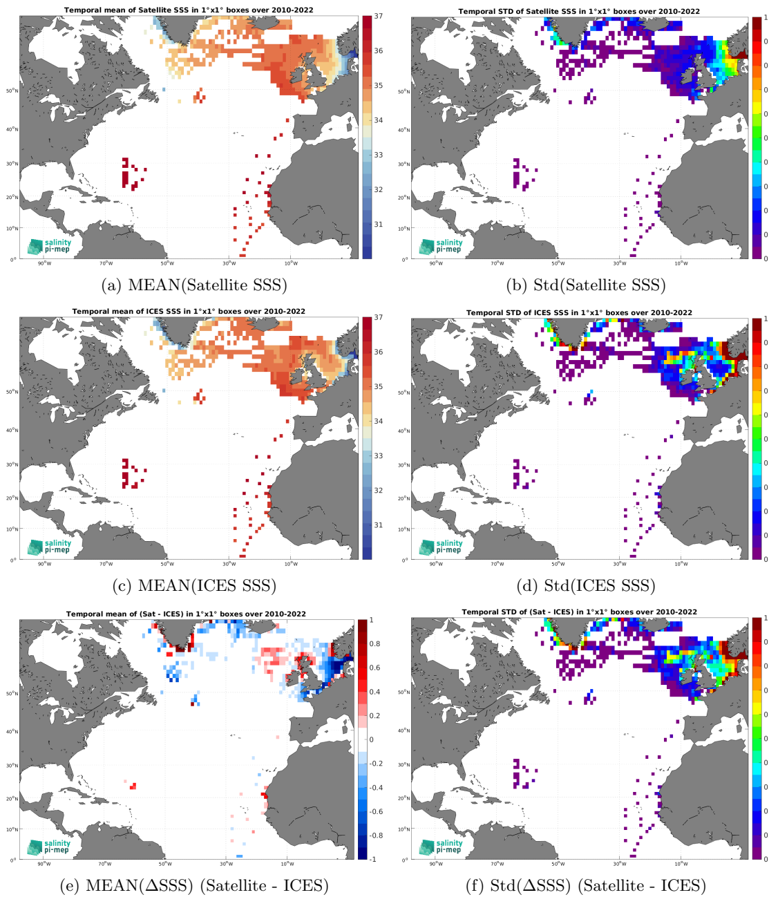
Figure 6: Temporal mean (left) and Std (right) of SSS from SMOS SSS L4 v1 - Monthly (CMEMS-CNR) (top), ICES (middle), and of \Delta SSS (Satellite - ICES). Only match-up pairs are used to generate these maps.
