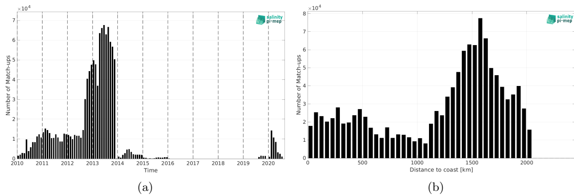
Figure 1: Number of match-ups between Surface drifters and SMOS SSS L4 v1 - Monthly (CMEMS-CNR) SSS as a function of time (a) and as function of the distance to coast (b) over the North Atlantic Ocean Pi-MEP region and for the full satellite product period.
