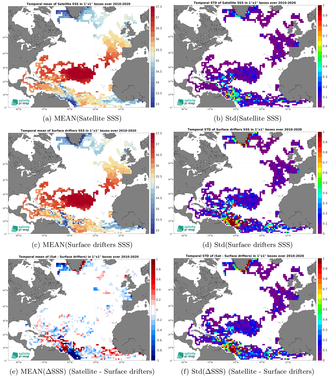
Figure 5: Temporal mean (left) and Std (right) of SSS from SMOS SSS L4 v1 - Monthly (CMEMS-CNR) (top), Surface drifters (middle), and of \Delta SSS (Satellite - Surface drifters). Only match-up pairs are used to generate these maps.
