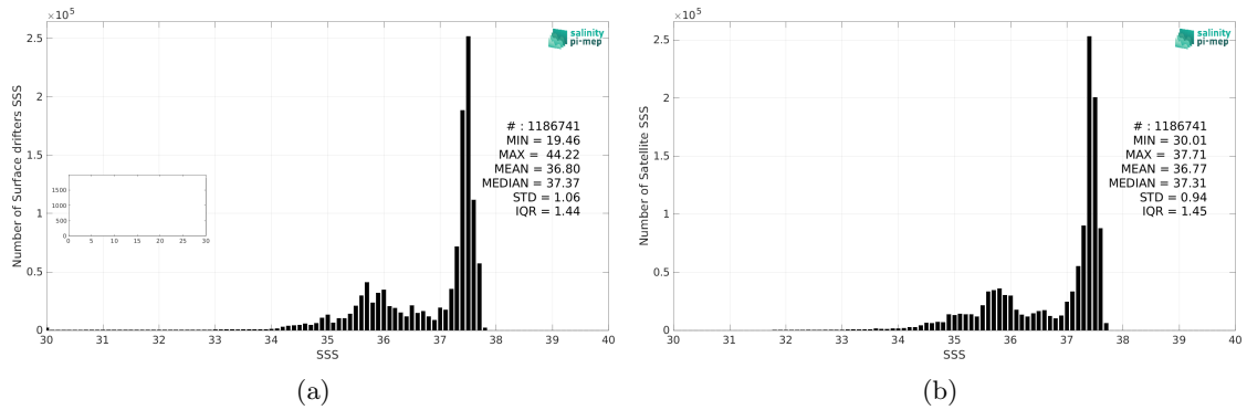
Figure 2: Histograms of SSS from Surface drifters (a) and SMOS SSS L4 v1 - Monthly (CMEMS-CNR) (b) considering all match-up pairs per bins of 0.1 over the North Atlantic Ocean Pi-MEP region and for the full satellite product period.
