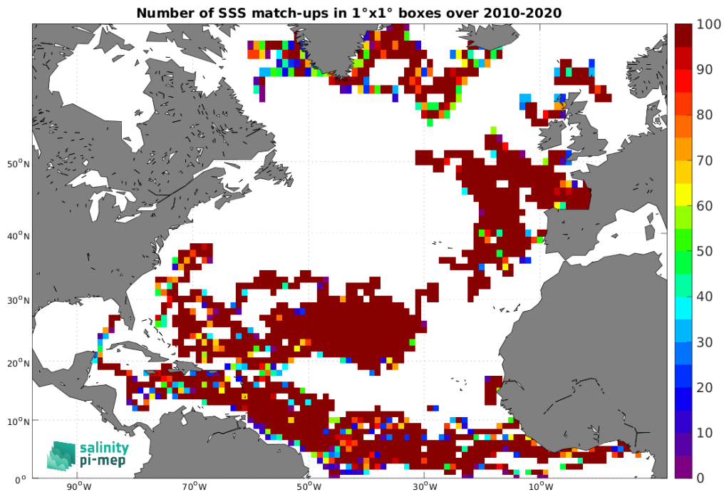
Figure 3: Number of SSS match-ups between Surface drifters SSS and the SMOS SSS L4 v1 - Monthly (CMEMS-CNR) SSS product for the North Atlantic Ocean Pi-MEP region over 1^\circ \times 1^\circ boxes and for the full satellite product period.
