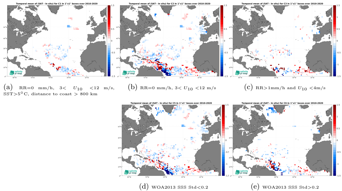
Figure 11: Temporal mean gridded over spatial boxes of size 1^\circ \times 1^\circ of \Delta\text{SSS} (SMOS SSS L4 v1 - Monthly (CMEMS-CNR) - Surface drifters) for 5 different subdatasets corresponding to:RR=0 mm/h, 3 < U_{10} < 12 m/s, SST > 5^\circ\text{C} , distance to coast > 800 km (a), RR=0 mm/h, 3 < U_{10} < 12 m/s (b), RR > 1 mm/h and U_{10} < 4 m/s (c), WOA2013 SSS Std < 0.2 (d), WOA2013 SSS Std > 0.2 (e).
