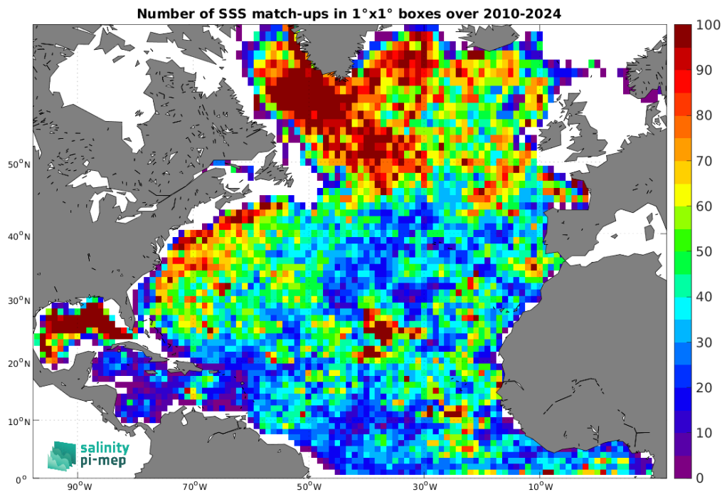
Figure 5: Number of SSS match-ups between Argo SSS and the SMOS SSS L4 v1 - Monthly (CMEMS-CNR) SSS product for the North Atlantic Ocean Pi-MEP region over 1^\circ \times 1^\circ boxes and for the full satellite product period.
