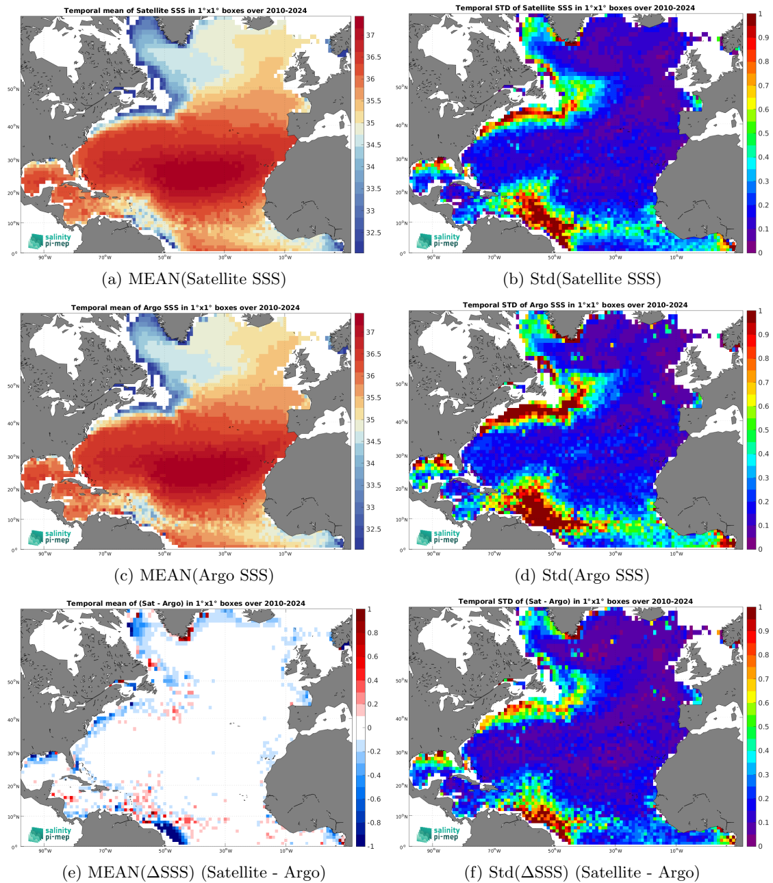
Figure 7: Temporal mean (left) and Std (right) of SSS from SMOS SSS L4 v1 - Monthly (CMEMS-CNR) (top), Argo (middle), and of \Delta SSS (Satellite - Argo). Only match-up pairs are used to generate these maps.
