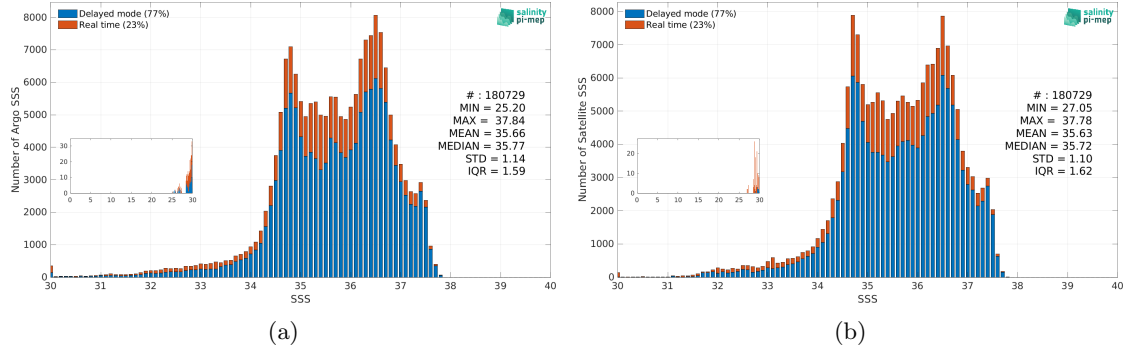
Figure 3: Histograms of SSS from Argo (a) and SMOS SSS L4 v1 - Monthly (CMEMS-CNR) (b) considering all match-up pairs per bins of 0.1 over the North Atlantic Ocean Pi-MEP region and for the full satellite product period.
