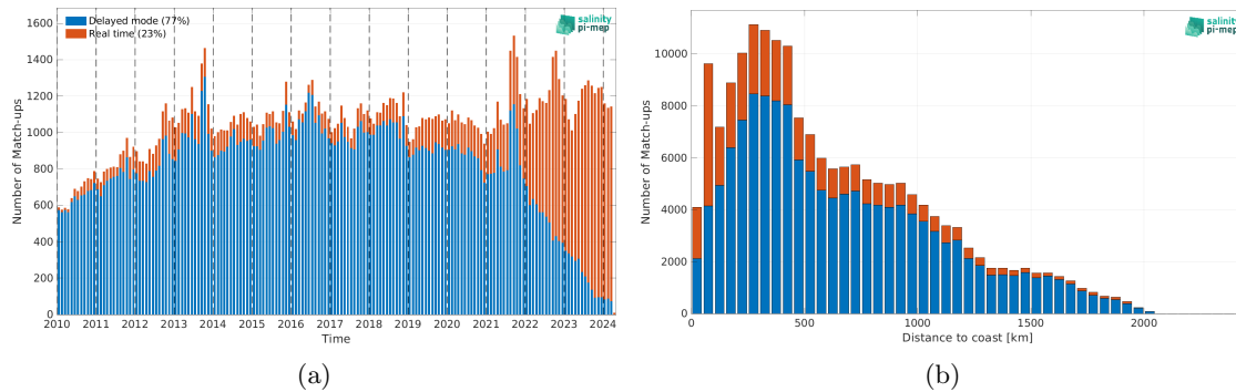
Figure 2: Number of match-ups between Argo and SMOS SSS L4 v1 - Monthly (CMEMS-CNR) SSS as a function of time (a) and as function of the distance to coast (b) over the North Atlantic Ocean Pi-MEP region and for the full satellite product period.
