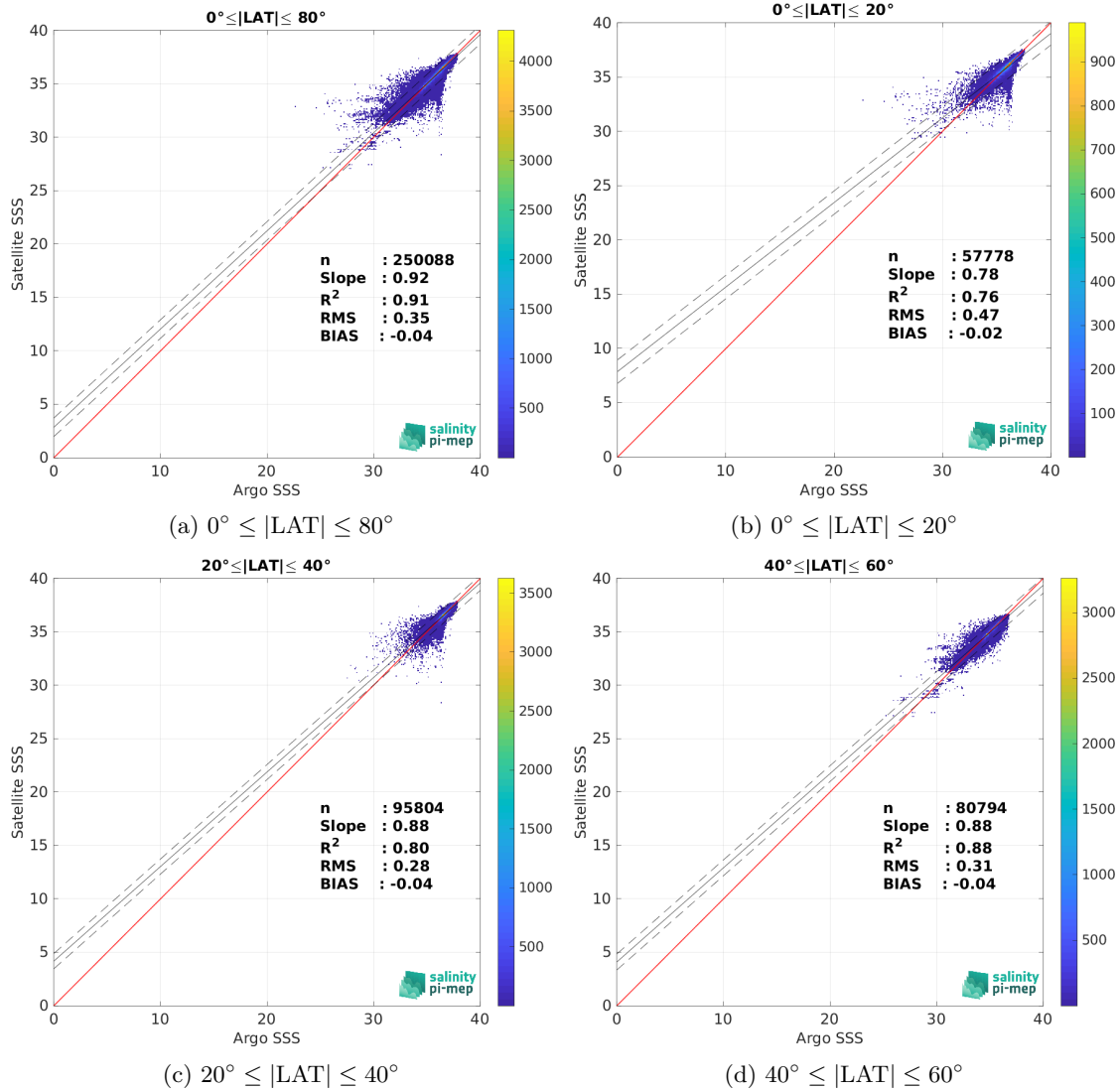
Figure 9: Contour maps of the concentration of SMOS SSS L4 v1 - Monthly (CMEMS-CNR) SSS (y-axis) versus Argo SSS (x-axis) at match-up pairs for different latitude bands. For each plot, the red line shows x=y . The black thin and dashed lines indicate a linear fit through the data cloud and the \pm 95\% confidence levels, respectively. The number match-up pairs n , the slope and R^2 coefficient of the linear fit, the root mean square (RMS) and the mean bias between satellite and in situ data are indicated for each latitude band in each plots.
