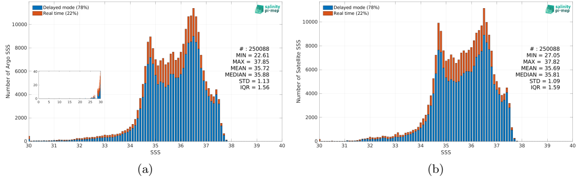
Figure 2: Histograms of SSS from Argo (a) and SMOS SSS L4 v1 - Monthly (CMEMS-CNR) (b) considering all match-up pairs per bins of 0.1 over the North Atlantic Ocean Pi-MEP region and for the full satellite product period.
