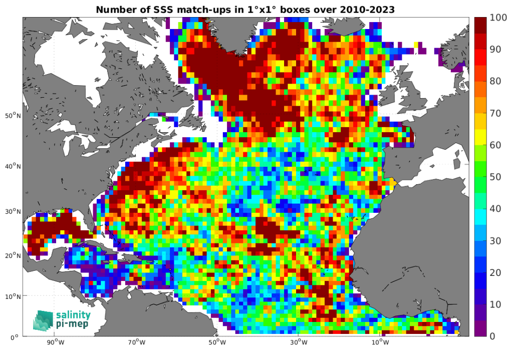
Figure 4: Number of SSS match-ups between Argo SSS and the SMOS SSS L4 v1 - Monthly (CMEMS-CNR) SSS product for the North Atlantic Ocean Pi-MEP region over 1^\circ \times 1^\circ boxes and for the full satellite product period.
