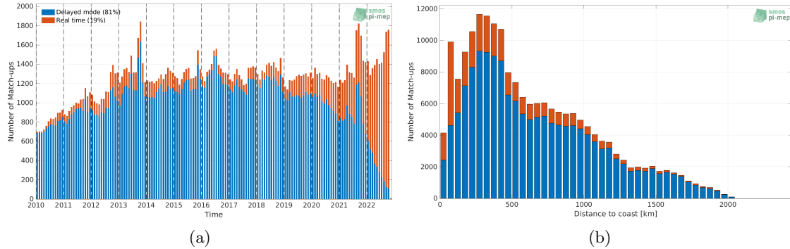
Figure 1: Number of match-ups between Argo and SMOS SSS L4 v1 - Monthly (CMEMS-CNR) SSS as a function of time (a) and as function of the distance to coast (b) over the North Atlantic Ocean Pi-MEP region and for the full satellite product period.
