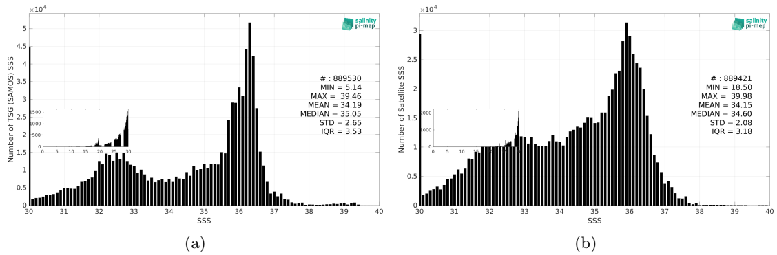
Figure 3: Histograms of SSS from TSG (SAMOS) (a) and SMOS SSS L4 v1 - Daily (CMEMS-CNR) (b) considering all match-up pairs per bins of 0.1 over the North Atlantic Ocean Pi-MEP region and for the full satellite product period.
