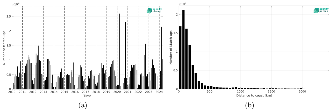
Figure 2: Number of match-ups between TSG (SAMOS) and SMOS SSS L4 v1 - Daily (CMEMS-CNR) SSS as a function of time (a) and as function of the distance to coast (b) over the North Atlantic Ocean Pi-MEP region and for the full satellite product period.
