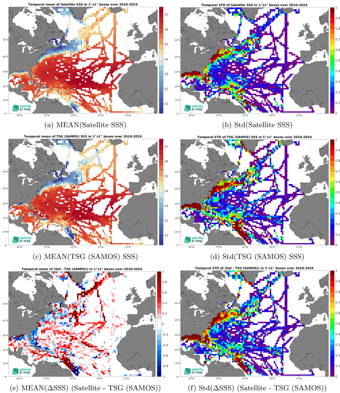
Figure 7: Temporal mean (left) and Std (right) of SSS from SMOS SSS L4 v1 - Daily (CMEMS-CNR) (top), TSG (SAMOS) (middle), and of \Delta SSS (Satellite - TSG (SAMOS)). Only match-up pairs are used to generate these maps.
