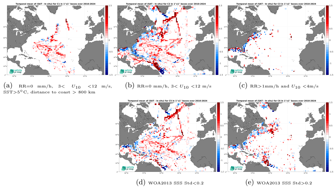
Figure 14: Temporal mean gridded over spatial boxes of size 1^\circ \times 1^\circ of \Delta SSS (SMOS SSS L4 v1 - Daily (CMEMS-CNR) - TSG (SAMOS)) for 5 different subdatasets corresponding to:RR=0 mm/h, 3 < U_{10} < 12 m/s, SST >5^\circ\text{C} , distance to coast > 800 km (a), RR=0 mm/h, 3 < U_{10} < 12 m/s (b), RR >1 mm/h and U_{10} < 4 m/s (c), WOA2013 SSS Std <0.2 (d), WOA2013 SSS Std >0.2 (e).
