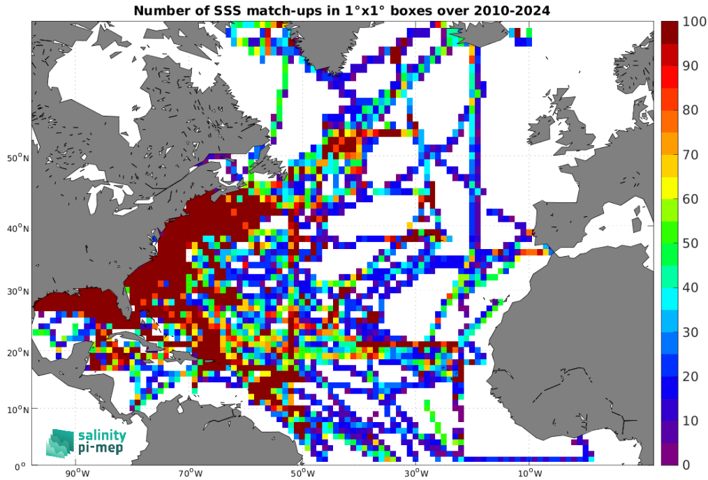
Figure 5: Number of SSS match-ups between TSG (SAMOS) SSS and the SMOS SSS L4 v1 - Daily (CMEMS-CNR) SSS product for the North Atlantic Ocean Pi-MEP region over 1^\circ \times 1^\circ boxes and for the full satellite product period.
