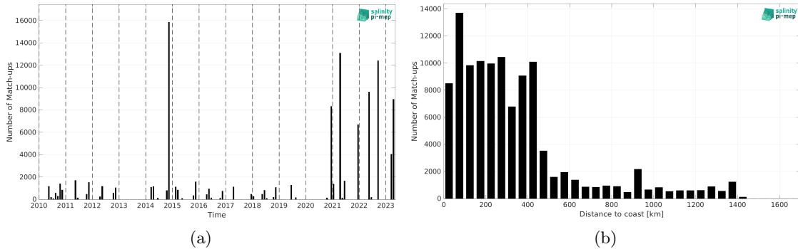
Figure 2: Number of match-ups between TSG (Polarstern) and SMOS SSS L4 v1 - Daily (CMEMS-CNR) SSS as a function of time (a) and as function of the distance to coast (b) over the North Atlantic Ocean Pi-MEP region and for the full satellite product period.
