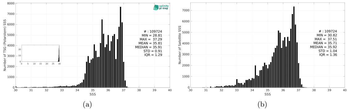
Figure 3: Histograms of SSS from TSG (Polarstern) (a) and SMOS SSS L4 v1 - Daily (CMEMS-CNR) (b) considering all match-up pairs per bins of 0.1 over the North Atlantic Ocean Pi-MEP region and for the full satellite product period.
