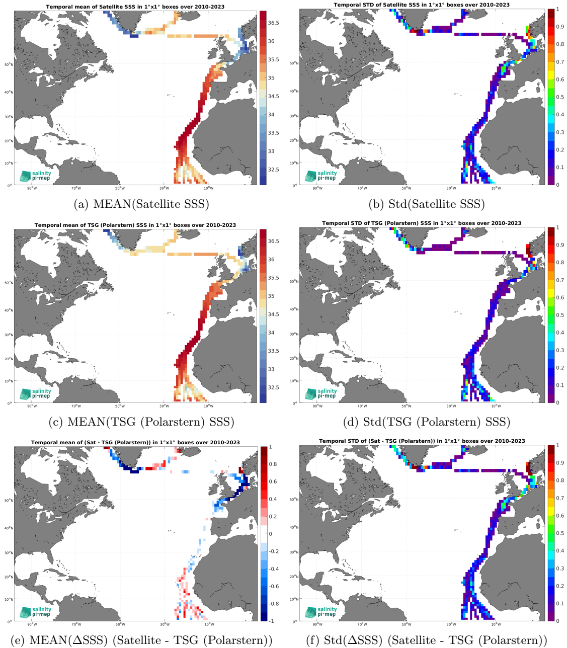
Figure 7: Temporal mean (left) and Std (right) of SSS from SMOS SSS L4 v1 - Daily (CMEMS-CNR) (top), TSG (Polarstern) (middle), and of \Delta SSS (Satellite - TSG (Polarstern)). Only match-up pairs are used to generate these maps.
