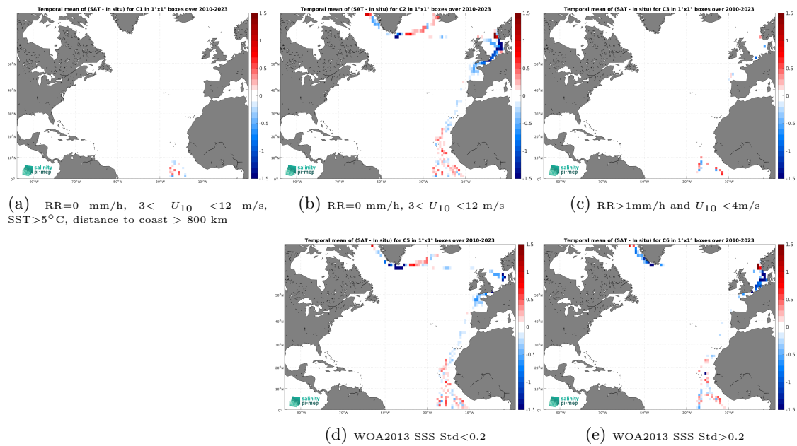
Figure 14: Temporal mean gridded over spatial boxes of size 1^\circ \times 1^\circ of \Delta\text{SSS} (SMOS SSS L4 v1 - Daily (CMEMS-CNR) - TSG (Polarstern)) for 5 different subdatasets corresponding to:RR=0 mm/h, 3 < U_{10} < 12 m/s, SST >5^\circ\text{C} , distance to coast > 800 km (a), RR=0 mm/h, 3 < U_{10} < 12 m/s (b), RR >1 mm/h and U_{10} < 4 m/s (c), WOA2013 SSS Std <0.2 (d), WOA2013 SSS Std >0.2 (e).
