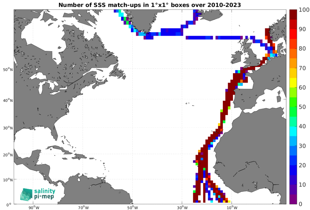
Figure 5: Number of SSS match-ups between TSG (Polarstern) SSS and the SMOS SSS L4 v1 - Daily (CMEMS-CNR) SSS product for the North Atlantic Ocean Pi-MEP region over 1^\circ \times 1^\circ boxes and for the full satellite product period.
