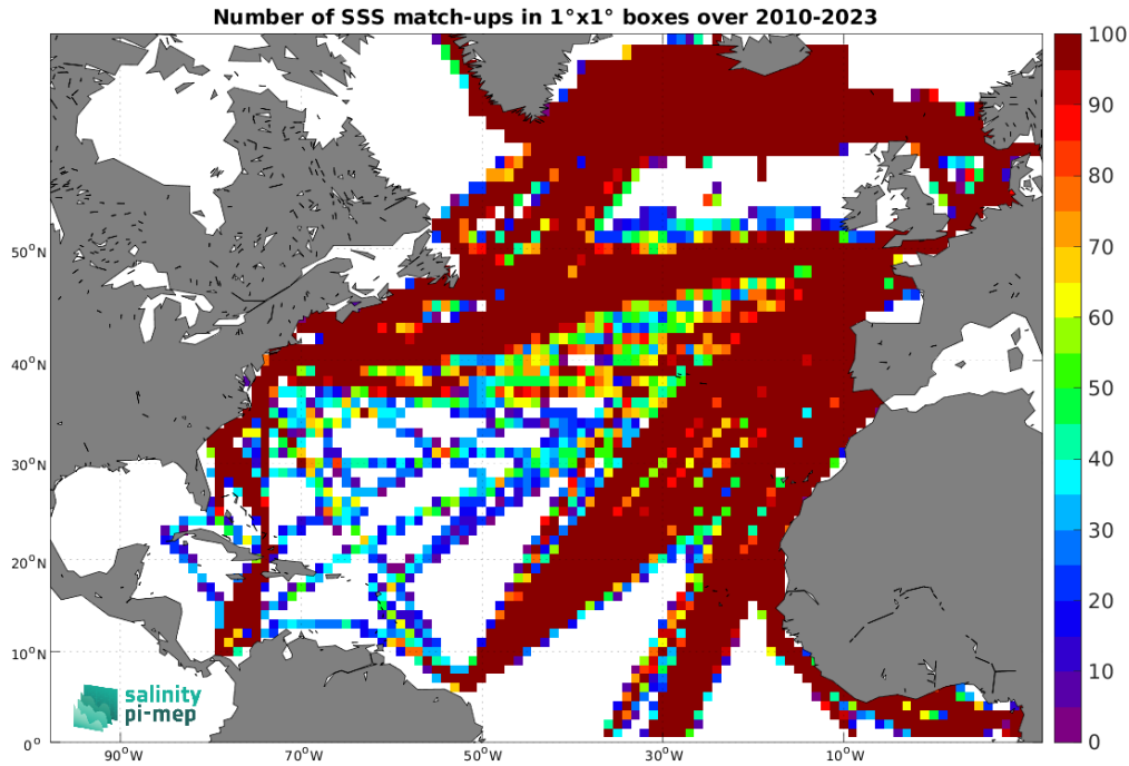
Figure 5: Number of SSS match-ups between TSG (LEGOS-DM) SSS and the SMOS SSS L4 v1 - Daily (CMEMS-CNR) SSS product for the North Atlantic Ocean Pi-MEP region over 1^\circ \times 1^\circ boxes and for the full satellite product period.
