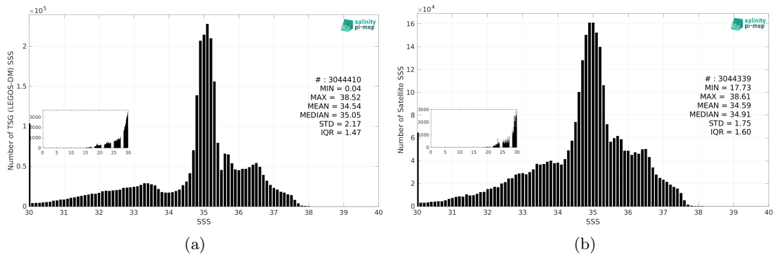
Figure 3: Histograms of SSS from TSG (LEGOS-DM) (a) and SMOS SSS L4 v1 - Daily (CMEMS-CNR) (b) considering all match-up pairs per bins of 0.1 over the North Atlantic Ocean Pi-MEP region and for the full satellite product period.
