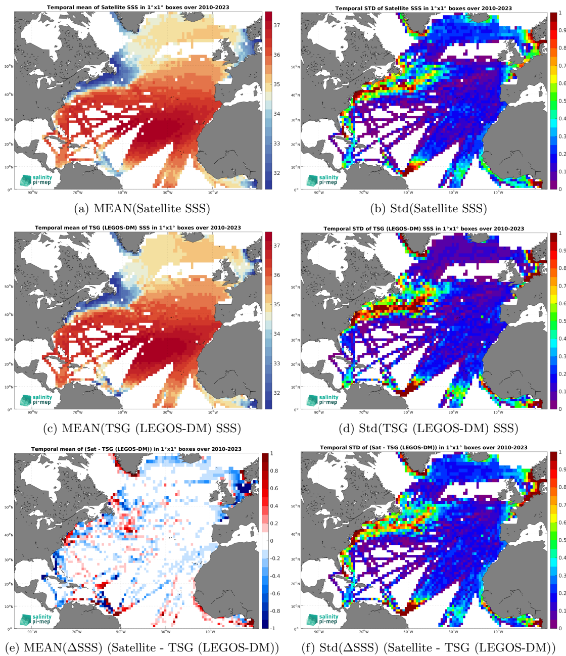
Figure 7: Temporal mean (left) and Std (right) of SSS from SMOS SSS L4 v1 - Daily (CMEMS-CNR) (top), TSG (LEGOS-DM) (middle), and of \Delta SSS (Satellite - TSG (LEGOS-DM)). Only match-up pairs are used to generate these maps.
