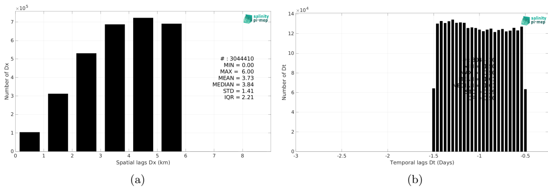
Figure 6: Histograms of the spatial (a) and temporal (b) lags between the location/time of the TSG (LEGOS-DM) measurement and the date of the corresponding SMOS SSS L4 v1 - Daily (CMEMS-CNR) SSS pixel.
