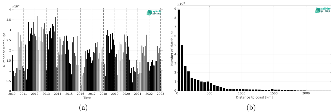
Figure 2: Number of match-ups between TSG (LEGOS-DM) and SMOS SSS L4 v1 - Daily (CMEMS-CNR) SSS as a function of time (a) and as function of the distance to coast (b) over the North Atlantic Ocean Pi-MEP region and for the full satellite product period.
