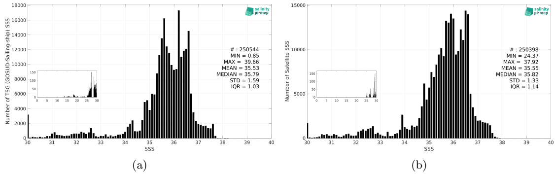
Figure 3: Histograms of SSS from TSG (GOSUD-Sailing-ship) (a) and SMOS SSS L4 v1 - Daily (CMEMS-CNR) (b) considering all match-up pairs per bins of 0.1 over the North Atlantic Ocean Pi-MEP region and for the full satellite product period.
