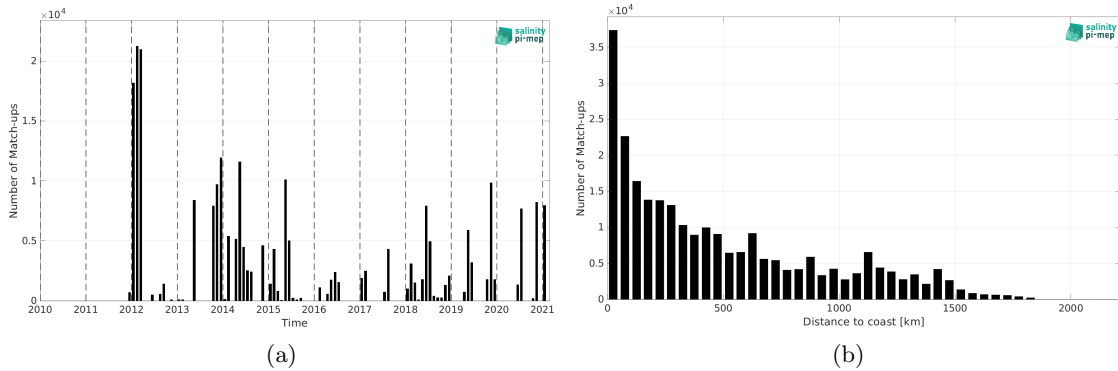
Figure 2: Number of match-ups between TSG (GOSUD-Sailing-ship) and SMOS SSS L4 v1 - Daily (CMEMS-CNR) SSS as a function of time (a) and as function of the distance to coast (b) over the North Atlantic Ocean Pi-MEP region and for the full satellite product period.
